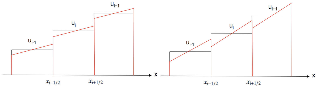
Figure 4.3: Illustration of the minmod (left) and mocnen (right) slope limiters applied to a piecewise constant function. Slope limiter minmod ensures that \mathbb{U}_{i+1/2,L} \leq \mathbb{U}_{i+1/2,R} and mocnen ensures that \mathbb{U}_{i-1} \leq \mathbb{U}_{i+1/2,L} \leq \mathbb{U}_{i+1} . Taken from Romain Teyssier lecture.
