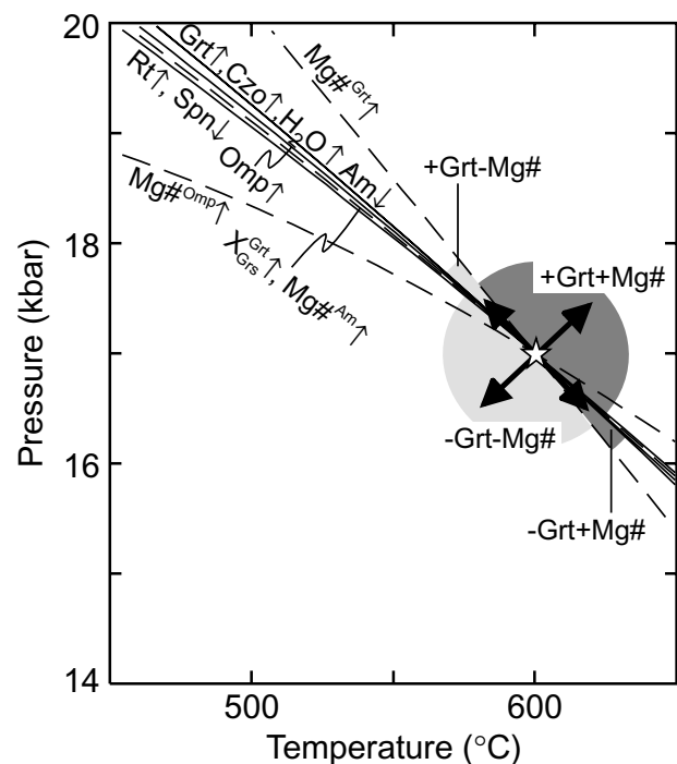
Fig. 11. Calculated phase relationships among garnet, omphacite, amphibole, clinozoisite, rutile, titanite and \text{H}_2\text{O} -fluid within the \text{SiO}_2 - \text{TiO}_2 - \text{Al}_2\text{O}_3 - \text{FeO} - \text{MgO} - \text{CaO} - \text{Na}_2\text{O} - \text{H}_2\text{O} system using program Gibbs (Spear & Menard, 1989; January 2000 thermodynamic data base). Clinozoisite, rutile, titanite and \text{H}_2\text{O} -fluid are pure phases, while garnet is treated as a Fe-Mg-Ca solution (3-site mixing model after Berman, 1990), omphacite as a diopside-hedenbergite-jadeite solution (2-site mixing model after Spear, unpublished), and amphibole an Fe-Mg solution (1-site-ideal mixing model, with the formula \text{Si}_6\text{Al}_{3.7}(\text{Fe},\text{Mg})_{3.3}\text{Ca}_2\text{Na}_{0.3}\text{O}_{22}(\text{OH})_2 , after Spear, unpublished). The starting conditions for the calculations (star) are as follows: P = 17 kbar; T = 600 °C, garnet = 29.5% volume ( X_{\text{alm}} = 0.55 , X_{\text{prp}} = 0.15 , X_{\text{grs}} = 0.30 , \text{Mg\#} = 0.79 ), omphacite = 45% ( X_{\text{dp}} = 0.5 , X_{\text{hd}} = 0.1 , X_{\text{jd}} = 0.4 , \text{Mg\#} = 0.17 ), amphibole = 20% ( \text{Mg\#} = 0.58 ), clinozoisite = 3%, rutile = 1.5%, titanite = 1%, and \text{H}_2\text{O} = 0\% . \text{H}_2\text{O} -fluid is allowed to fractionate (leave/enter the system) along the projected isopleths. The small arrows adjacent to the labels of the minerals (moles) and chemical variables indicate the direction of increasing contents. The shaded sectors indicate the P - T fields (relative to the star) where Mg# in growing/dissolving garnet decreases or increases.
