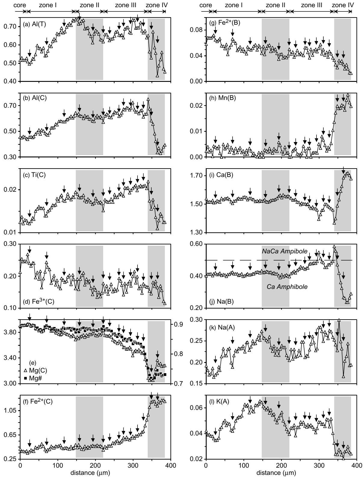
Fig. 6. Detailed core to rim profile (probe step: 4 μm) of amphibole porphyroblast shown in Fig. 5. Note that zoning includes large-range (zones I-IV) and short range oscillations (arrows define decrease in Al(C) and/or Al(T)).
