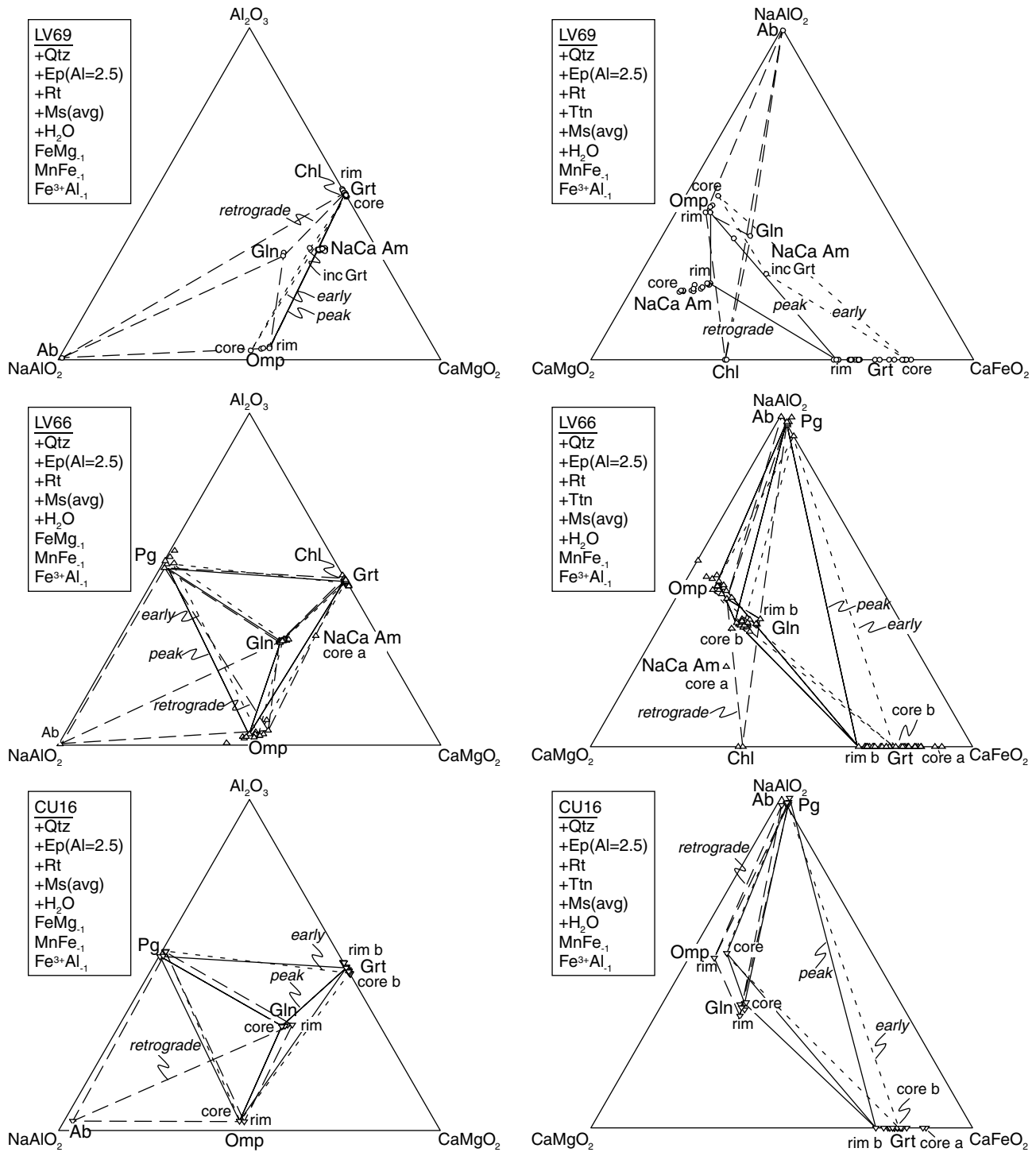
Fig. 6. Al_2O_3 - NaAlO_2 - CaMgO_2 (Schliestedt, 1990) and NaAlO_2 - CaFeO_2 - CaMgO_2 (García-Casco et al. , 2002) phase diagrams after projection of the composition of minerals from the molecular species indicated in the boxes. Small dashed line joins the pre-peak assemblage, plain line the eclogitic-peak assemblage and large dashed line the retrogressed assemblage. (avg): average.
