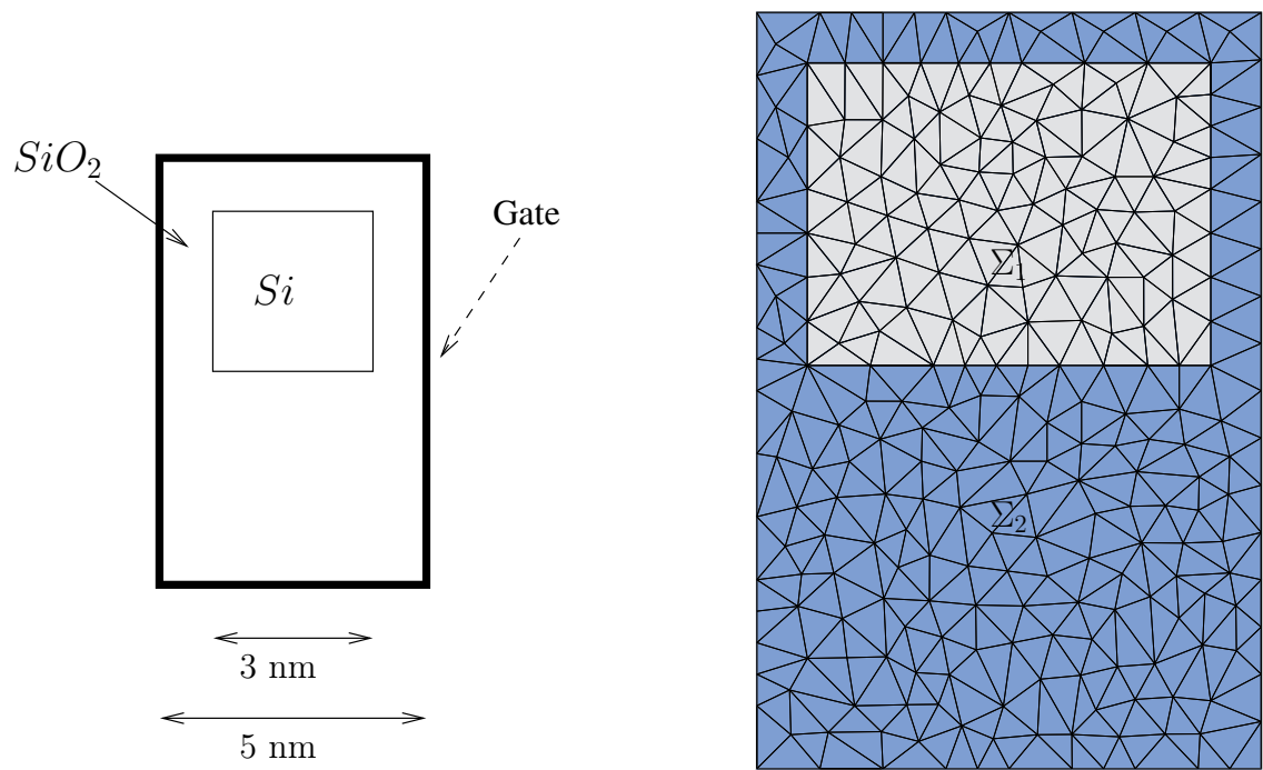
FIG. 6.1 – Section carrée
