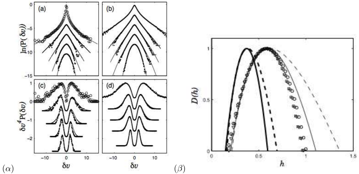
Figure 7: (α) (a)(c) Fit of the multifractal description on experimental data (circles: acceleration data from Cornell, dots: velocity increments from ultrasound Doppler, solid lines fits) – (b)(d) same for numerical simulations. See [11] for details. (β) Spectrum \mathcal{D}(h) extracted from the silicon strip acceleration data (triangles), ultrasound data (squares) and DNS data (circles). Thick lines are Eulerian spectra (lognormal: solid, log-Poisson: dashed) and thin lines are their Lagrangian counterparts. Figures from [11].
