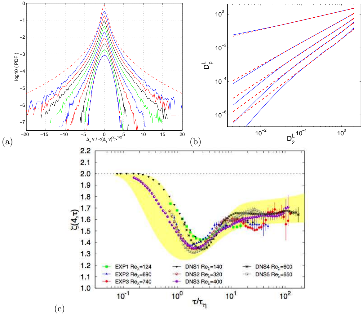
Figure 5: (a) Distributions of the velocity increments \Delta_\tau v . Solid lines: PDF of the increments for \tau = 0.15, 0.31, 0.61, 1.2, 2.5, 4.9, 9.8, 20 at 39 ms (from top to bottom). At R_\lambda \sim 800 , we measured T_L \approx 22 ms. Data from ultrasound Doppler. Top dashed line: PDF of the acceleration component measured by silicon strip detectors from [48]. Bottom dashed line: Gaussian distribution. Figure from [33]. (b) ESS plot of the structure functions S_p(\tau) (here noted D_p ) versus S_2(\tau) for p = 1, 3, 4, 5, 6 from top to bottom together with linear fits in dashed line. The estimated slopes are \zeta_p = 0.56, 1.34, 1.58, 1.76, 1.9 respectively. Figure from [39]. (c) Compilation of experimental and numerical values of the scale dependant fourth order scaling exponent \zeta(4, \tau) of S_4(\tau) . Our ultrasound Doppler data is EXP3. Details about other datasets are to be found in [2]. The yellow area is the prediction obtained starting from Eulerian measurement through a change of variable from length scale to time scale in a multifractal framework. Figure from [2].
