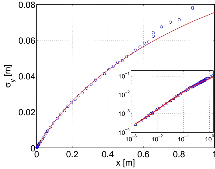
Figure 11: Width of the average temperature profiles as a function of the distance downstream the source. Circles are measurements, the solid line is the model prediction (11) with C_0 = 2.7 . Inset: same in loglog scale.
