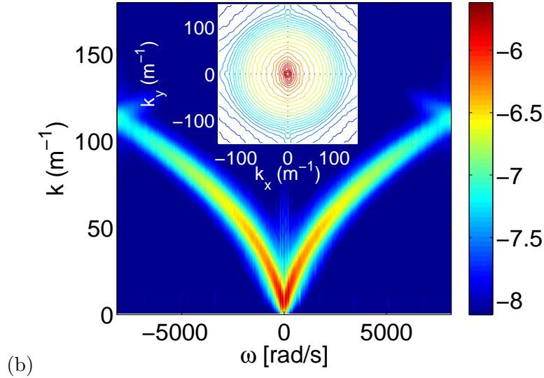
Figure 26: (a) Space-time spectrum E_v(\mathbf{k}, \omega) of the deformation velocity of the plate. Measurement by the FTP technique. Colors are log-scaled. (b) Space-time spectrum E_v(k, \omega) averaged over directions of \mathbf{k} . Colors are log-scaled. Inset: contours of the space spectrum E_v(\mathbf{k}) integrated over the frequencies (i.e. averaged in time). Figures from [15].
