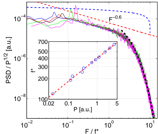
Figure 29: One point spectrum measured by Laser Doppler profilometry. Thin solid lines: measured spectra for various forcing amplitude. Red dashed line 1/F^{0.6} scaling. Blue dashed line, \ln(10f^*/F)^{1/3} . Black dashed line: exponential decay. Inset: measured f^* as a function of the input power. Figure from [34].
