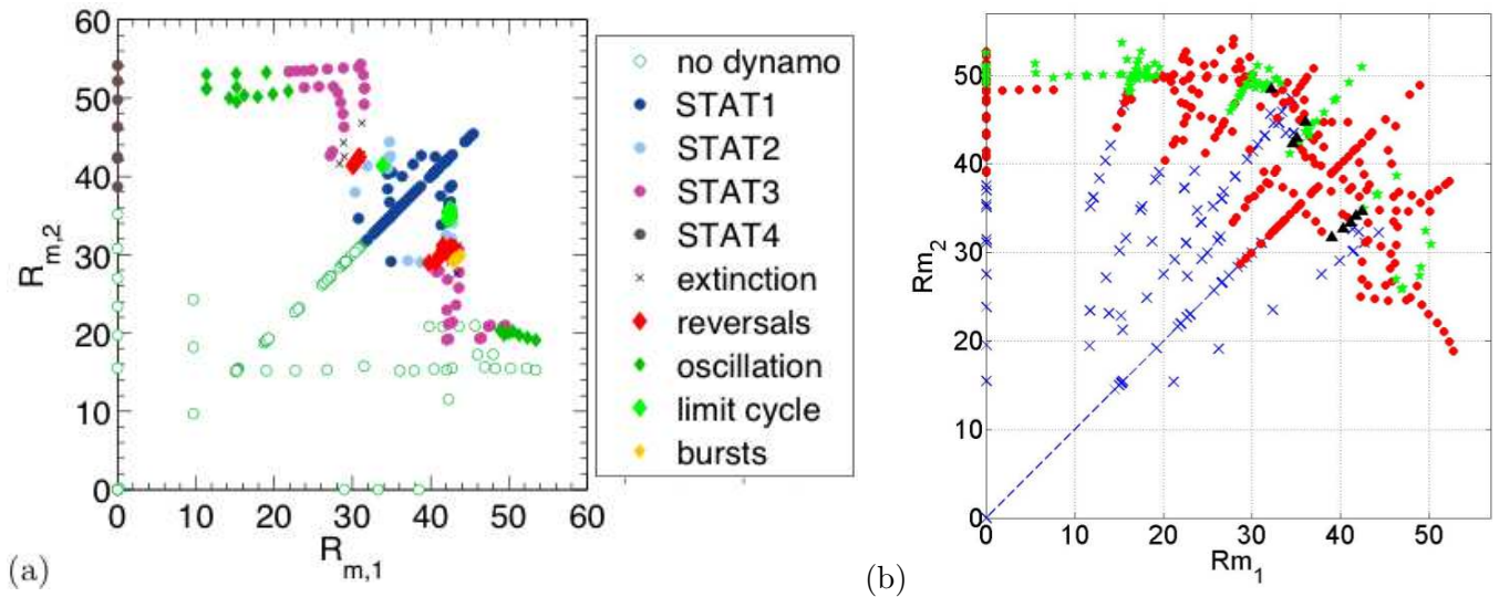
Figure 21: Parameter space: type of dynamo in the plane (Rm_1, Rm_2) . (a) Case with the full set of appendices. Figure from [31]. (b) same but without the annulus. x no dynamo (i.e. < 10G at the center). Red dots: stationary dynamos. Green stars: reversing/oscillating dynamos. Black triangles: intermittent dynamos. Dashed line: Rm_1 = Rm_2 . Figure from [5].
