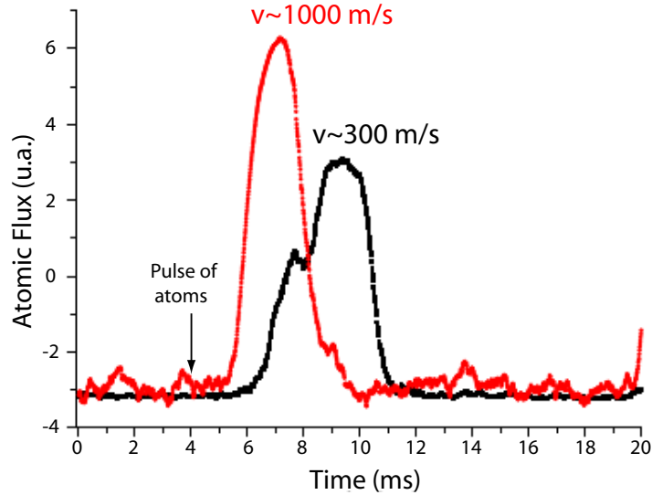
Figure 6.10: Effect of the first Zeeman slower on the atoms, measured using the channeltron. In red is the atomic signal without Zeeman slowing whereas the black curve corresponds to an atomic jet which has experienced longitudinal cooling. The shoulder of the black curve represents a fraction of atoms which do not experience the slowing effect and cannot be trapped in the MOT.
