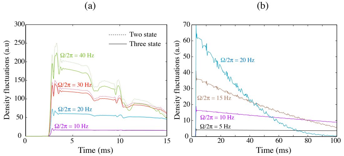
Figure 5.12: (a) Shows a comparison of the time-dependent density of the two- and three-state atom lasers at a point located 30 \mu\text{m} below the condensate, after 15 \text{ ms} of output coupling and for different Rabi frequencies in the low coupling regime. (b) Is the time-dependent density of the two-state atom laser measured at the same point, at very low intensities, after 100 \text{ ms} of output coupling. Parameters are N = 5 \times 10^4 atoms, \omega_z = 2\pi \times \frac{260}{\sqrt{2}} \text{ Hz} , U = 6.6 \times 10^{-4} , G = 9.24 , and \Delta = 43 .
