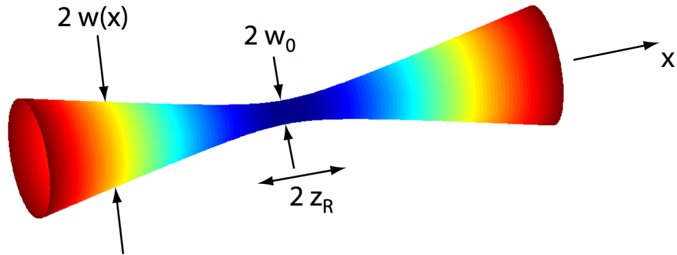
Figure 7.1: Laser beam profile of a single Gaussian beam of waist w_0 and Rayleigh length z_R .
