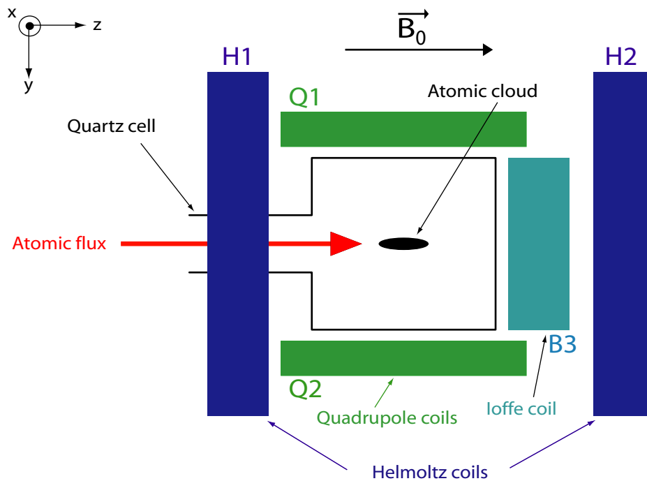
Figure 6.13: Schematics of the magnetic trap, where Q_1 , Q_2 and B_3 form the Ioffe-Pritchard trap whereas H_1 and H_2 are the Helmholtz coils that can compensate the bias field B_0 .
