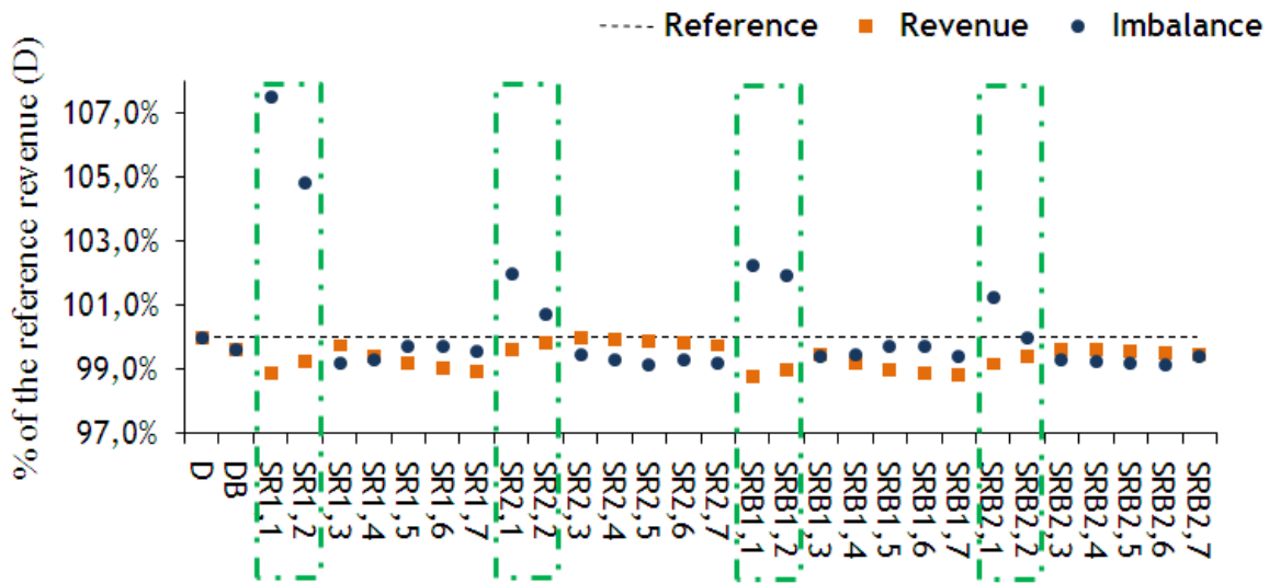
FIGURE 6.14: Total imbalance and revenue obtained for all the wind/pumped-hydro stochastic simulations. The reference deterministic simulations are the ones denoted by D and DB .
