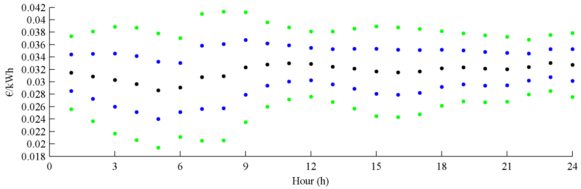
FIGURE 6.6: Forecasted day-ahead single-stage market price scenarios. Black dots correspond to day-ahead market price scenarios bearing a 0.50 probability of occurrence. Blue dots correspond to day-ahead market price scenarios bearing a 0.15 probability of occurrence. Green dots correspond to day-ahead market price scenarios bearing a 0.10 probability of occurrence.
