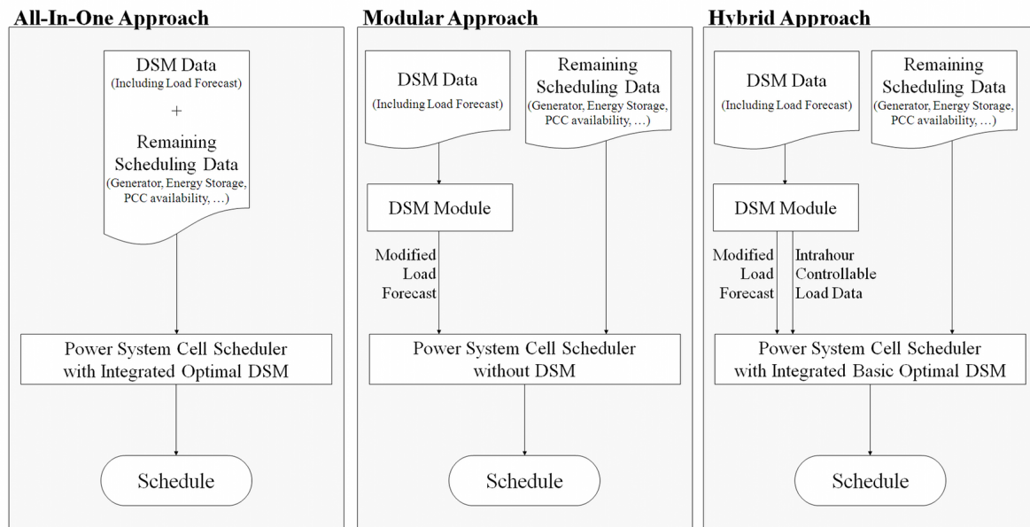
FIGURE 5.4: Three basic approaches for integrating demand side management (DSM) in the scheduling of the power system cell. The All-In-One Approach completely integrates DSM in the scheduling procedure. The Modular Approach completely separates DSM from the scheduling procedure. The Hybrid Approach is a mix of the previous ones separating the multi-stage DSM tasks (e.g.: definition load shifting actions) from the scheduling procedure. Such approach supplies the scheduler with data concerning intrahour load control possibilities, which enables the scheduler to perform optimal intrahour load control.
