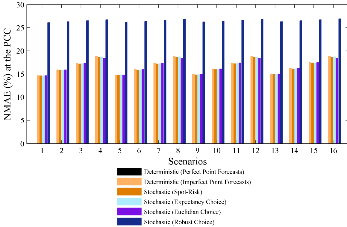
FIGURE 6.7: Mean absolute error at the point of common coupling (PCC) normalized by the peak PCC power flow that was obtained for the various decision-making options that were tested and for every scenario described in Table 6.2.
