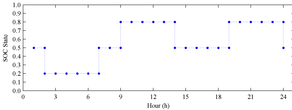
FIGURE 5.10: Representation of a state-of-charge preference rule in which the preferred state-of-charge is set to one of three predefined values (0.2, of 0.5, and of 0.8) while closely following the global time-dependent rule depicted in Figure 5.6.
