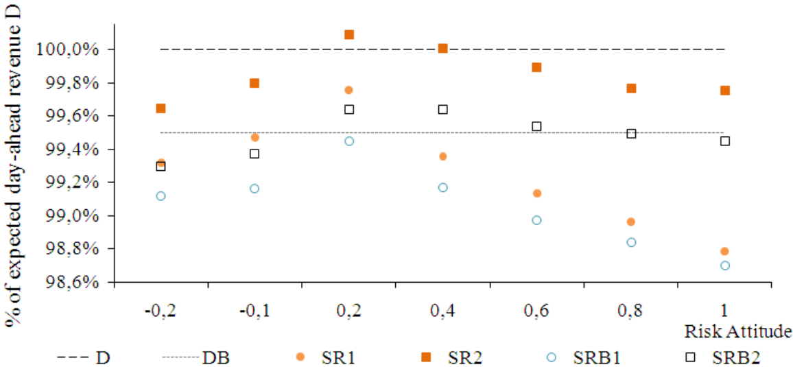
FIGURE 6.19: Day-ahead expected revenue achieved in the wind/pumped-hydro case-study for different risk attitudes \beta .
