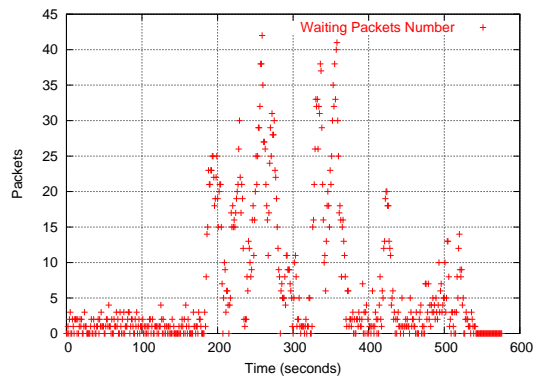
Figure 9.18: Waiting Packets (Test 1-Poisson)
