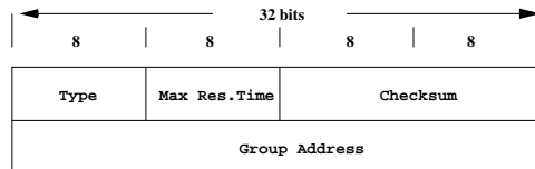
Figure 3.3: IGMPv2 packet format.
