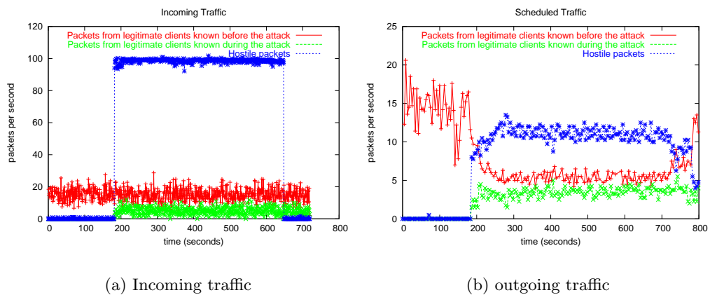
Figure 9.26: Traffic entering and leaving the filter (Test 3).
