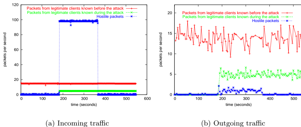
Figure 9.2: Traffic Entering and Leaving the Filter (Test 1).
