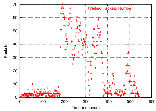
Figure 9.24: Waiting Packets (Test 2-Poisson)
