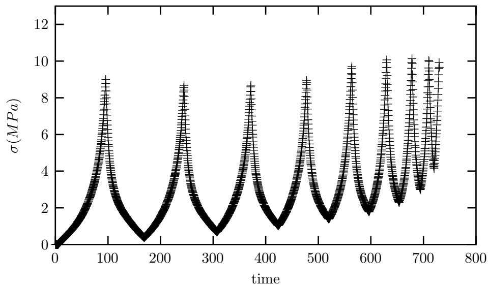
Figure I.25 : Evolution de la contrainte ( \sigma = \frac{F}{S} ) .
