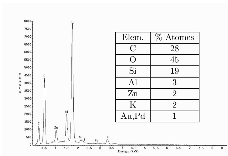
Figure III.43 : Aluminosilicate. Essai DIAB-TSTTC-10
