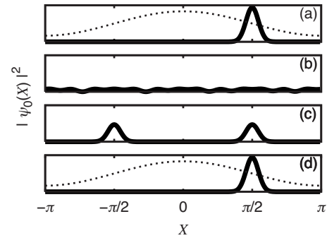
FIG. 1. Free evolution of a localized wave packet ( \beta=0 ) between two kicks for k=4\pi (note that the packet is shown in the interval X\in[-\pi, \pi] , but it reproduces itself periodically outside this range). (a) An initial wave packet centered at X=\pi/2 , (b) wave packet at t=0.115 , showing complete delocalization, (c) wave packet at t=0.25 , showing two replicas of the initial shape, (d) “reconstructed” wave packet at t=1^- , identical to the initial one. The vertical scale is the same for all the panels.
