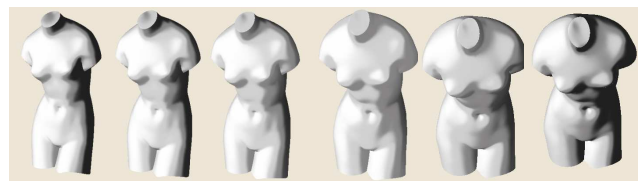
Figure 6: We show six frames of a small animation where coarser detail is automatically selected where the magnitude of optical flow is higher. We used the receding shadow texture from Figure 7.
