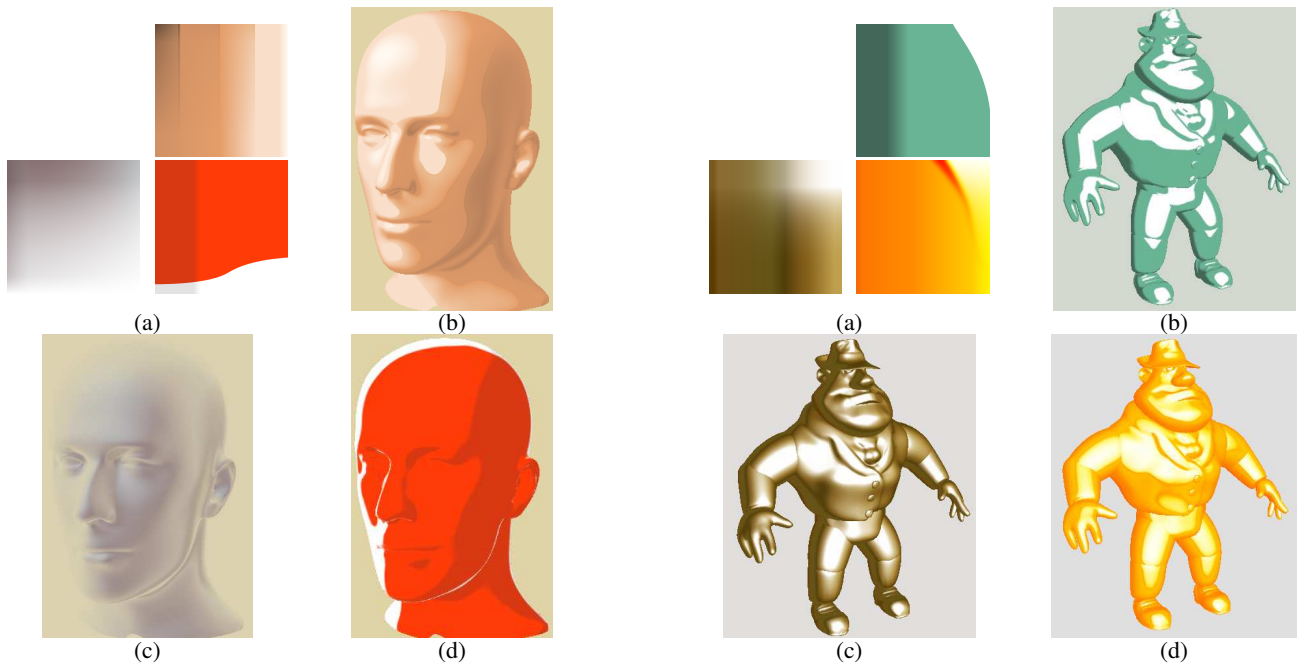
Figure 10: Near-silhouette abstraction and backlighting: (a) shows the textures used in (b), (c) and (d). In (b), we use a texture where intermediate tones are blurred prior to dark or light ones; this has the effect of smoothing out the shading in near-silhouette regions so that hard boundaries are only visible in regions facing the camera. In (c), the same approach is applied, this time to decrease opacity of the shading except for dark tones; this gives a fuzzy rendering of the model. In (d), we apply a simple white backlight that grows thinner in darker tones; we can thus control the thickness of the backlighting by moving the light.
