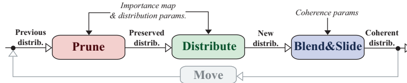
Figure 2: The different steps of our dynamic distribution algorithm: pruning, distribution, blending&sliding. A coherent non-uniform distribution is dynamically updated from frame to frame regardless of how the scene moved: 3D objects can be deformed, viewpoint motion is not restricted, and motion in video can be provided via its optical flow.
