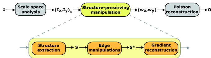
Figure 3: Overview of our method.
