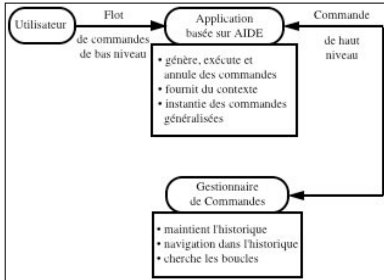
Figure 25 : Architecture de AIDE
