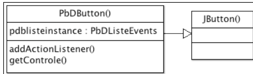
Figure 44 : La classe PbDButton
