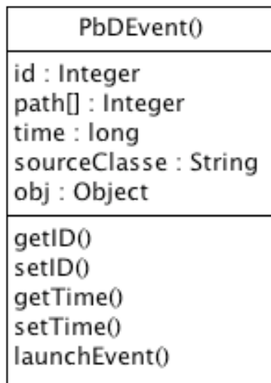
Figure 39 : La classe PbDEvent
