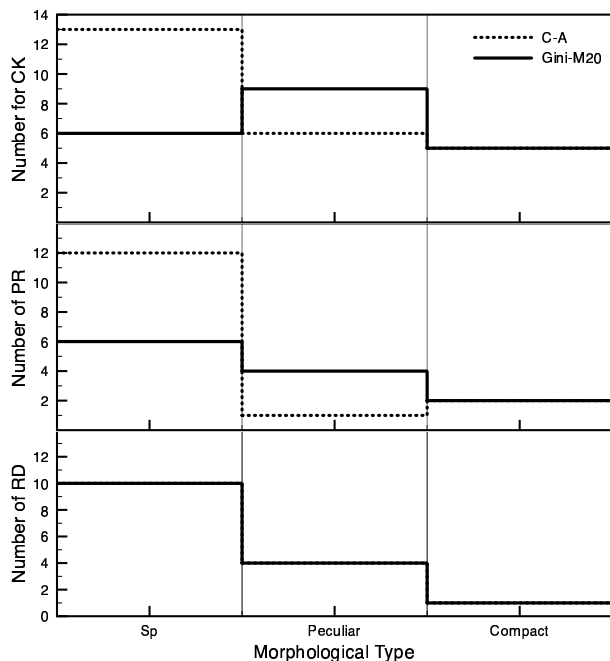
Fig. 7. Comparison between the concentration-asymmetry (dotted filled histogram), Gini-M20 (solid histogram) morphological classification, and the kinematical classification. Morphological classes are quoted in the bottom of X-coordinate, kinematical classes in Y-coordinate. RD refers to rotating disks, PR to perturbed rotations and CK to complex kinematics. The line for the CA and Gini/M20 exactly overlap for the RD types.
