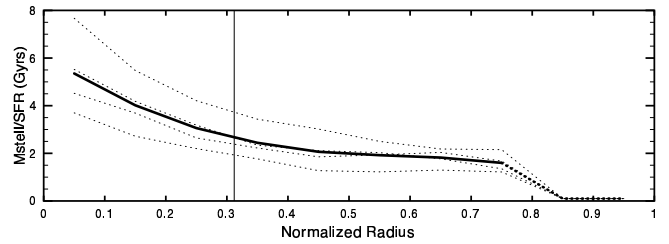
Fig. 11. Ratio between stellar mass and SFR_{tot} as a function of galaxy radius. SFR_{tot} is defined as the sum of SFR_{UV} and SFR_{IR} . Only galaxies which have been detected by Spitzer are used in this analysis. The vertical line is at 1/3.2 of R_{max} which roughly corresponds to the disk scale length limit.
