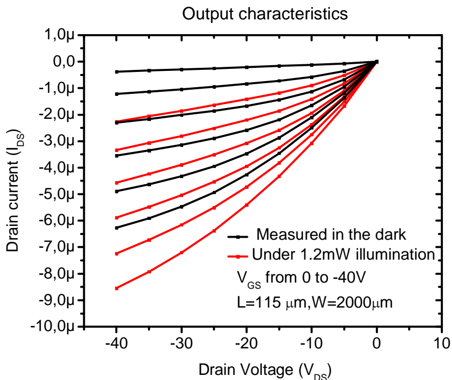
Figure 4.6: Output characteristics of a representative rubrene transistor in dark and under illumination showing clear photocurrent effects
