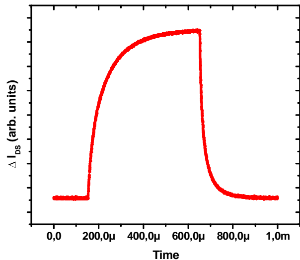
Figure 4.11: Representative photocurrent response under pulsed illumination
