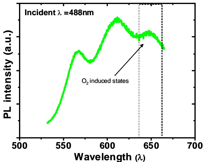
Figure 4.10: Photoluminescence spectra proving the presence of oxygen related band states on rubrene surface
