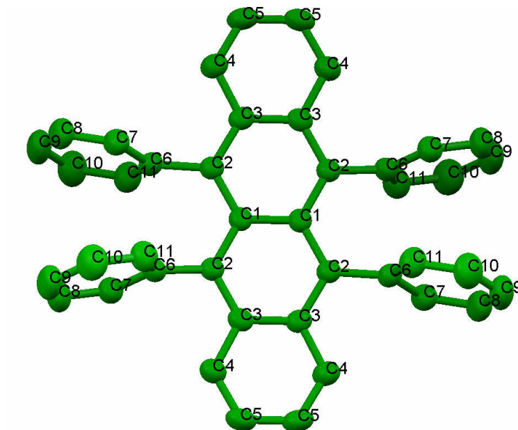
Figure 5.9: Geometrical structure of rubrene molecule extracted from single crystal diffraction 31
