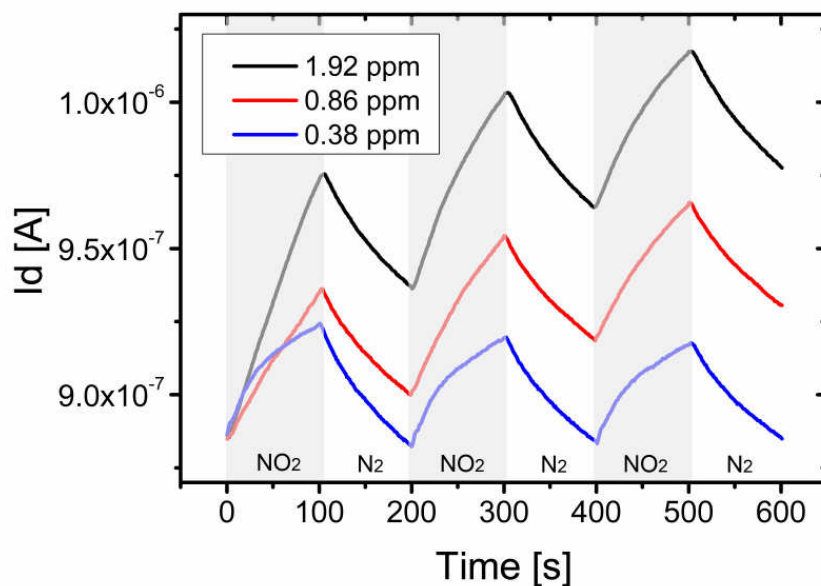
Figure 6.7: Variation of drain current with time on cyclic exposure to NO 2
