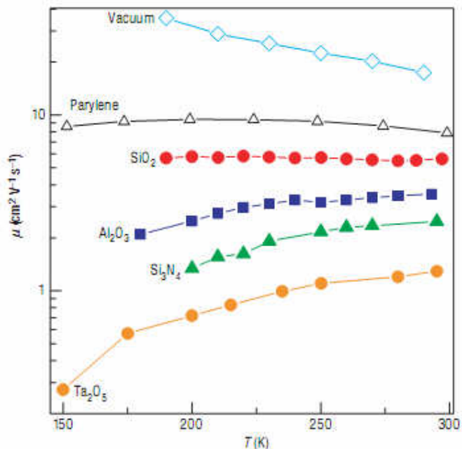
Figure 2.9: Temperature dependence of the carrier mobility for six different gate dielectrics. The temperature dependence evolves from metallic-like to insulator-like, as the dielectric constant is increased.
