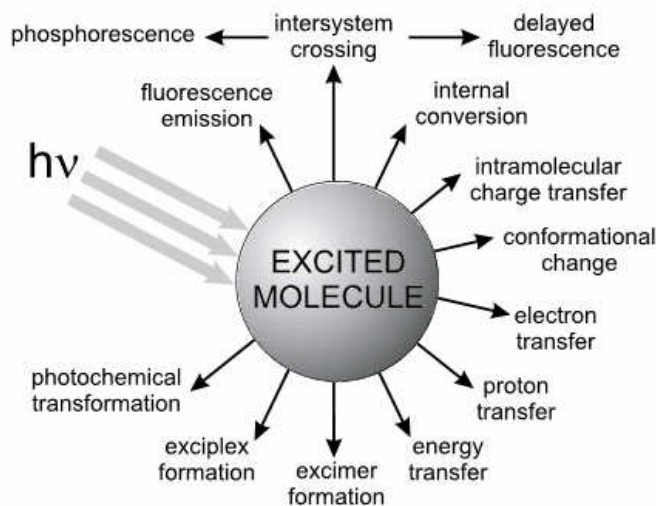
Figure 5.1: Possible de-excitation pathways of excited molecules
