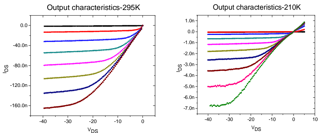
Figure 3.5: Output characteristics of a rubrene air-gap transistor ( L=300\ \mu\text{m} , W=1000\ \mu\text{m} ) measured at 295K and 210K illustrating contact effects.
