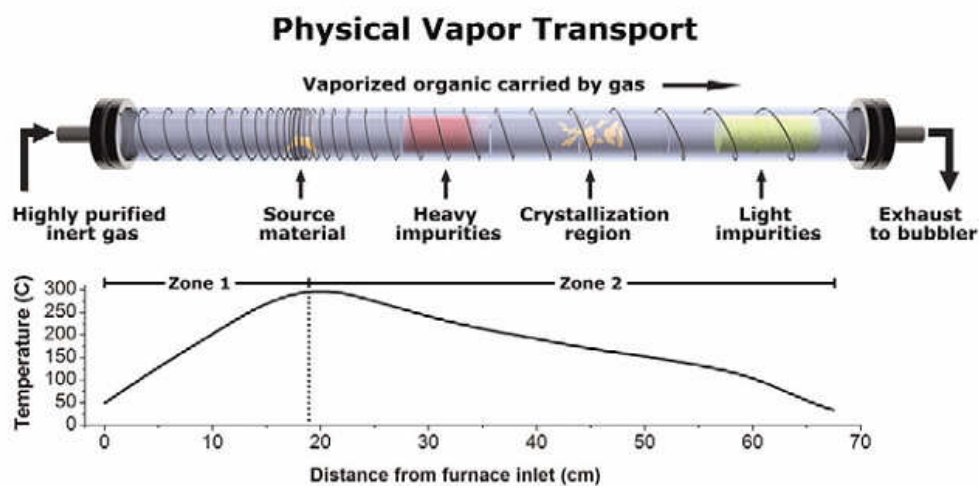
Figure 3.1: Schematic of the PVT crystal growth apparatus 8
