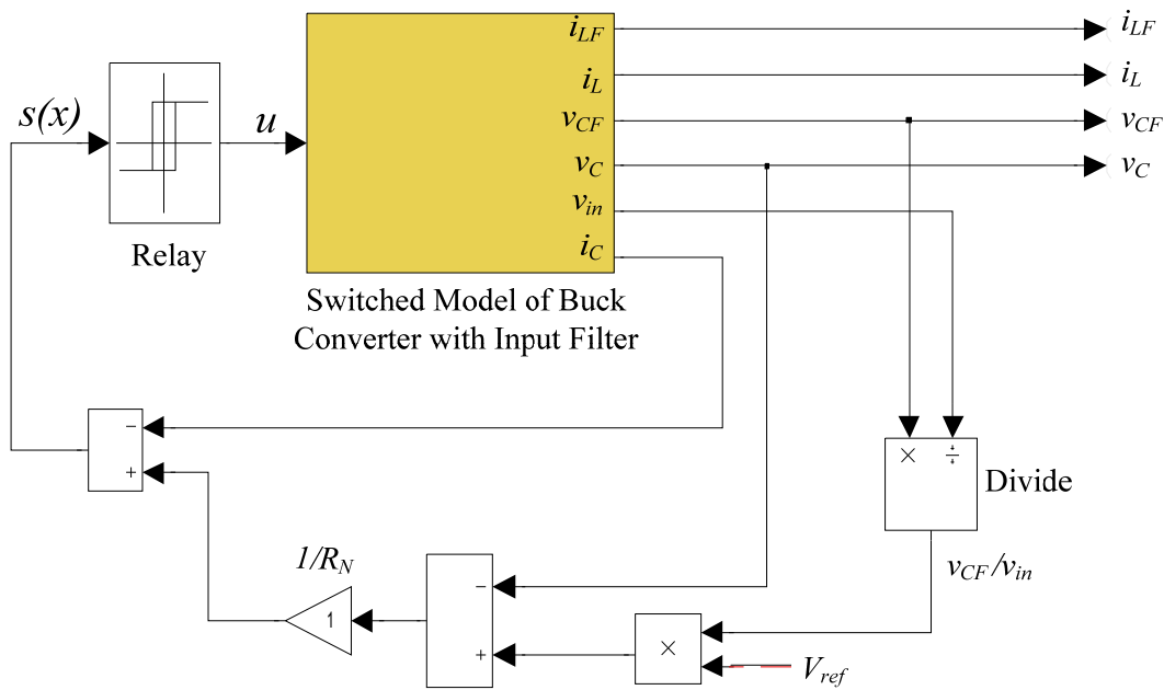
Fig. 5.13. Block diagram of a sliding-mode controller [nic95] for buck converter with input filter.
