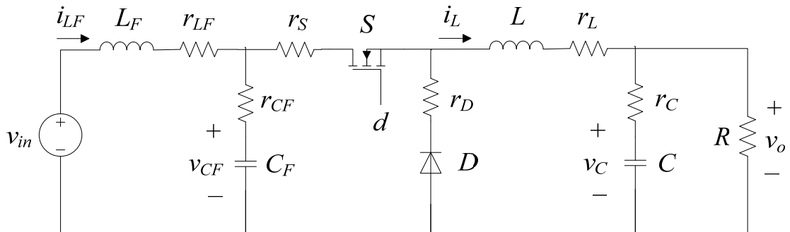
Fig. 2.1. Non-ideal buck converter circuit with input filter.
