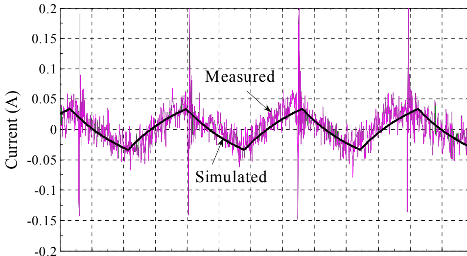
Fig. 4.15. Measured and simulated current i_2(t) in R_d - C_d branch for R_d = 10\Omega . (Parameter values: L_F = 4mH , C_F = 0.47\mu F , L = 0.8mH , C = 1\mu F , k = 10 , d = 0.5 , f_s = 112kHz , V_o = 24V and I_o = 0.18A )
