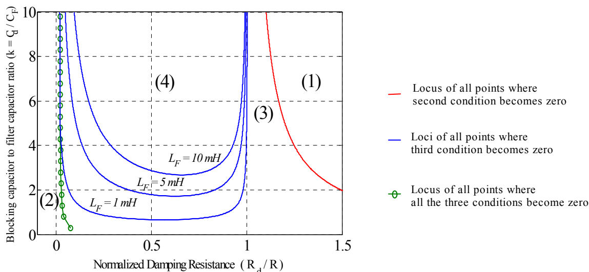
Fig. 3.21. Plot of stability conditions for buck-boost converter. (Parameter values: C_F = 4.7 \mu\text{F} , L = 0.1\text{mH} , C = 1 \mu\text{F} , R = 50 \Omega , V_{in} = 24\text{V} , D = 0.5 , r_s = r_D = 50\text{m}\Omega , r_{LF} = r_{CF} = r_L = r_C = 0.5 \Omega )
