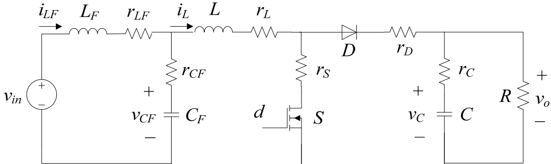
Fig. 2.3. Non-ideal boost converter circuit with input filter.
