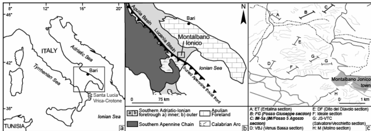
Figure 1. a: Geographical location of the studied area. b: Schematic geological map of the South-Eastern Italy. c: Zoom on Early to Middle Pleistocene sediments of the Montalbanio Jonico composite section. The two sections analysed in this study are in bold.
