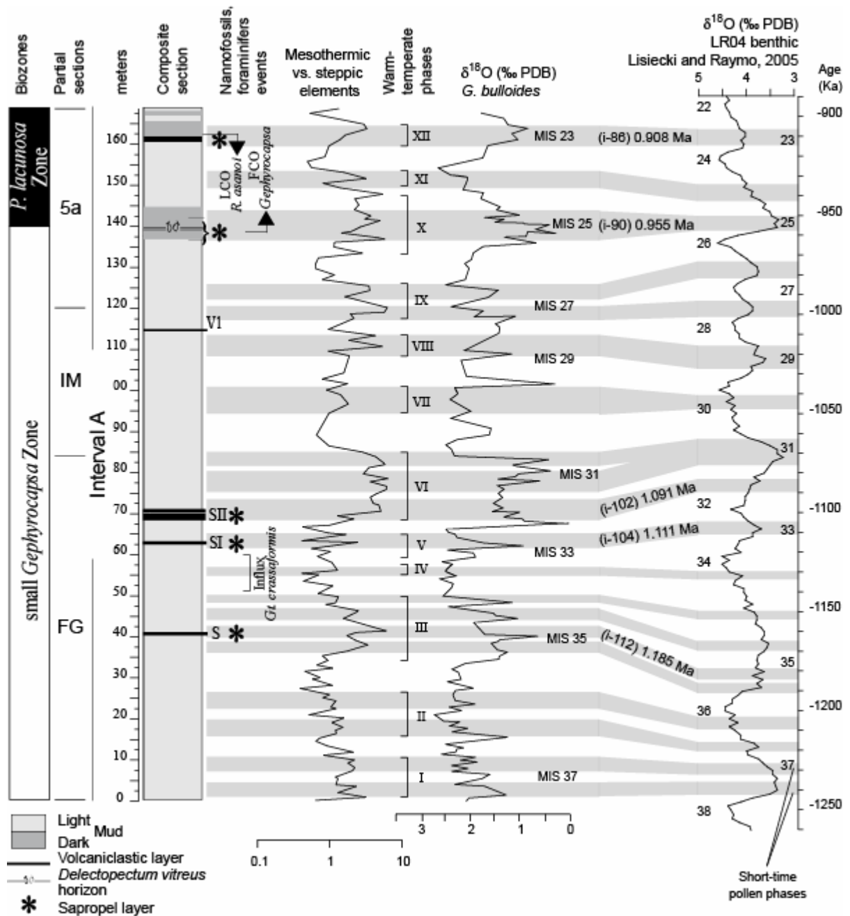
Figure 3. Lithological section, biostratigraphical events, pollen ratio “mesothermic vs. steppic elements” and main warm-temperate pollen phases (using roman numerals) compared to oxygen isotopic records from the same samples. Short-time warm-temperate pollen phases have grey shapes. Proposed marine isotopic stages are correlated with global oxygen isotopic record (Lisiecki and Raymo, 2005).
