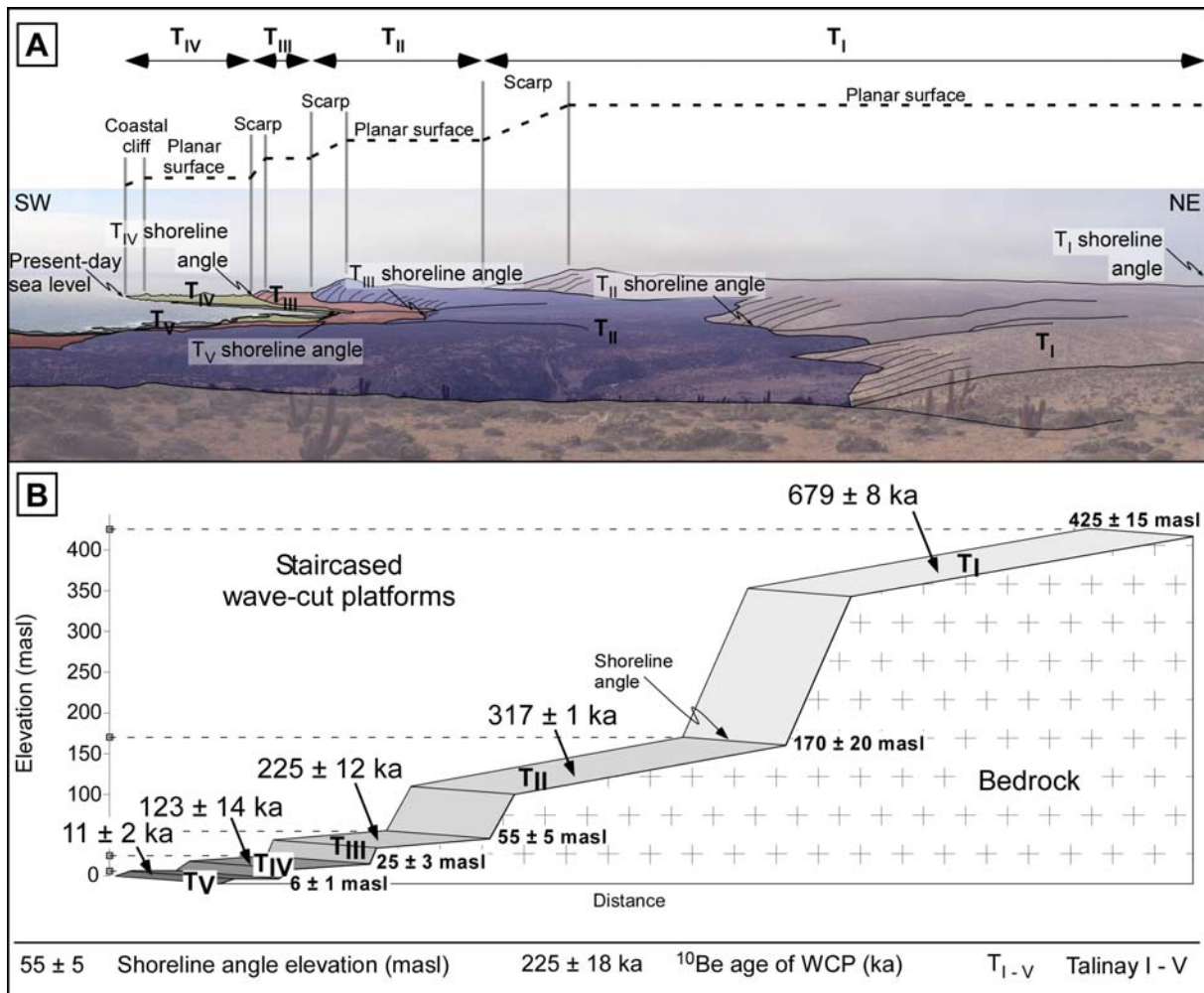
Figure 40 : A - Panoramic view of WCPs sequence near Mina Talca with their mean morphological features. T I , T II , T III , T IV , T V : Talinaly I, Talinaly II, Talinaly III, Talinaly IV, Talinaly V. B - Schematic cross-section of WCPs sequence and 10 Be age of each WCP (without horizontal scale). Dashed lines show shoreline angle elevation.
