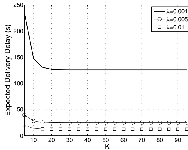
Figure 6.5: Expected delivery delay under K -transmissions MTR protocol for different values of K ( N=100 , \mu=0.001 ).
