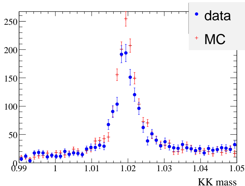
Figure 4.34: K^+K^- mass distribution for events with a reconstructed D_s^+ . Data (blue points) and MC (red) have been normalized to the same number of reconstructed D_s^+ mesons.
