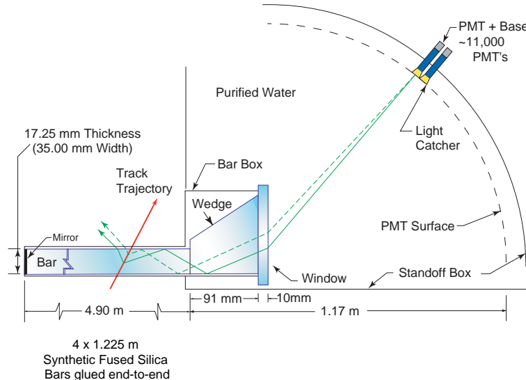
Figure 2.11: Schematics of the DIRC fused silica radiator bar and imaging region.
