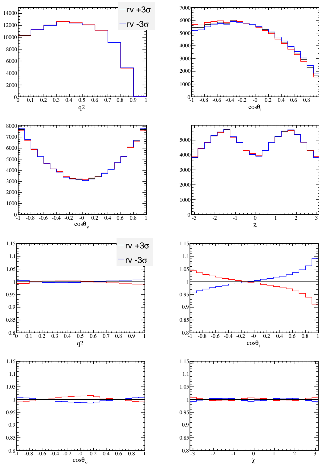
Figure 5.3: Distribution of the kinematic variables for different values of r_V . The reference histogram ( r_V^{ref} = 1.5 ) is in black. The bottom plots correspond to the ratio between the histograms r_V^{ref} \pm 3\sigma and the reference histogram.
