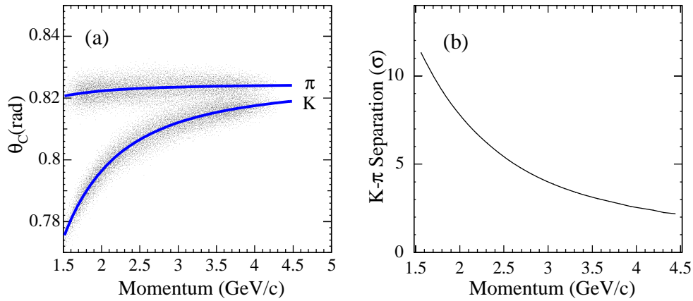
Figure 2.15: (a) The measured Cherenkov angle for pions (upper band) and kaons (lower band) from D^* \rightarrow D^0 \pi , D^0 \rightarrow K \pi decays reconstructed in data. The curves show the expected angle \theta_C as a function of laboratory momentum, for the K and \pi mass hypothesis. (b) The average difference between the expected value of \theta_C for kaons and pions, divided by the uncertainty, as a function of momentum.
