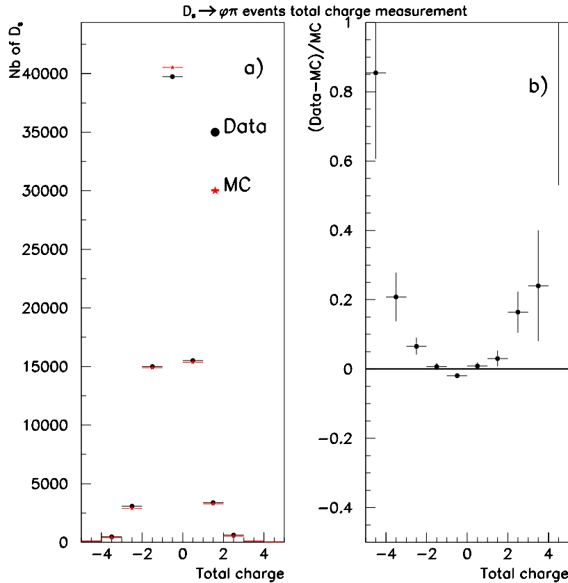
Figure 4.16: Charge imbalance distribution in events tagged with a D_s .
