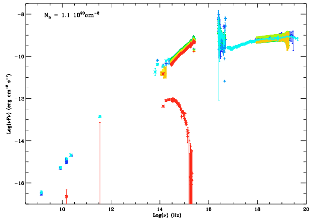
Figure 4. Spectral energy distribution for all the epochs overlotted.
