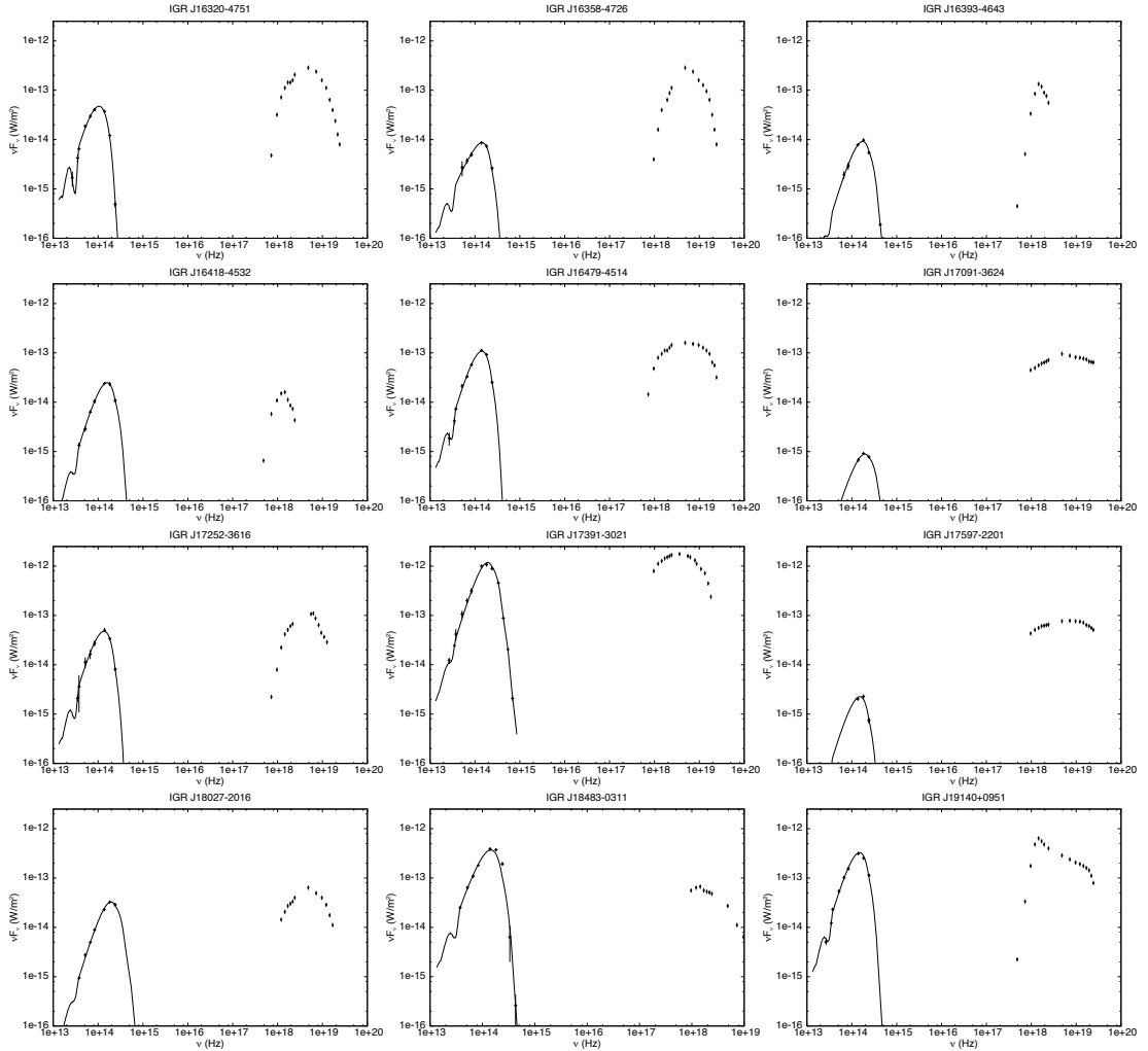
Fig. 1. SEDs of all these INTEGRAL sources, showing the observations from hard X-rays to MIR wavelengths. In each case, we overlaid the black-body emission representing the stellar spectral type of the companion star, which is given in Table 7 for the sources IGR J16393-4643, IGR J16418-4532, IGR J17091-3624, IGR J17597-2201, IGR J18027-2016 and IGR J18483-0311, and in Rahoui et al. (2008) for the remaining sources. See Section 2.4 for more details on the X-ray data. From top to bottom, and left to right: IGR J16320-4751, IGR J16358-4726, IGR J16393-4643, IGR J16418-4532, IGR J16479-4514, IGR J17091-3624, IGR J17252-3616, IGR J17391-3021, IGR J17597-2201, IGR J18027-2016, IGR J18483-0311 and IGR J19140+0951.
