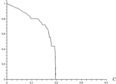
\dim_H F(c, 3)
