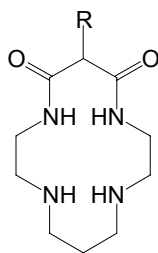
\text{L}^{16} (R = H) \text{L}^{22} (R = \text{CH}_2\text{C}_6\text{H}_5 )
