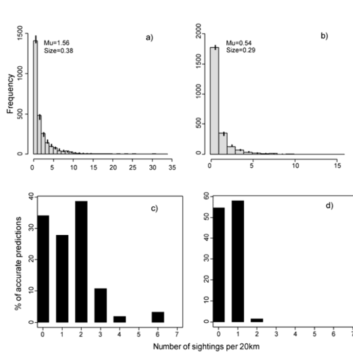
Fig 12. Graphs checking for validity and performance of our models. a) shows the statistical distribution of the response of the first model (number of sightings per bin of 20km). Black bars represent 95% confidence intervals of a negative binomial distribution fitted to the data whose parameters are reported on the graph. Confidence intervals are extracted from 999 simulations. b) idem for the second model. c) Accuracy of the first model, calculated as the percentage of good predictions obtained by the model when applied to the 50 % of the data not used to build the model. The percentage of good prediction had been calculated for every value of the response. d) idem for the second model
