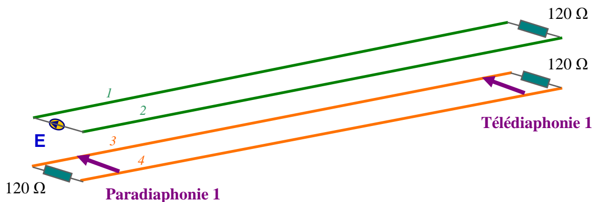
Figure IV.7 - Configuration 1
