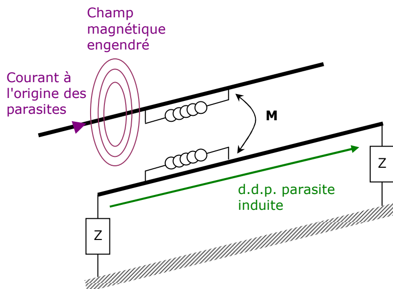
Figure I.11 - Diaphonie inductive
