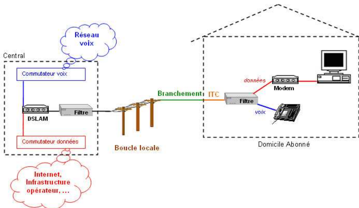
Figure I.13 - Architecture de raccordement des systèmes xDSL
