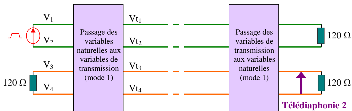
Figure IV.8 - Configuration 2
