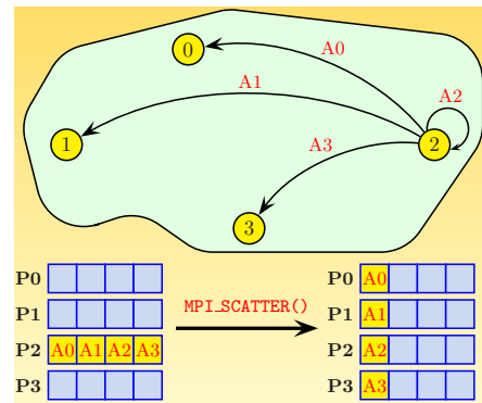
(b) MPI_Scatter
