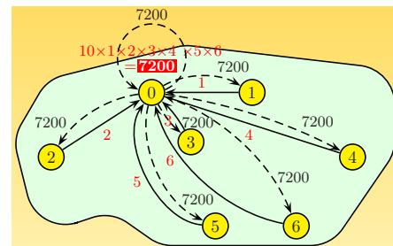
(f) MPI_Allreduce
