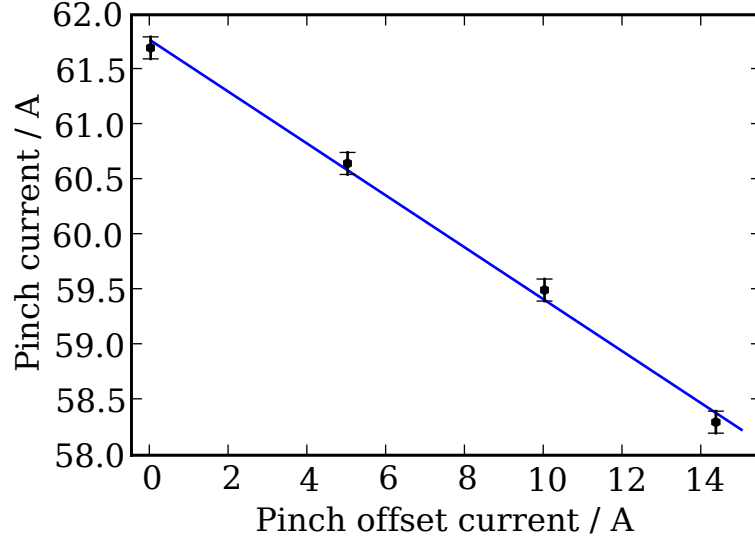
Figure 5.20: Calibration of the magnetic fields of the two coil systems. The points are the position of the p -wave resonance |1/2,1/2\rangle + |1/2,1/2\rangle . The fit of the points gives a calibration of I_{\text{pinch}} = 0,24I_{\text{offset}} .
