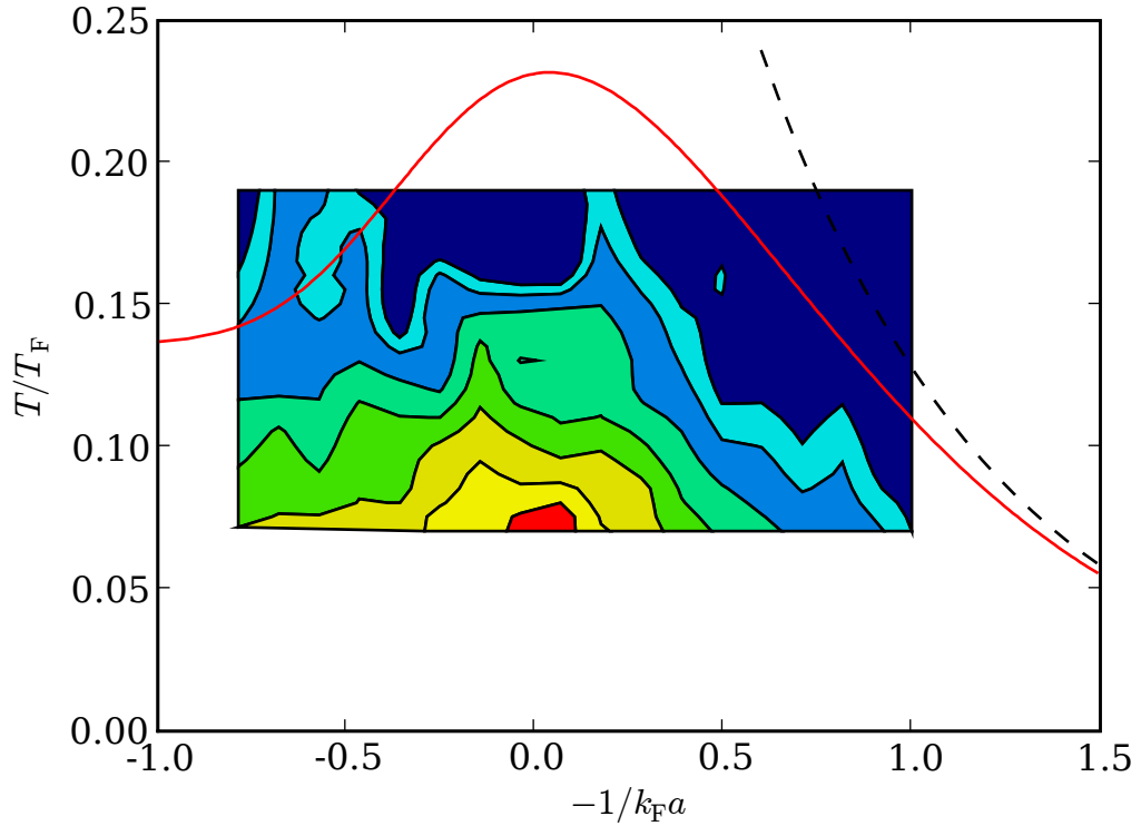
Figure 2.9: The transition temperature in the BEC-BCS crossover (solid line). The data in the background is a measurement taken in ^{40}\text{K} of the condensate fraction. Above the curve the gas is in the normal state, while we have a superfluid phase below. We note that there is no phase transition between a superfluid BEC on the left side and BCS superfluidity on the right. Both theory and data is by Chen et al. [27]. The colors correspond to a condensate fraction between 0 (dark) and 15,5% (bright). The curve is higher than the data since they could not measure a condensate fraction below 1%. The dashed line shows the transition temperature usually used to describe superconductivity in metals, it is the temperature below which pairing begins.
