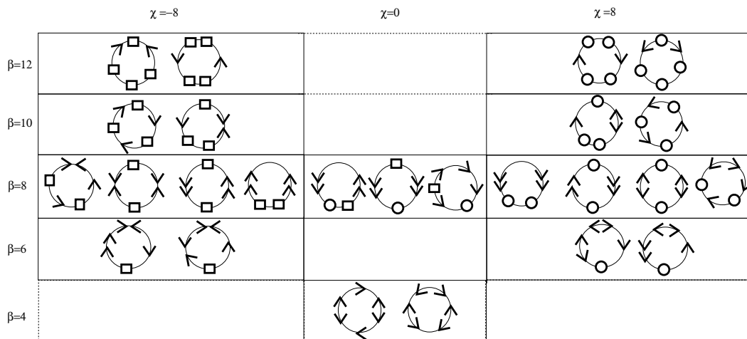
Fig. 6.16. List of necklace diagrams of real E(1) having only real critical values and admitting a real section.
