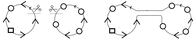
Fig. 6.14. An example of odd connected sum.
