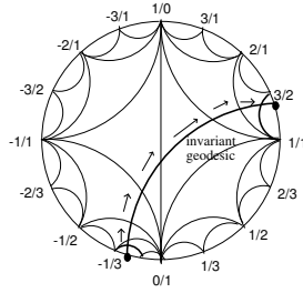
Fig. 3.6. Modular action of a hyperbolic matrix.
