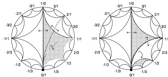
Fig. 3.10. Decompositions of modular actions of parabolic matrices P_1, P_2 .
