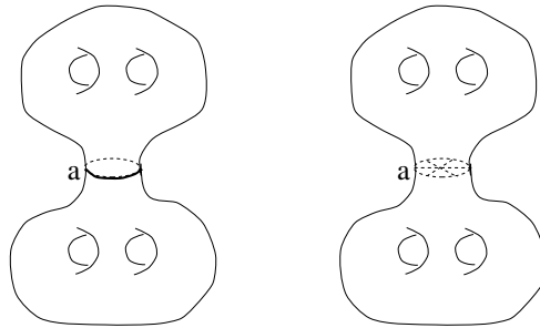
Fig. 4.11. Real and totally imaginary separating curves.
