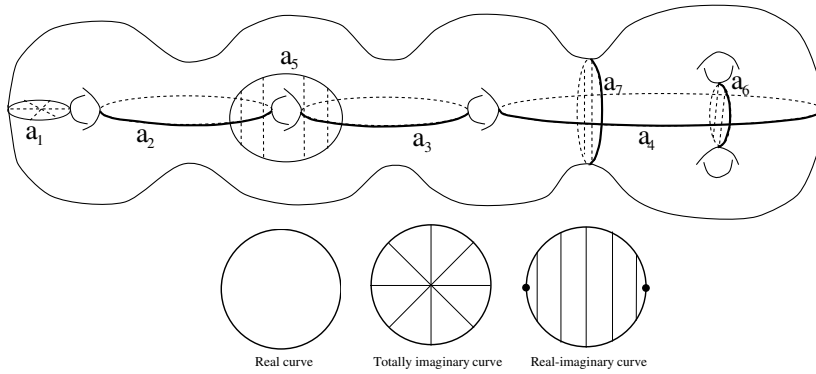
Fig. 4.7. c -invariant curves on (\Sigma_5, c) . We showed explicitly the action of c on a_1, a_2, a_3, a_4, a_5, a_6, a_7 .
