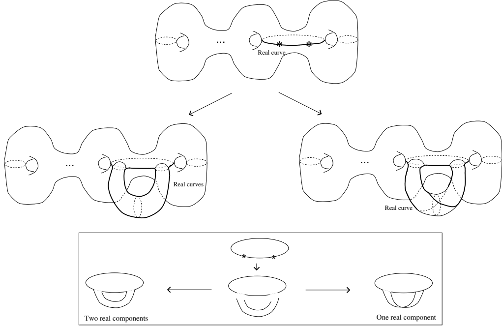
Fig. 4.9. Gluing neighborhood of the vanishing cycle to a real genus- (g - 1) surface with two real marked points belonging to the same real component.
