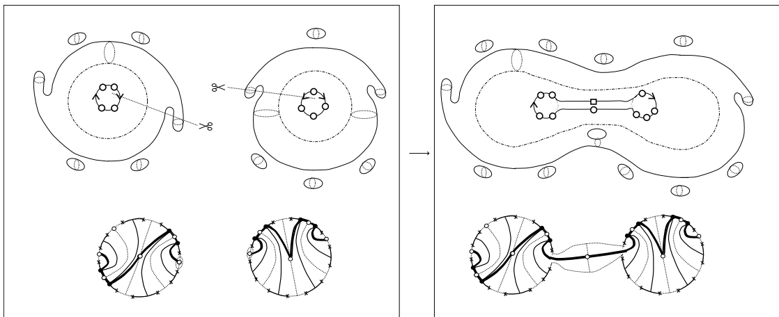
Fig. A.11. An example of even connected sum creating a maximal necklace diagram.
