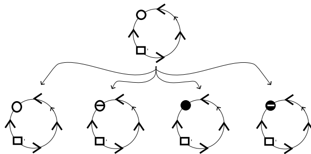
Fig. 6.7. An example of refinements of a necklace diagram.
