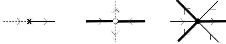
Fig. A.2. The graph around the inverse images of zeros of p, q, D .
