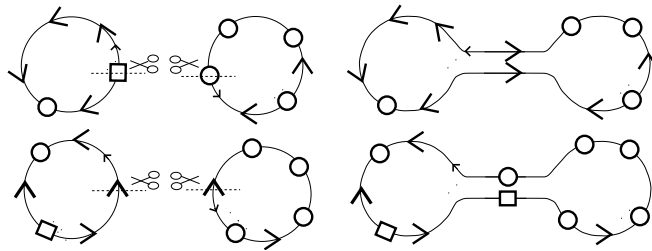
Fig. 6.15. Examples of even connected sums.
