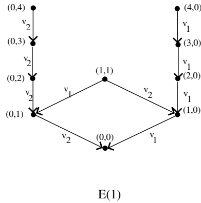
Fig. 6.20. Vertices of the graph correspond to the necklace diagrams of real E(1) whose real part has fixed topological type. Edges correspond to the transformations v_1 or v_2 .
