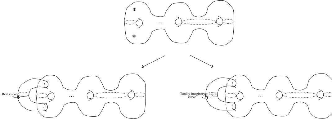
Fig. 4.8. Gluing neighborhood of the vanishing cycle to a real genus- (g - 1) surface with two complex conjugated marked points.
