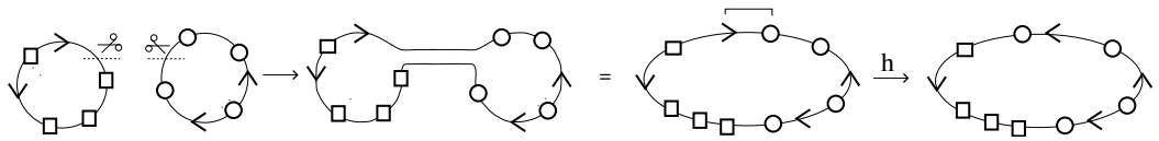
Fig. 6.18. An example of construction of a non-decomposable necklace diagram.
