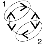
Fig. A.6. The number of essential intervals is 2 and there are 6 arrow type stones.
