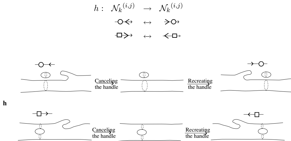
Fig. 6.9. The relation between transformations h and the real part of X .
