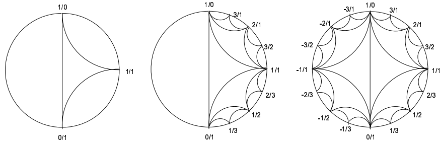
Fig. 3.3. Tessellation of \mathbb{D} .
