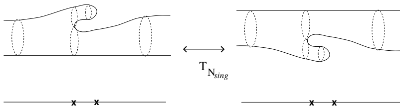
Fig. 5.18. The action of T_{N_{sing}} on the real part.
