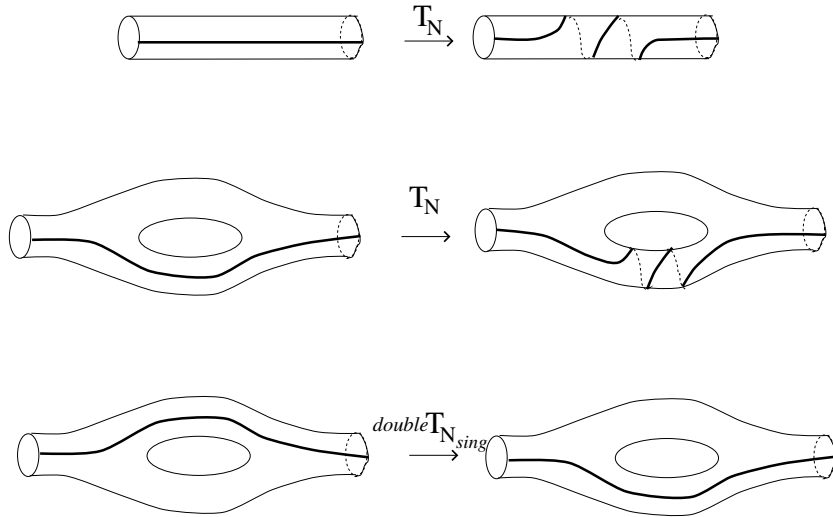
Fig. 5.20. Modification of the real section over the real part of D^2 .
