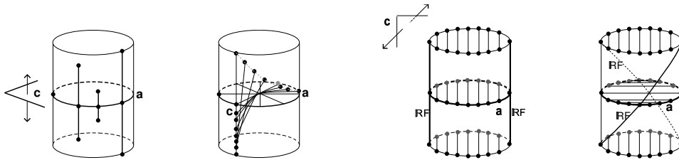
Fig. 4.6. Actions of the real structure on nearby regular fibers of \xi_{\pm} .
