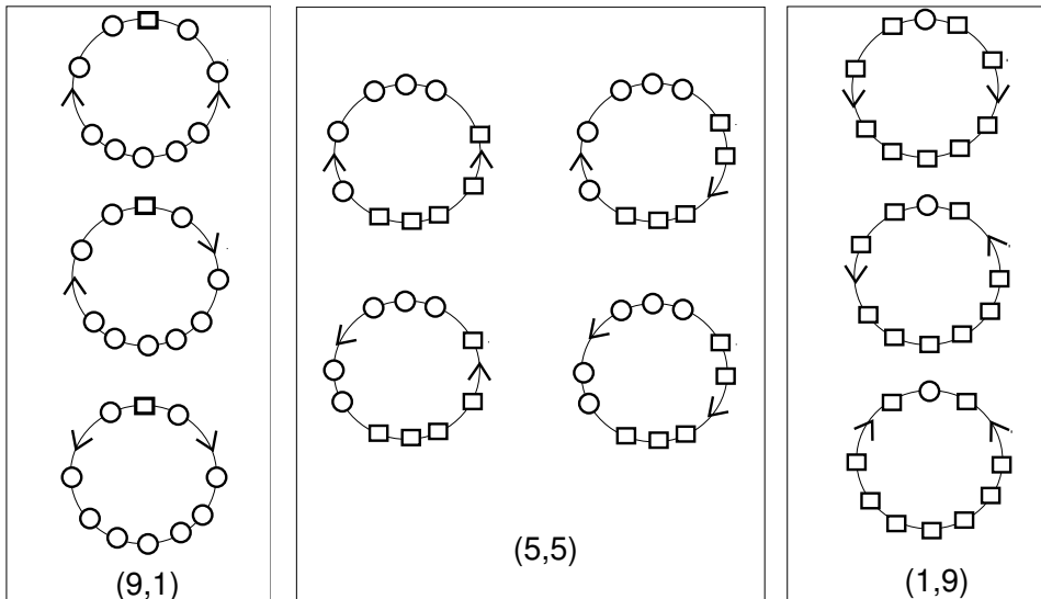
Fig. 6.17. List of necklace diagrams of maximal real E(2) having only real critical values and admitting a real section.
