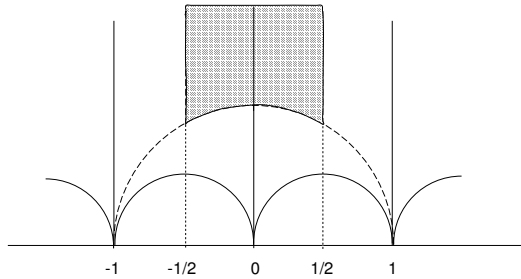
Fig. 3.2. The upper half plane model of hyperbolic space, and the standard fundamental domain of SL(2, \mathbb{Z}) .
