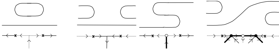
Fig. A.3. Because of the symmetry property we consider only one of the symmetric piece of real dessins d'enfants.
