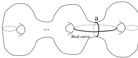
Fig. 4.12. Real-imaginary separating curve.
