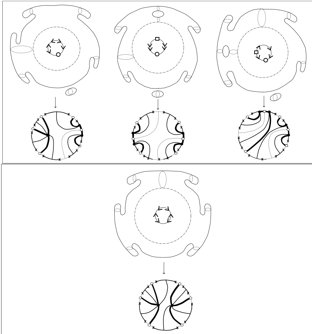
Fig. A.13. Around necklace diagrams, the real part of the corresponding real elliptic Lefschetz fibrations are shown. The dotted inner circle stands for a lift of the exceptional section.
