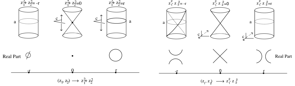
Fig. 4.2. Nearby regular fibers of \xi_{\pm} and vanishing cycles.
