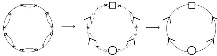
Fig. 6.4. Uncoated necklace diagram.
