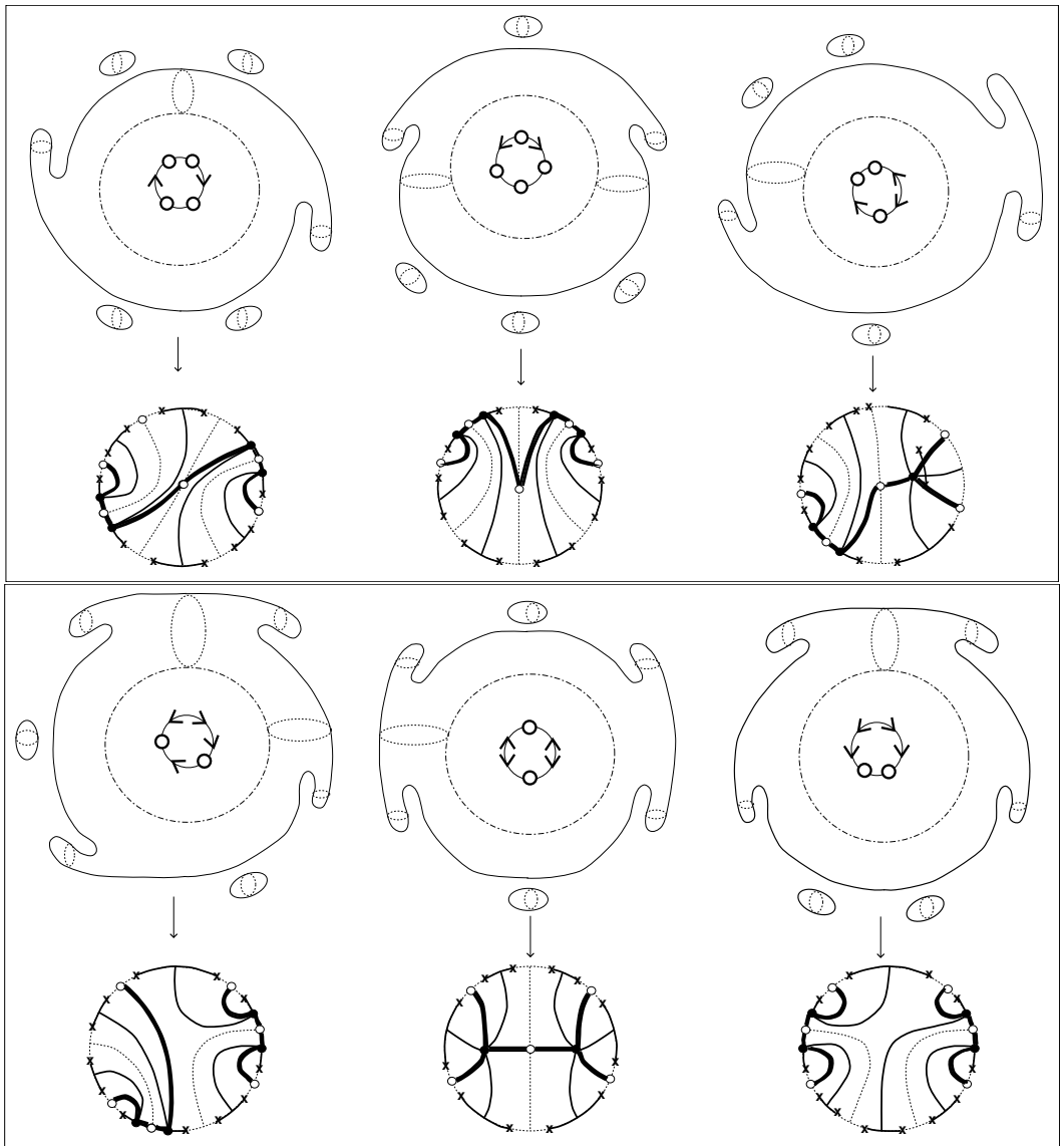
Fig. A.12. Around necklace diagrams, the real part of the corresponding real elliptic Lefschetz fibrations are shown. The dotted inner circle stands for a lift of the exceptional section.
