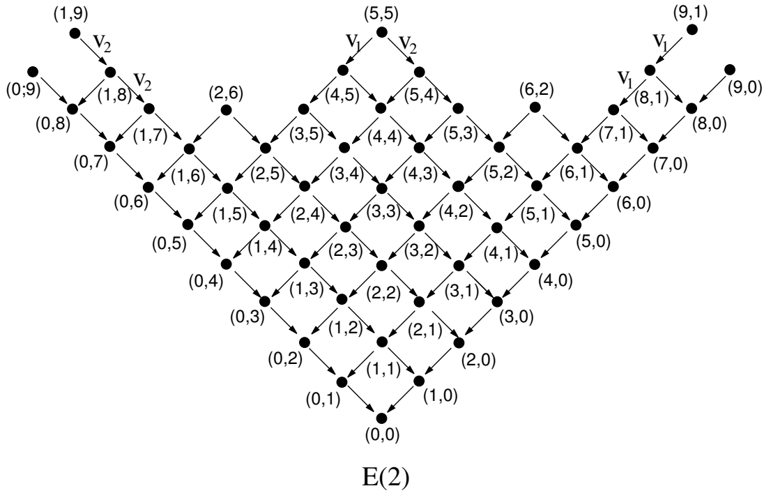
Fig. 6.21. Vertices of the graph correspond to necklace diagrams of real E(2) whose real part has fixed topological type. Edges correspond to the transformations v_1 or v_2 .
