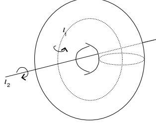
Fig. 5.5. Rotations generating Diff_0(\Sigma_1) .
