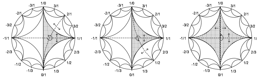
Fig. 3.9. Decompositions of modular actions of elliptic matrices.
