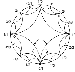
Fig. 3.5. Modular actions of parabolic matrices P_n .
