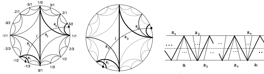
Fig. 3.7. Periodic pattern of the truncated triangles of the Farey tessellation.
