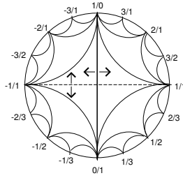
Fig. 3.8. Modular actions of linear real structures.
