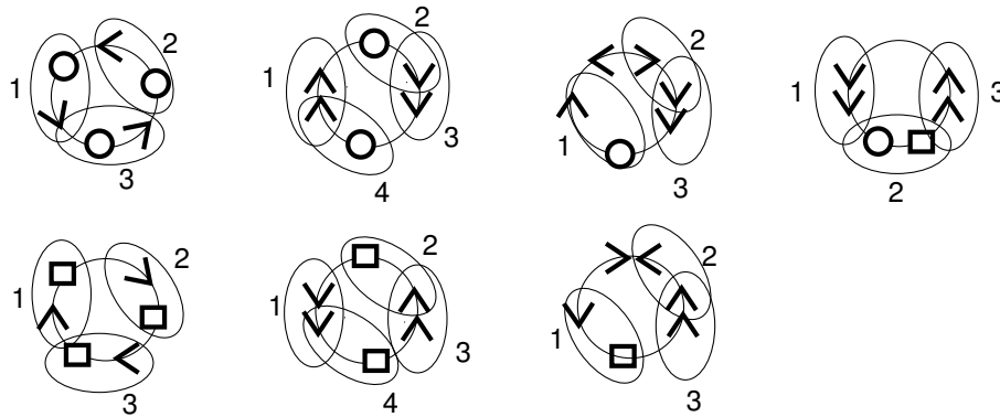
Fig. A.5. Necklace diagrams which contains more than 2 essential intervals.
