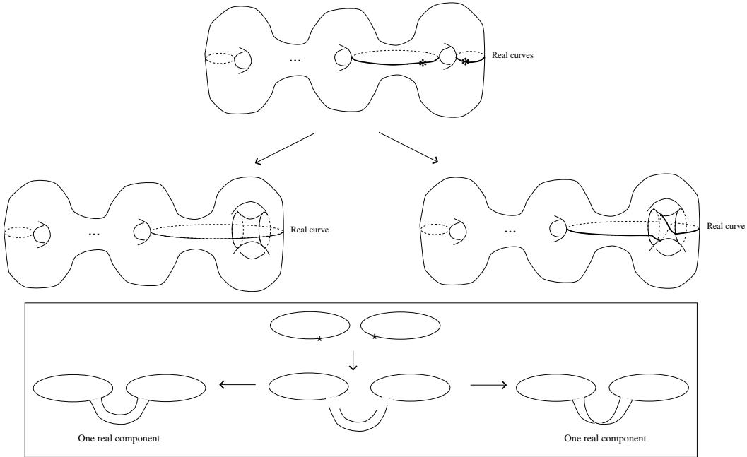
Fig. 4.10. Gluing neighborhood of the vanishing cycle to a real genus-( g - 1 ) surface with two real marked points belonging to different real components.
