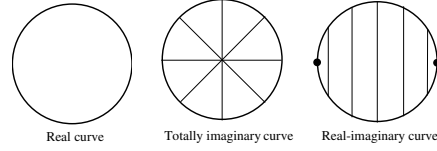
Fig. 4.5. Invariant curves together with the action of real structures.
