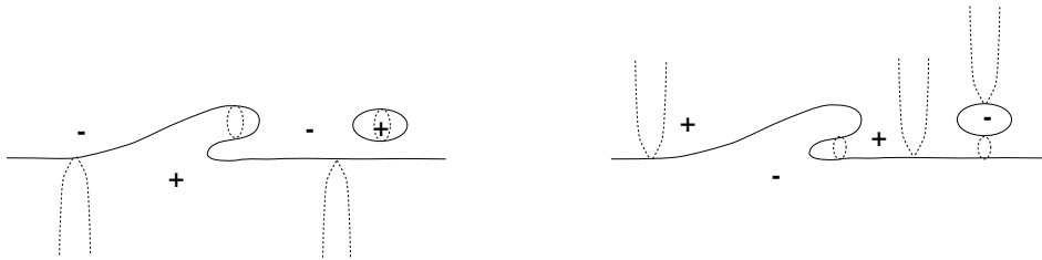
Fig. A.7. For each trigonal curve on H(2n) , there are two real structures of E(n) .
