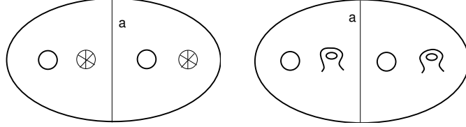
Fig. 4.15. Examples of k = 3, l = 2 .
