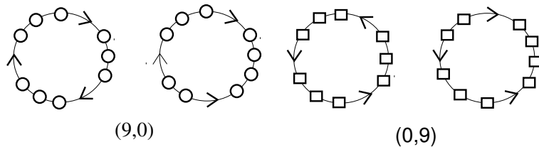
Fig. 6.19. Example of necklace diagrams which can not be obtained from the maximal necklace diagrams using v_1, v_2, h .
