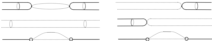
Fig. 6.8. Refinement of uncoated necklace diagram.
