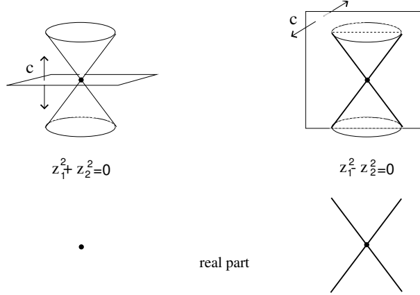
Fig. 4.1. Actions of real structures on the singular fibers of \xi_{\pm} .
