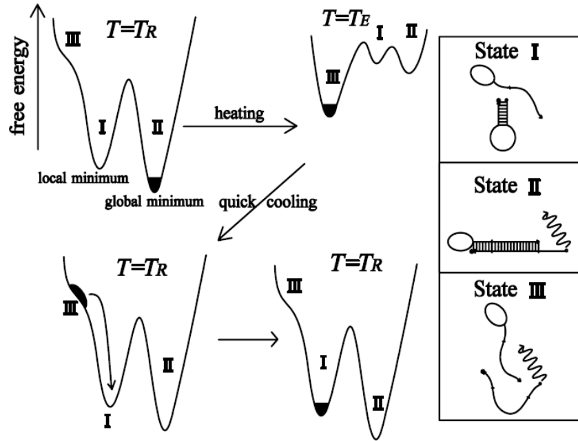
Figure 1.16: Schematic representation of the erasing process [45]. It is composed of the heating from T_R (room temperature) to T_E (erasing temperature) then cooling quickly from T_E to T_R .
