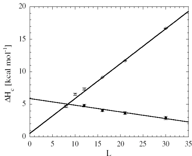
Figure 2.7: Closing enthalpy vs loop lengths (number of bases) of (\circ) poly(A) and (\bullet) poly(T) [37].
