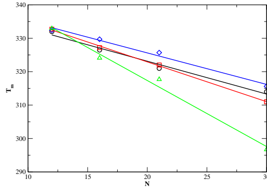
Figure 5.29: Variation of T_m as a function of the loop length N for different sets of parameters. \circ : experimental results for \text{poly}(T) ; \square : D=0.112 \text{ eV} , k=0.025 \text{ eV}\cdot\text{\AA}^{-2} , \alpha=6.9 \text{ \AA}^{-1} , \delta = 0.35 , \rho = 5 , \theta = 50^\circ ; \diamond : D=0.119 \text{ eV} , k=0.025 \text{ eV}\cdot\text{\AA}^{-2} , \alpha=6.9 \text{ \AA}^{-1} , \delta = 0.35 , \rho = 5 , \theta = 45^\circ ; \triangle : D=0.100 \text{ eV} , k=0.025 \text{ eV}\cdot\text{\AA}^{-2} , \alpha=6.9 \text{ \AA}^{-1} , \delta = 0.35 , \rho = 5 , \theta = 64^\circ
