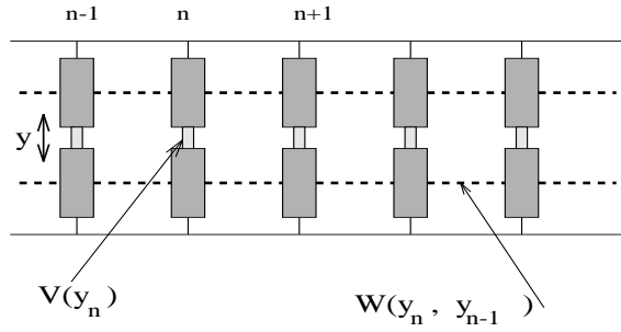
Figure 1.11: Peyrard-Bishop model for DNA.
