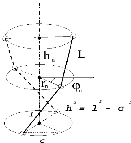
Figure 1.12: DNA Helicoidal Model [33].
