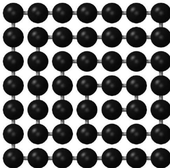
Figure 3.9: A compact conformation of the 49-mer on the square lattice [21].
