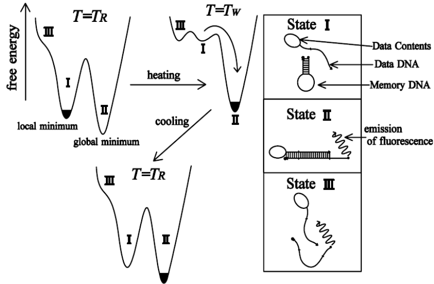
Figure 1.15: Schematic representation of the writing process [45]. It is composed of the heating from T_R (room temperature) to T_W (writing temperature) then cooling from T_W to T_R .
