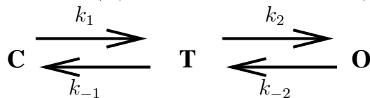
Figure 5.12: Chemical equilibrium.
