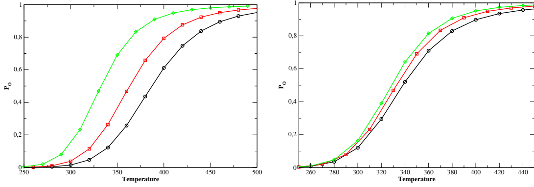
Figure 5.21: Effect of \alpha and \rho on the melting curve. The parameters are the following: D=0.107 \text{ eV} , k=0.025 \text{ eV.\AA}^{-2} , \alpha=6.9 \text{ \AA}^{-1} , \delta = 0.35 , \theta = 60^\circ . Left: Effect of \alpha , \bullet : \alpha=4.0 \text{ \AA}^{-1} ; \square : \alpha=5 \text{ \AA}^{-1} ; \diamond : \alpha=6.9 \text{ \AA}^{-1} . Right: Effect of \rho , \bullet : \rho = 2 ; \square : \rho=5 ; \diamond : \rho=10 .
