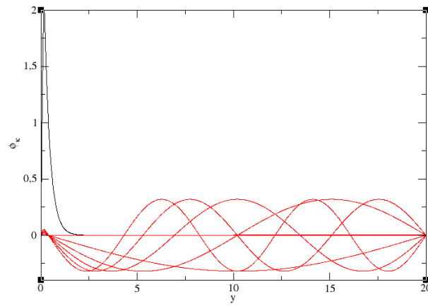
Figure 5.4: Representation of eigenfunctions.
