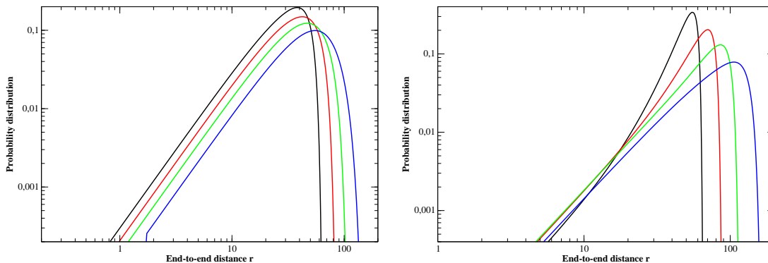
Figure 5.19: Plot of the probability distribution of the Kratky-Porod chain. Left: T=330 K, \epsilon=0.0019 \text{ eV} \cdot \text{\AA}^{-2} ; black: N=12 ; red: N=16 ; green: N=21 ; blue: N=30 . Right: T=275 K, \epsilon=0.0040 \text{ eV} \cdot \text{\AA}^{-2} ; black: N=12 ; red: N=16 ; green: N=21 ; blue: N=30
