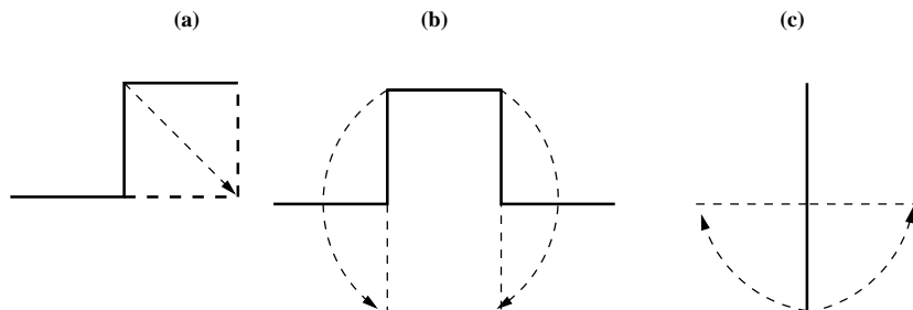
Figure 4.2: three possible motions: (a), flipping of a corner of a lattice cell with respect to the diagonal of the cell; (b) crank mechanism; (c), change of the angle between the two segments at one end of the chain.
