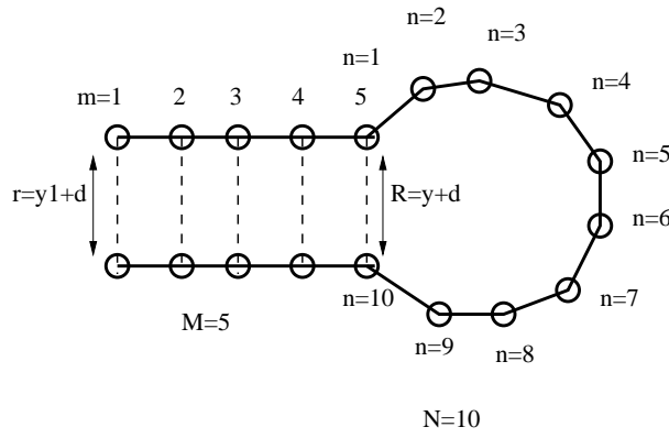
Figure 5.1: Plot of the model to define some notations. Index m=1 \dots M will be used for the stem base-pairs. Index n=1 \dots N+1 will be used for the bases in the loop. Note we have 2M+N-1 bases in total. The variables y_m are the stretching of the base pairs y_m = 0 means that the distance between the bases is d=10\text{\AA} , which is the value that we use for the equilibrium distance of bases in a pair. The variable r will be used for the variation of the distance between the two bases at the end of the hairpin, i.e. r=y_1+d . The variable R is the distance between the two ends of the loop. Therefore R=y_M+d .
