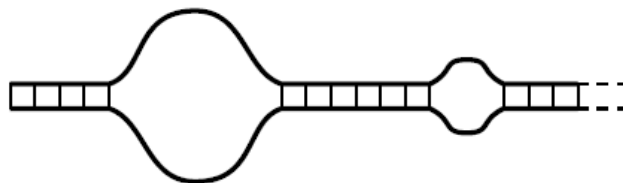
Figure 1.9: Schematic representation of the Poland-Scheraga model.
