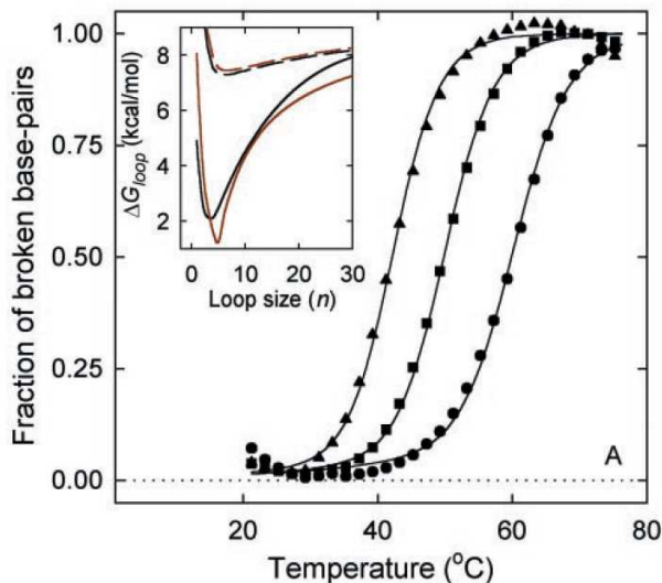
Figure 2.10: Fits to the equilibrium melting profiles. The symbols are normalized absorbance: ●, N=4 ; ■, N=8 ; ▲, N=12 ; the lines are the fraction of broken base-pairs. \Delta G_{loop} is the free energy of forming a loop closed by an A-T base-pair and is obtained by the model: red and black curve is the test of different \sigma_{loop} [6].
