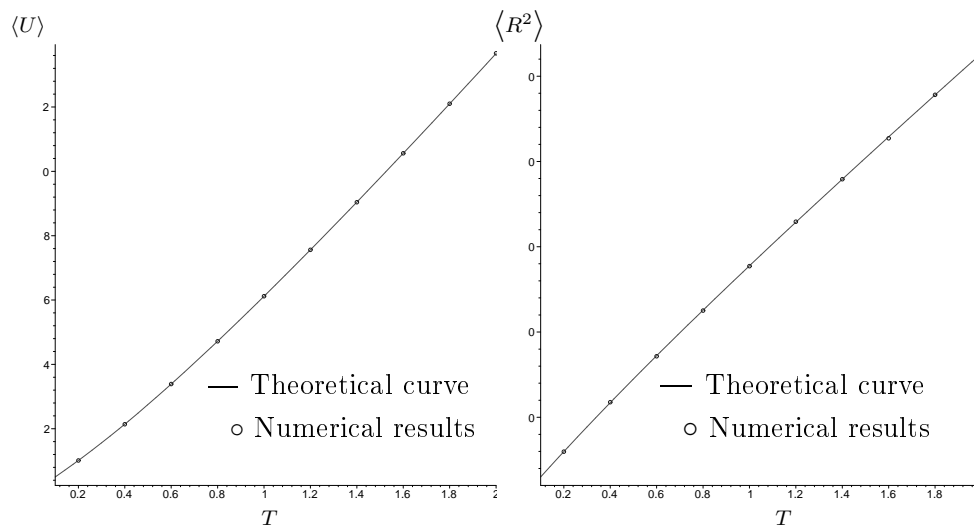
Figure B.3: potential energy of the chain and square mean end-to-end distance. Left: potential of the chain. Right: square mean end-to-end distance.
