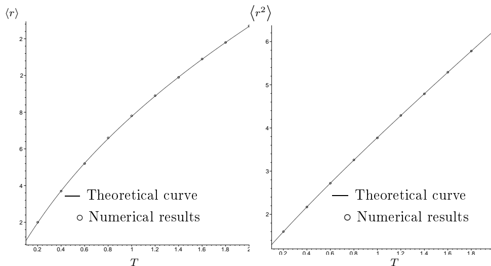
Figure B.2: Square mean length and mean length of a monomer. Left: mean length. Right: square mean length
