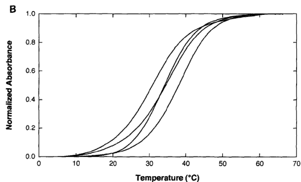
Figure 1.8: Melting curves example. The solution conditions were 10 nM sodium phosphate, pH 7.0, 1.0 M sodium chloride and a strand concentration of 2\mu\text{M} . The duplex sequences are GCAAAGAC/GTCTTTGC, GCATAGAC/GTCTATGC, GCAGAGAC/GTCTCTGC, and GCACAGAC/GTCTGTGC, with melting temperature of 33.7, 30.6, 35.7, and 38.5 °C, respectively [18].
