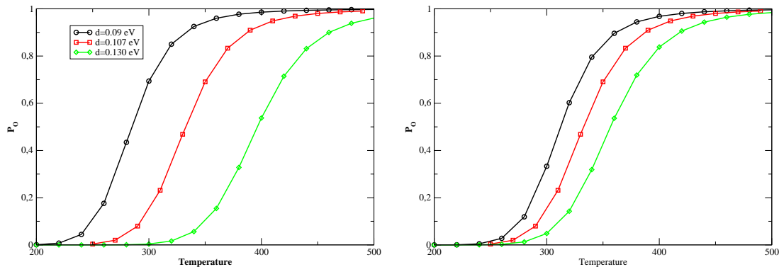
Figure 5.20: Effect of D and k on the melting curve. The parameters are the following: \alpha=6.9 \text{ \AA}^{-1} , \delta = 0.35 , \rho = 5 , \theta = 60^\circ , N=21 . Left: Effect of d , k=0.025 \text{ eV.\AA}^{-2} ; \bullet : D=0.09 \text{ eV} ; \square : D=0.107 \text{ eV} ; \diamond : D=0.13 \text{ eV} . Right: Effect of k , D=0.107 \text{ eV} ; \bullet : k=0.013 \text{ eV.\AA}^{-2} ; \square : k=0.025 \text{ eV.\AA}^{-2} ; \diamond : k=0.050 \text{ eV.\AA}^{-2} .
