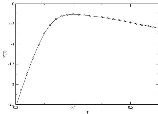
Figure 5.6: Free energy of a finite stem. The parameters are the following: D=4 ; a=0.1 , K=6 and N=5 in arbitrary units
