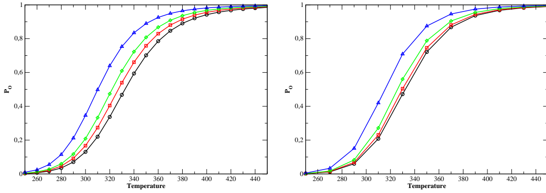
Figure 5.28: Melting curves equivalent to \text{poly}(T) with the FRC model. The parameters of the stem are: k=0.025 \text{ eV}\cdot\text{\AA}^{-2} , \alpha=6.9 \text{ \AA}^{-1} , \delta = 0.35 , \rho = 5 . Left: Melting profiles, D=0.112 \text{ eV} , \theta = 50^\circ ; \circ : N=12 ; \square : N=16 ; \diamond : N=21 ; \triangle : N=30 . Right: melting profiles, D=0.119 \text{ eV} , \theta = 45^\circ ; \circ : N=12 ; \square : N=16 ; \diamond : N=21 ; \triangle : N=30 .
