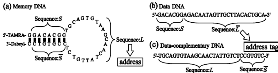
Figure 1.14: Schematic representation of the memory DNA and the data DNA [45]. (a) Memory DNA: a fluorescent dye TAMRA is attached to the 5'-end and its quencher Dabcyl is attached to the 3'-end. (b) Data DNA: a data DNA has a complementary base sequence of the loop and the 3'-stem of the memory DNA. (c) Data-complementary DNA: a data-complementary base sequences of S and L , respectively.
