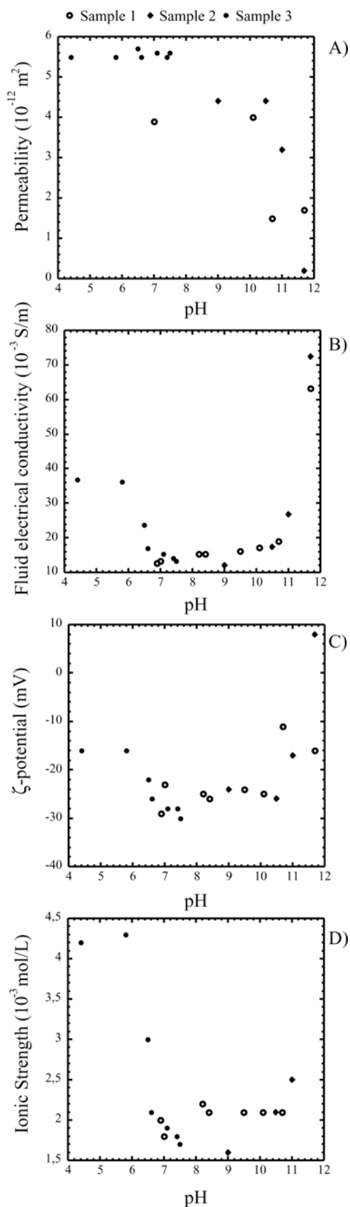
Figure 5. a: Variation of the permeability of the samples as a function of pH b: Variation of the electrical conductivity of the aqueous solutions, after flowing through the sand, as a function of pH c: Variation of the \zeta -potential derived from equation (1) using F=4.8 , \sigma_s=10^{-4} \text{ S/m} and m=1.3 , as a function of pH d: Variation of the ionic strength of the aqueous solutions as a function of pH calculated using the chemical analyses and WATEQ program [Plummer et al. , 1976]. The ionic strength is not calculated for experiments run at pH higher than 11.
