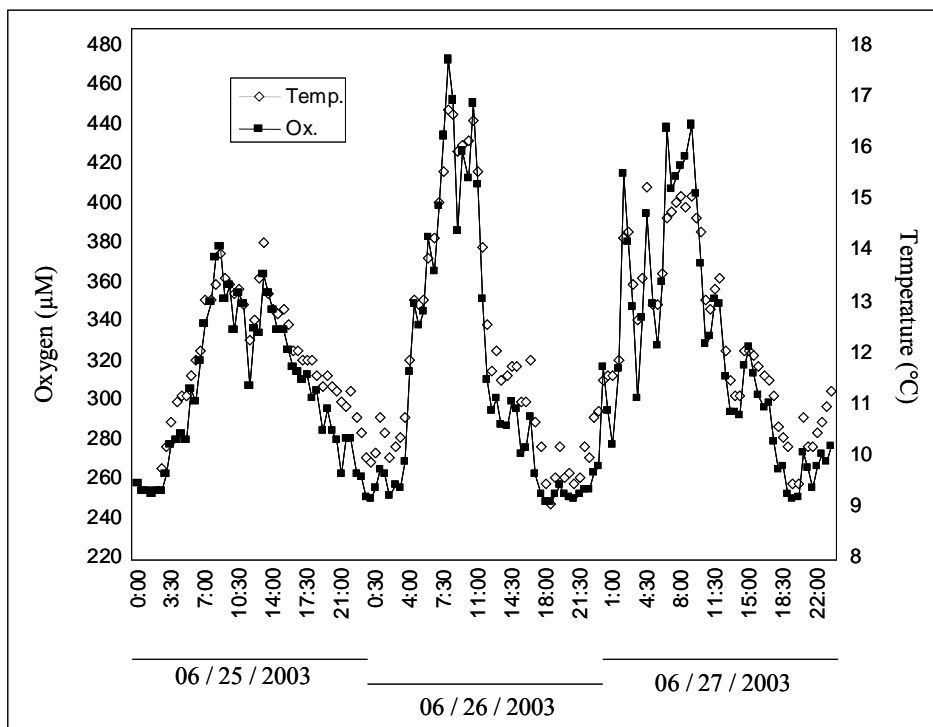
Fig. 9. Variations in the temperature (°C) and the oxygen concentration (µM) at 13 m depth in the Lac du Bourget from 25 to 27 June 2003. This figure demonstrates the presence of internal waves which might explain differences in the position of the metalimnic layer between distinct sampling points on the same day of sampling.
