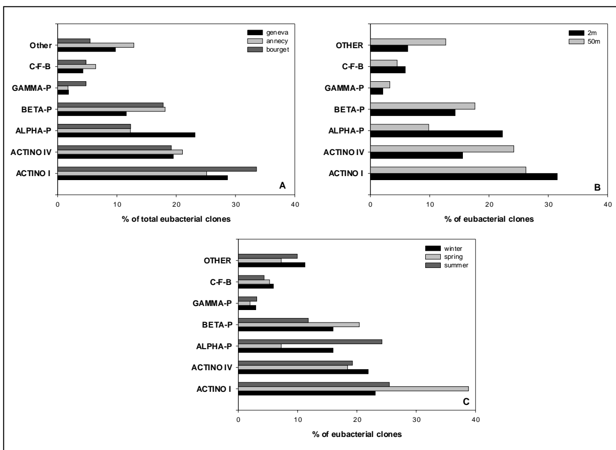
Fig 1. Relative proportions of sequences belonging to Actinobacteria groups I (ACTINO I) and IV (ACTINO IV) Alpha , Beta and Gammaproteobacteria (ALPHA-, BETA- and GAMMA-P), Bacteroidetes (C-F-B) and “other” for the lake (A), the depth (B) or the season (C).
