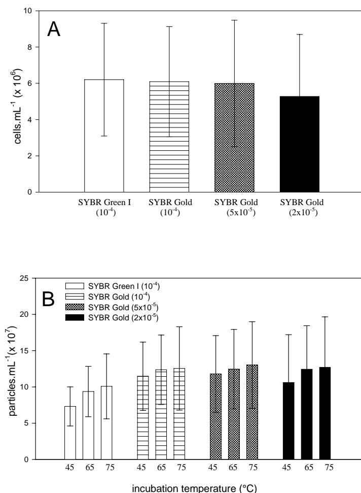
Fig. 2. FCM counts of heterotrophic bacteria (A) or viruses (B) stained with SYBR Green I ( 10^{-4} , white bars) or SYBR Gold at 3 different concentrations ( 10^{-4} , hatched bars; 5 \times 10^{-5} , dotted bars; 2 \times 10^{-5} , black bars) for 12 different samples. Viruses were incubated with each dye and concentration tested at 3 different incubation temperatures ( 45^{\circ}\text{C} , 65^{\circ}\text{C} and 75^{\circ}\text{C} ). Error bars are relative to 12 different water samples. Experiment 4.
