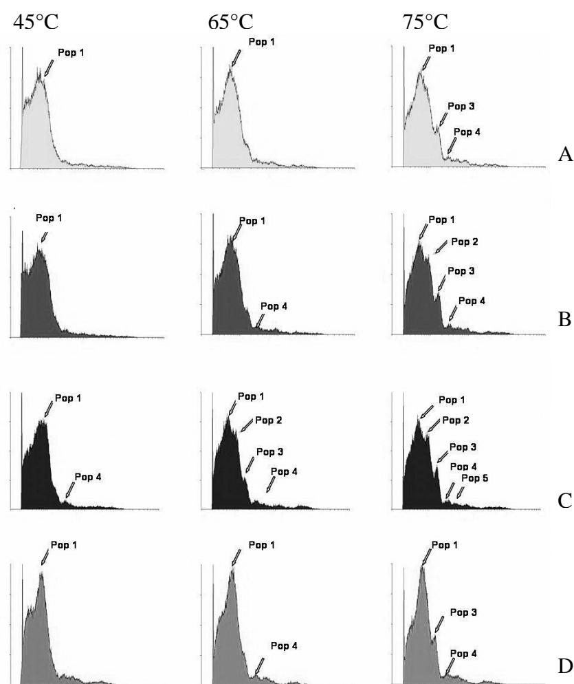
Fig. 3. Histograms of virus distributions showing different populations or groups (Pop). Samples were stained with SYBR Gold at a final concentration of 10^{-4} (A), 5 \times 10^{-5} (B) or 2 \times 10^{-5} (C) or with SYBR Green I at a final concentration of 10^{-4} (D), and incubated at different temperatures (45°C, 65°C or 75°C) for 10 minutes. Experiment 4.
