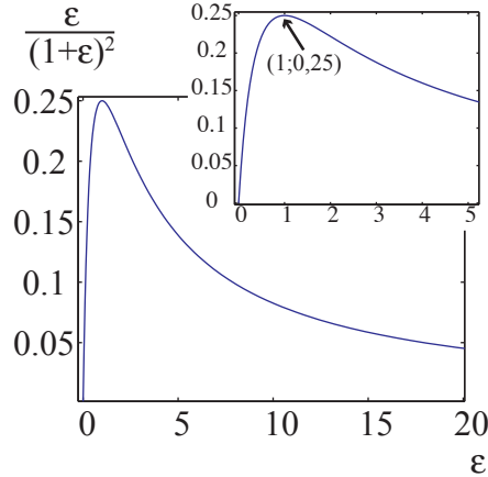
FIG. III.2.6 – f(\varepsilon) = \varepsilon/(1 + \varepsilon)^2
