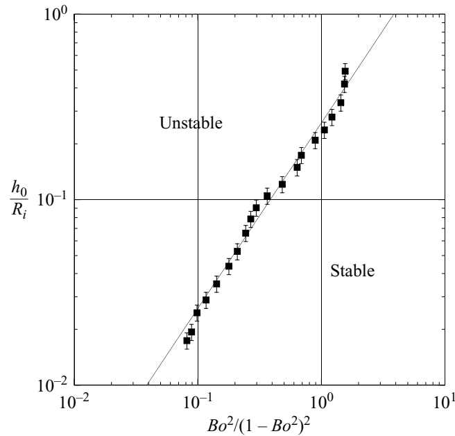
FIGURE 8. Transition between stable and unstable interfaces in the plane [h_0/R_i; Bo^2/(1 - Bo^2)^2] : \blacksquare , experimental data. The continuous line is the best linear fit: h_0/R_i = 0.26Bo^2/(1 - Bo^2)^2 .
