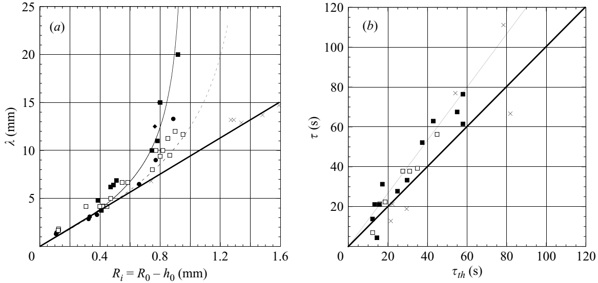
FIGURE 5. (a) Evolution of the wavelength \lambda as a function of the interface radius R_i for different liquids: \square , V100; \blacksquare , V1000; \circ , V12500; \bullet , glycerol; \times , experiments by Goldsmith & Mason (1963). The thick continuous line is the classical result \lambda = 2\pi\sqrt{2}R_i , the thin continuous line and the dashed line respectively represent the curves \lambda = 2\pi\sqrt{2}R_i/\sqrt{1-2.5Bo^2} for the silicone oils and the glycerol. (b) Comparison between the measured characteristic time \tau and the theoretical expression \tau_{th} \equiv 12\mu R_i^4/(\sigma h_0^3) for different liquids: \square V100, \blacksquare V1000, \times Experiments by Goldsmith & Mason (1963). The thick continuous line stands for the theoretical value and the thin continuous line for the best fit.
