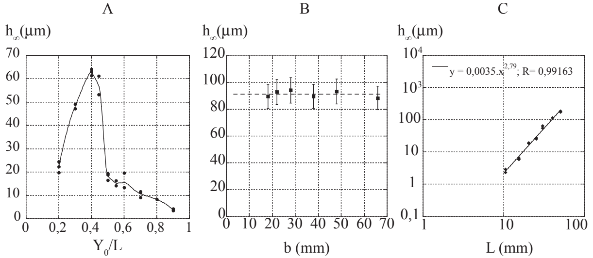
FIG. II.3.2 – A/ Effet de Y_0/L sur h_\infty (huile silicone V100; U = 28,8 mm/s; b = 38 mm; L = 28,5 mm; e = 180 \mu\text{m} ; \Omega = 800 \mu\text{L} ). B/ Effet de b sur h_\infty (huile silicone V100; U = 28,8 mm/s; L = 35,5 mm; Y_0/L = 0,42 ; e = 100 \mu\text{m} ; \Omega = 800 \mu\text{L} ). C/ Effet de L sur h_\infty (huile silicone V100; U = 28,8 mm/s; b = 38 mm; L = 35,5 mm; Y_0/L = 0,42 ; e = 100 \mu\text{m} ; \Omega = 800 \mu\text{L} ).
