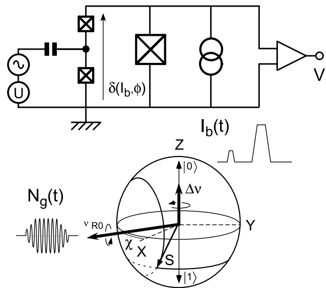
FIG. 1. Top: quantronium circuit. The Hamiltonian is controlled by the gate charge N_g applied to the island between the two small junctions, and by the phase \delta across their series combination. This phase is determined by the flux \phi through the loop, and by the bias current I_b . The two lowest energy states form a two-level system suitable for a qubit. The readout is performed by inducing the switching of the larger readout junction to a finite voltage V with a bias-current pulse I_b(t) approaching the critical current of this junction. Bottom: The quantum state is manipulated by applying resonant microwave pulses (phase \chi ) on the gate, or adiabatic pulses on the bias current. These pulses induce a rotation of the effective spin \vec{S} representing the qubit state on the Bloch sphere in the rotating frame. The Rabi precession of \vec{S} during a microwave pulse results in oscillations of the switching probability p with the pulse length \tau .
