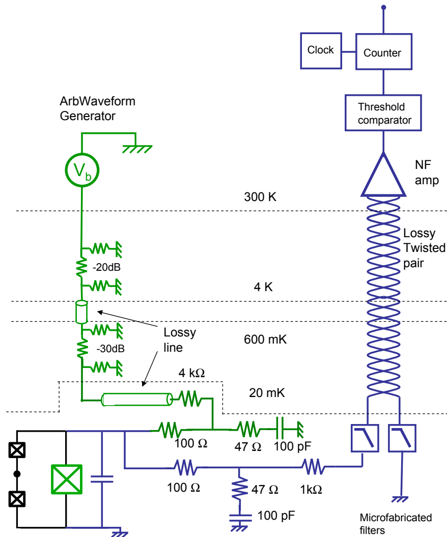
Figure 2.13: Experimental setup of the readout. Left: current biasing line. Right: measuring line. The two RC = 47\ \Omega/100\text{pF} shunts the measuring and biasing lines above 100\text{MHz} , which protects the qubit from any spurious resonance in these lines and sets the quality factor of the readout junction to Q \approx 3 . Since the measuring line is not attenuated contrary to the biasing one, this line needs an extremely strong filtering in the microwave frequency range, in order to avoid any thermal photons exciting the qubit or the readout junction. This filtering is provided by microfabricated distributed RC filters, having more than 110\text{dB} attenuation above 100\text{ MHz} .
