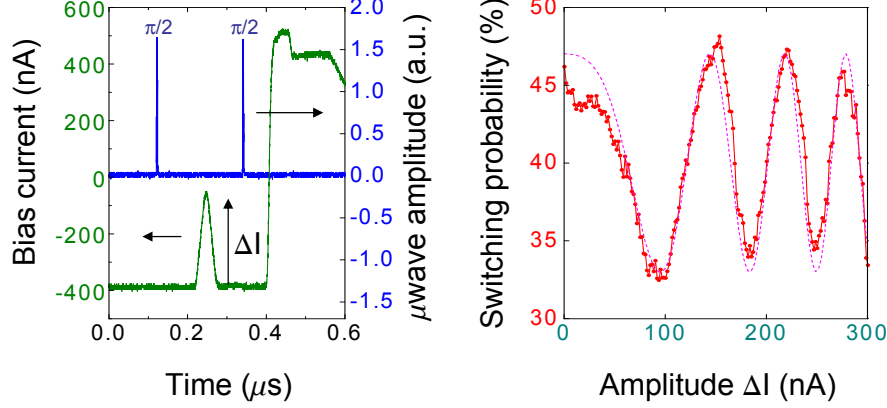
Figure 3.8: Rotation around the Z axis with a detuning pulse. Left: a current pulse changes adiabatically the transition frequency during a Ramsey sequence. Top: during triangular adiabatic current pulse, the working point is moved away from (\delta = 0, N_g = 1/2) in the phase direction and put back. Right: The switching probability oscillates with the amplitude of the current detuning pulse which renders the rotation of the qubit around the Z axis. The experimental curve is fitted (dashed line) by taking into account the parabolic dependance of \nu_{01} with \delta . The maximum contrast of the signal has been optimized and is lower than during a Rabi. We attribute this discrepancy to errors on the microwave pulses durations.
