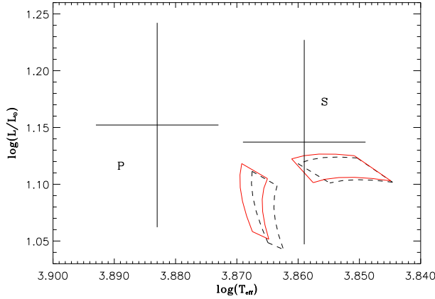
Fig. 5. Error boxes calculated by decreasing the rate of the ^{12}\text{C}(p,\gamma)^{13}\text{N}(e^+, \nu)^{13}\text{C} reaction of 10% (full line) from the NACRE rate (dashed line)
