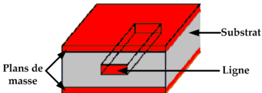
Fig. II-7: configuration "triplaques"
