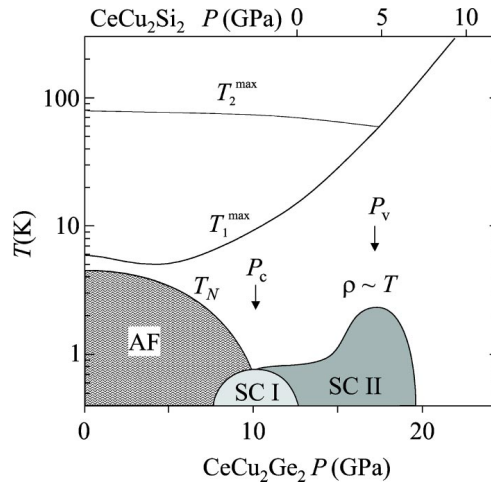
FIG. 7. Schematic P - T phase diagram for \text{CeCu}_2(\text{Si}/\text{Ge})_2 showing the two critical pressures P_c and P_v . At P_c , where the antiferromagnetic ordering temperature T_N \rightarrow 0 , superconductivity in region SC I is mediated by antiferromagnetic spin fluctuations; around P_v , in region SC II, valence fluctuations provide the pairing mechanism and the resistivity is linear in temperature. The temperatures T_1^{\max} and T_2^{\max} merge at a pressure coinciding with P_v .
