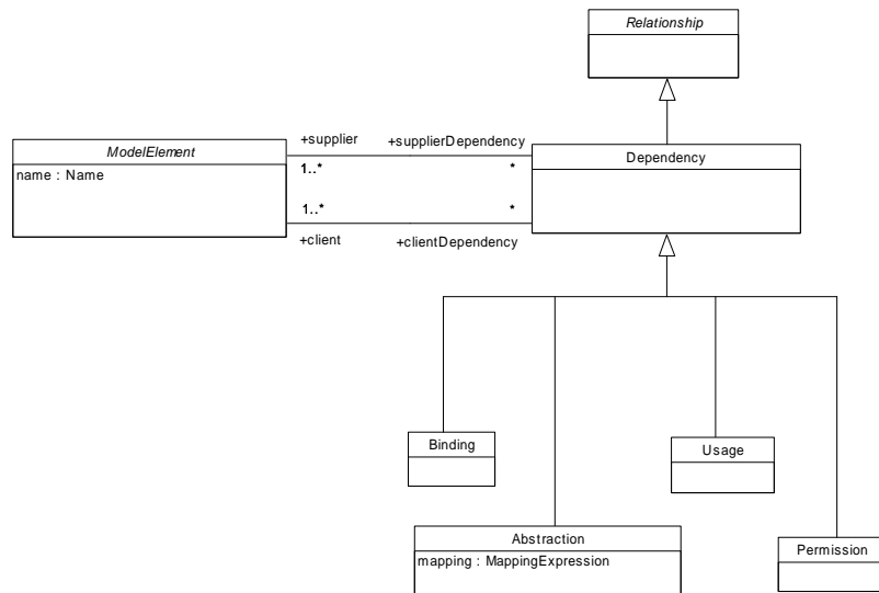
Figure 6.5. UML Core Package — Dependencies
