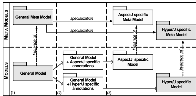
Figure 4.31. Processus de transformation
