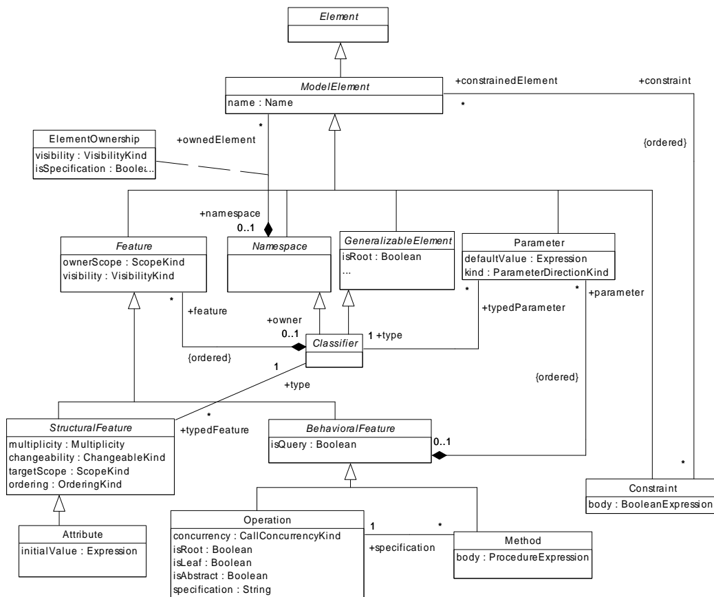
Figure 6.2. UML Core Package — Backbone
