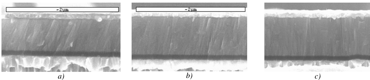
Figure 3.23 : SEM pictures of a typical c-axis inclined ZnO film (sample PIIj). a) 23^\circ inclined columns at a distance of 5 mm from the blind, b) 11^\circ inclination at 17mm and c) 0^\circ at the border of the wafer. A 100 nm thick top Pt electrode and a 100 nm \text{Al}_2\text{O}_3 buffer-layer below the ZnO can be seen.
