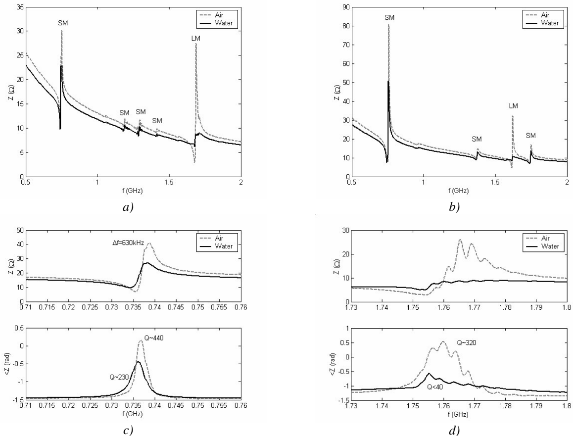
Figure 5.4 : Broadband impedance characteristics of samples SIIIa (a) and SIIIb (b) in air and pure water; and narrowband characteristics of the fundamental shear (c) and longitudinal (d) modes of SIIIa in air and water.
