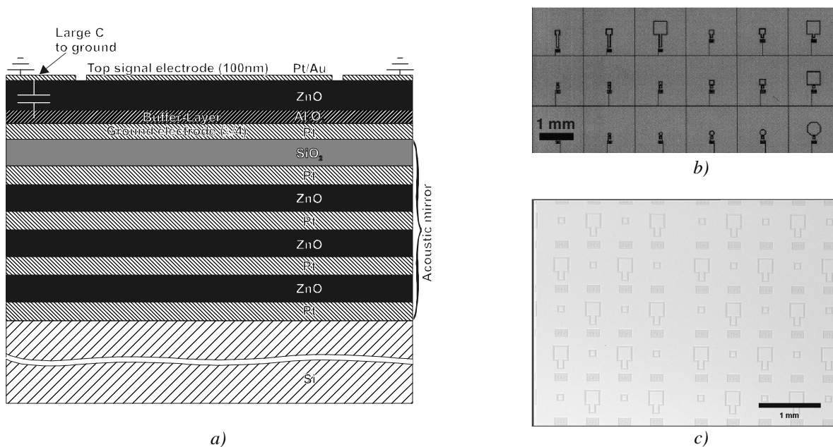
Figure 4.13 : a) Schematic cross-section of DESIGN 1 acoustic stack with a 4-fold Pt-ZnO mirror with top SiO 2 layer; b) classic mask picture and c) high density mask microscope view.
