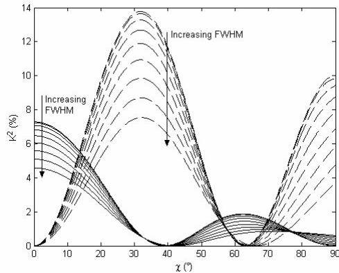
Figure 3.29 :Reduction of the coupling constant of shear (dashed) and longitudinal (solid) modes due to spread of the inclination in \chi direction for different FWHMs: ideal case ( 0^\circ ), 5^\circ , 10^\circ , 15^\circ , 20^\circ , 25^\circ , 30^\circ , 35^\circ , and 40^\circ .
