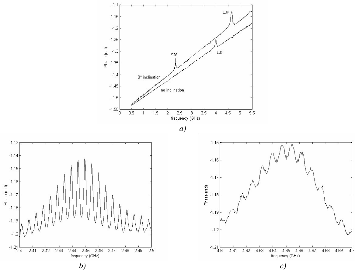
Figure 3.19 : a) Broad-band characteristic of the impedance phase for sample PI1b at a point of maximum inclination at around 4 mm from the electrode and at the border of the wafer, where no inclination has been recorded; and narrow-band characteristic for the shear mode (b) and longitudinal mode (c).
