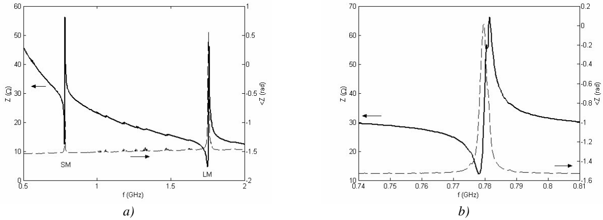
Figure 4.19 : Broadband (a) and narrowband (b) impedance characteristics of sample SIIE.
