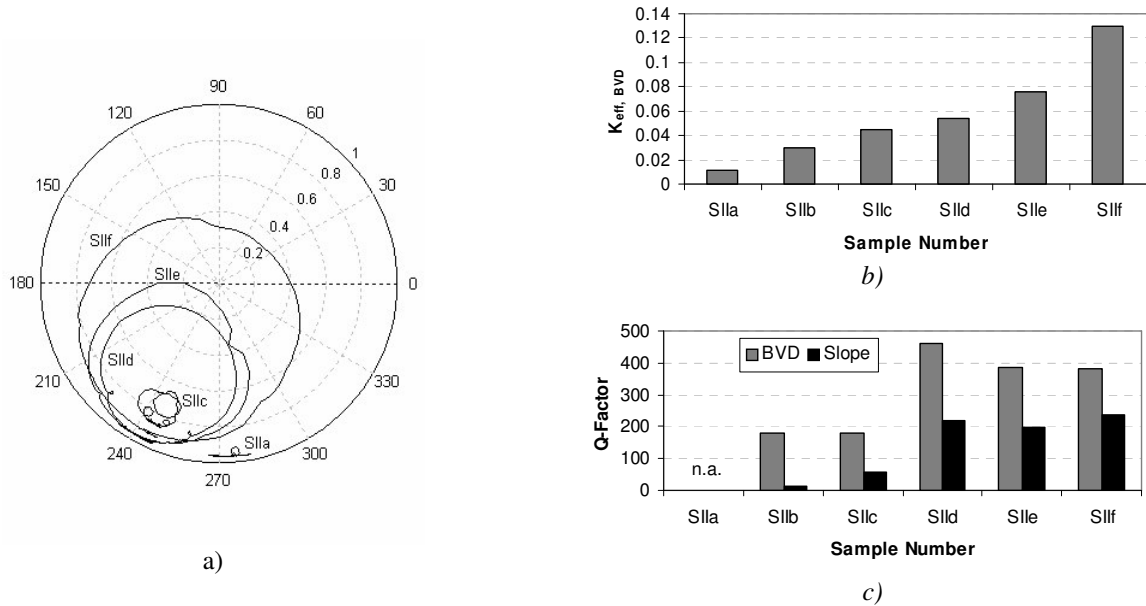
Figure 4.22 : a) Smith-chart representation of the impedances of samples SIIa to SIIf; b) evolution of the effective coupling coefficient and c) evolution of the Q -factors.
