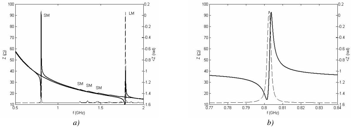
Figure 4.12 : Simulated impedance characteristic (a: broadband and b: narrow-band) of a typical solidly mounted FBAR on a 3-fold W-SiO 2 mirror with a total Q-factor of 500. The buffer-layer is 100 nm Al 2 O 3 .
