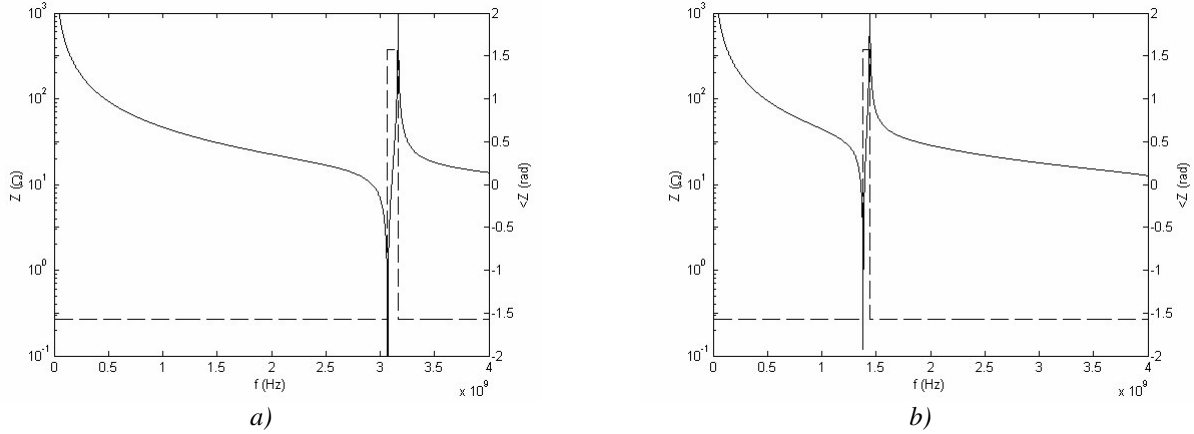
Figure 2.6 : Impedance characteristic (solid: amplitude, dashed: phase) of a simple FBAR of c-axis inclined ZnO. a) Pure longitudinal mode ( 0^\circ ), b) pure shear mode ( 90^\circ ). The area is 200\mu\text{m} \times 200\mu\text{m} and the thickness 1\mu\text{m} .
