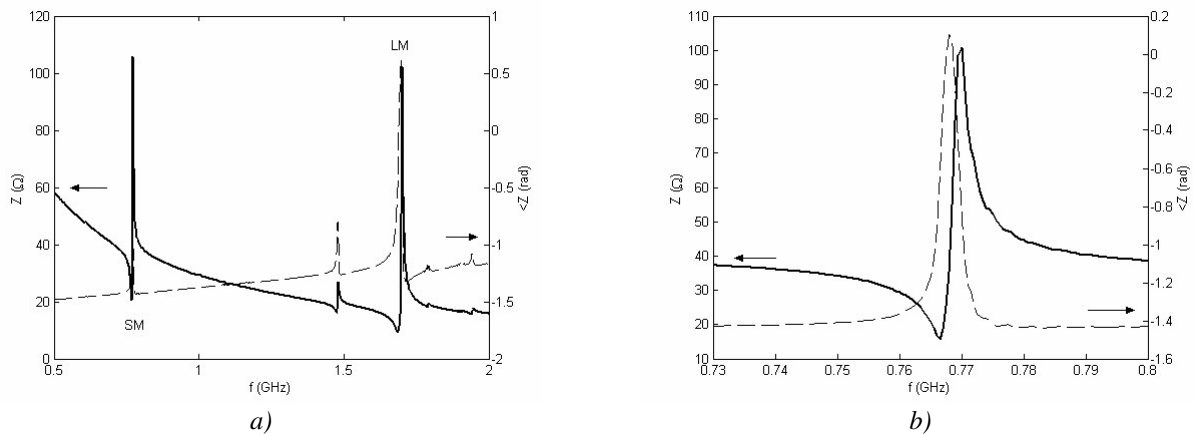
Figure 4.21 : Broadband (a) and narrowband (b) impedance characteristics of sample SII g .
