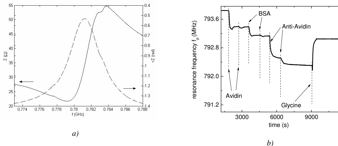
Figure 5.16 : a) Impedance characteristic in water of the resonator from sample SII used for the time-dependent biochemical measurement shown in b). (courtesy of Jan Weber)
