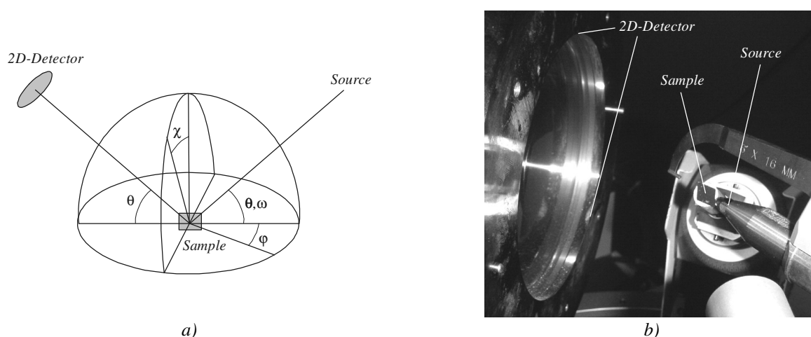
Figure 3.3 : A schematic illustration of the x-ray diffraction with \theta\varphi\chi geometry and a picture of the 2D-detector, sample-holder with sample and source of the XRD equipment used in this work.
