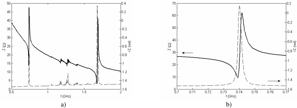
Figure 4.25 : Broadband (a) and narrowband (b) impedance characteristics of sample SIIIa.
