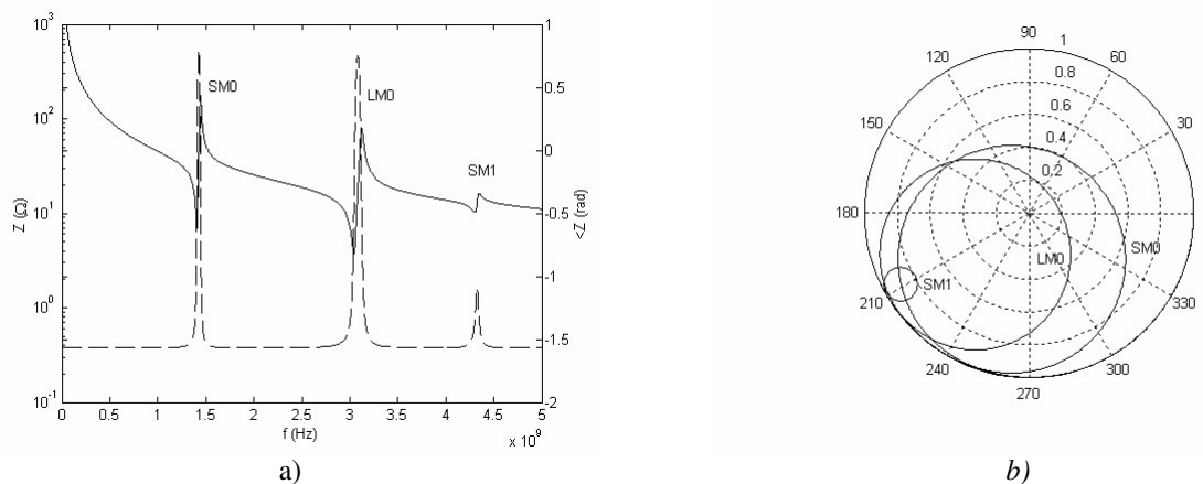
Figure 2.19 : a) Wide-band impedance characteristic (solid: amplitude, dashed: phase) and b) Smith-Chart of a simple ZnO FBAR of 13.6^\circ c -axis inclination, with a Q of 100. The area is 200 \mu\text{m} \times 200 \mu\text{m} and the thickness is 1 \mu\text{m} .
