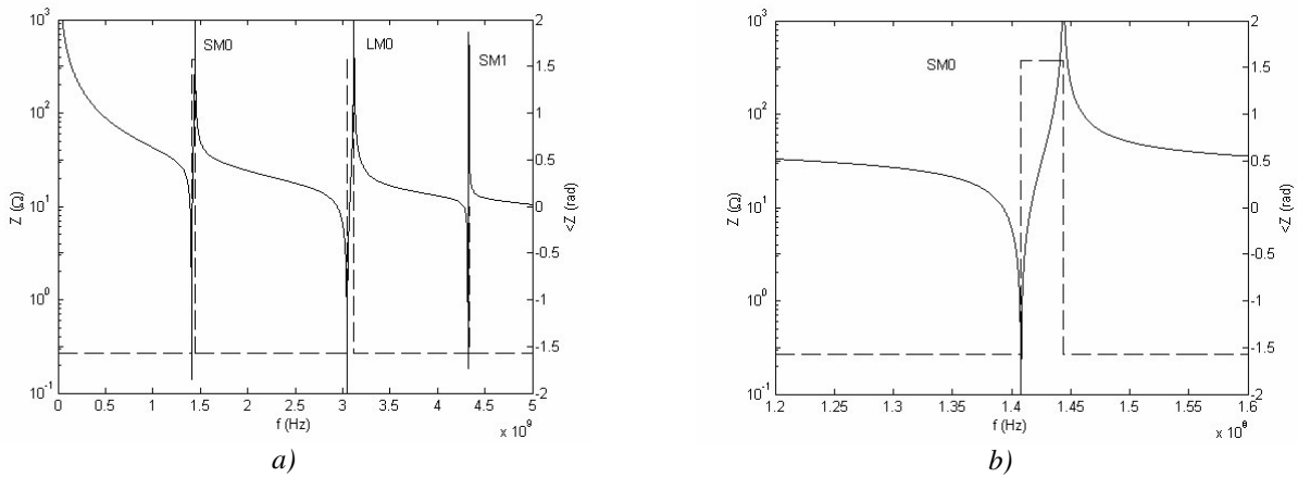
Figure 2.7 : Impedance characteristic (solid: amplitude, dashed: phase) of a simple FBAR of 13.6^\circ c-axis inclined ZnO. a) Wide-band, b) Narrow-band. The area is 200\mu\text{m} \times 200\mu\text{m} and the thickness is 1\mu\text{m} .
