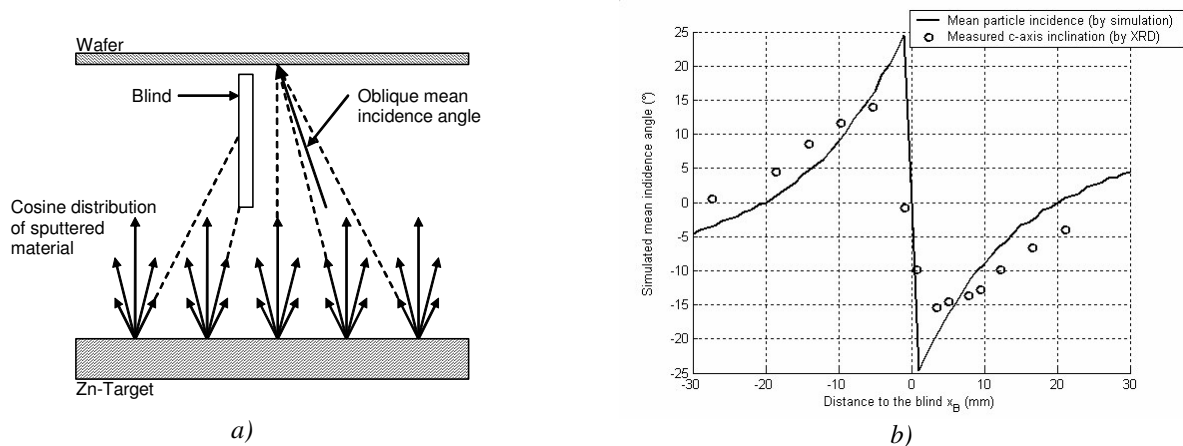
Figure 3.26 : a) Simple geometric explanation for the inclined ZnO films growth: oblique mean particle incidence results due to a blocking effect by the blind; b) Result of geometric simulations for a 15 mm blind compared to ZnO thin film inclinations obtained from XRD measurements for sample PIIk.
