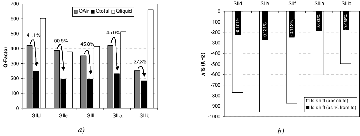
Figure 5.6 : Average change of SMR Q-factors (a) and resonance frequency (b) in water for resonators of different samples. Q_{Total} is the Q-factor in water; Q_{Air} and Q_{Liquid} are the Q-factor contributions from the losses in air and to the liquid respectively.
