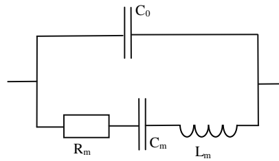
Figure 2.16 : Butterworth-Van Dyke model.
