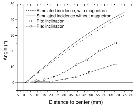
Figure 3.13 : Simulations and measurements of PROCESS I. The lines show the simulations for sputtering with (dashed) and without (solid) magnetron. The points show the measured points for samples P1b (squares) and P1e (circles).
