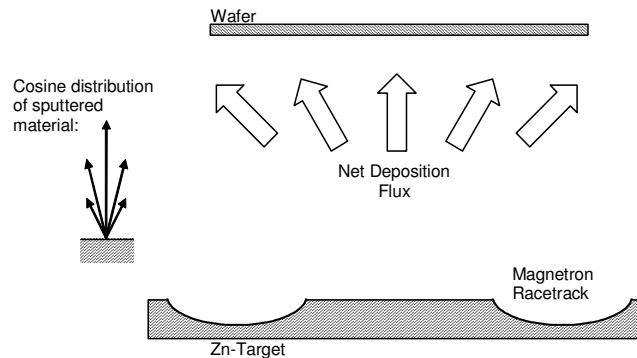
Figure 3.11 : Schematic of the substrate and target showing the direction of the net deposition flux of sputtered particles for low pressure processes. The inclination of the flux on the border of the substrate is due to the magnetron racetrack and the cosine distribution of sputtered material.
