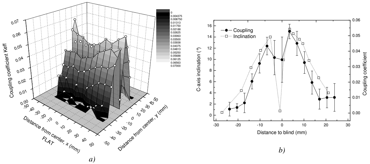
Figure 4.23 : a) 3D representation of the effective coupling coefficient distribution of sample SIIId over the 4" wafer surface; b) average values and standard deviations of this distribution along the projection on the x-axis perpendicular to the blind compared with the recorded c-axis inclinations.
