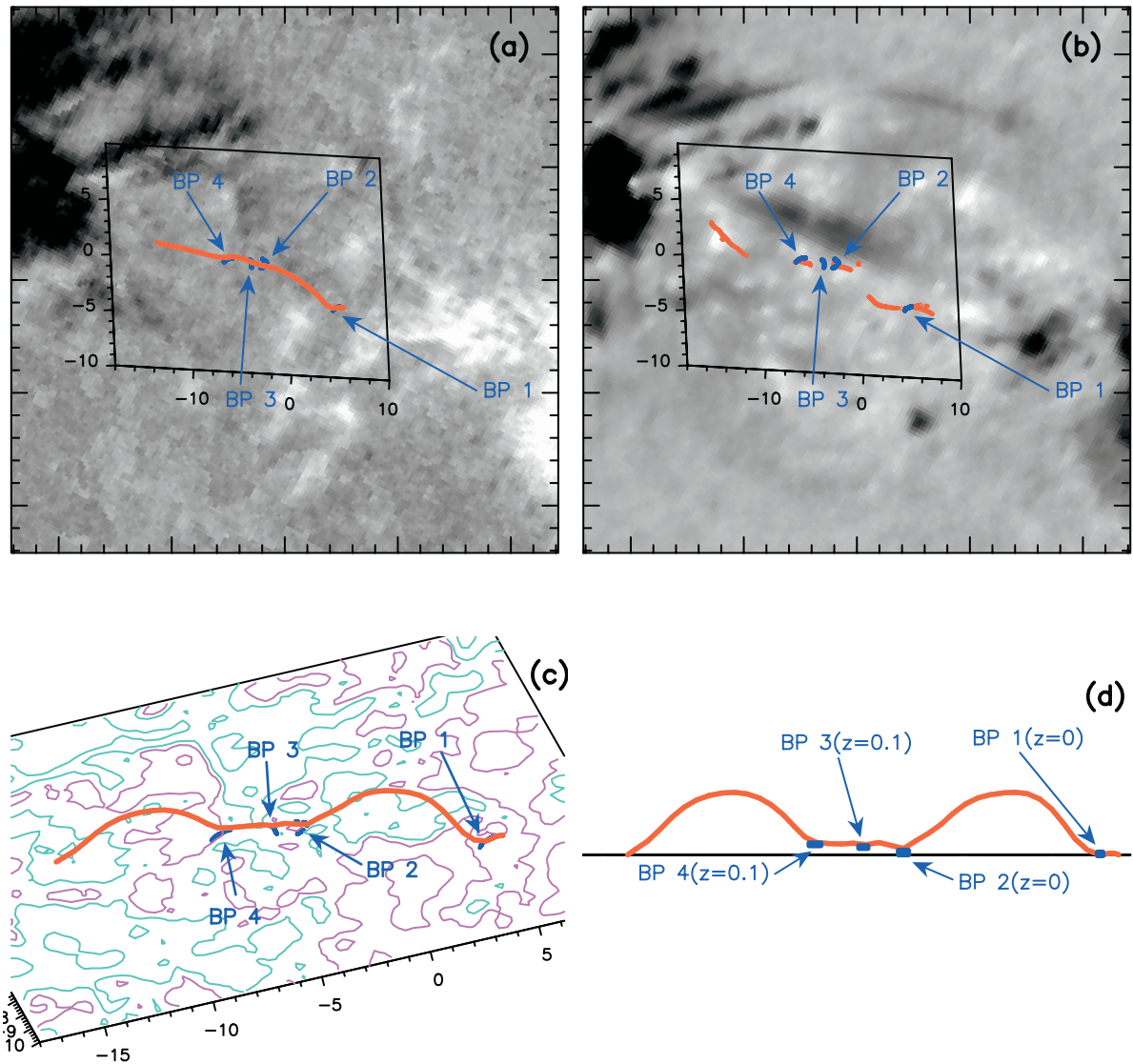
FIG. 5.—First example of an undulatory flux tube: only one field line of the serpentine flux tube ( red line ) is represented on these figures. The blue dots (denoted BP 1–BP 4) represent the BPs and dips through which the serpentine line is passing. (a) Position of the undulatory field line on the vertical magnetogram. (b) Positions of the footpoints of the serpentine line ( red dots ) on the H\alpha 0.8 Å filtergram. In (c) and (d), a multiplicative factor of 3 for vertical extension of the field line is used for a better viewing of the configuration. (c) Projection view of the undulatory flux. On the base plane, the isocontours represent B_z(z=0) = \pm 50, 300, 900, and 1800 G, pink for positive and blue for negative values. The base plane boundaries are represented in (a) and (b). (d) Side view of the undulatory field line. The height of the BPs and dips are indicated in Mm.
