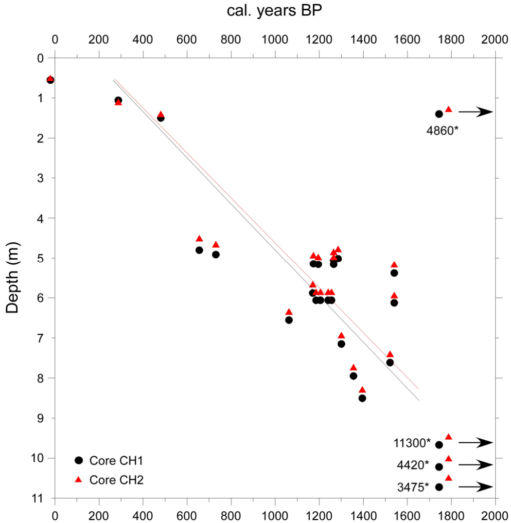
Figure 2.8: Age-depth plot for Cores CH1 (black circles) and CH2/1 (red triangles). 14 C values marked with * indicate reworked material older than 2000 yr BP.
