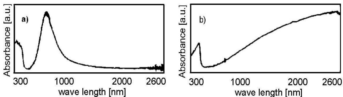
Fig. II.7.3 UV-Vis-NIR spectra of PANI/(CSA) 0.5 films cast from: a) chloroform, b) m -cresol [66]
