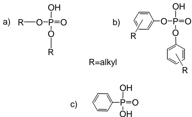
Fig.II.7.2 Diesters of phosphoric acid (a,b) and phenylphosphonic acid (c) used for the acid-base doping of PANI
