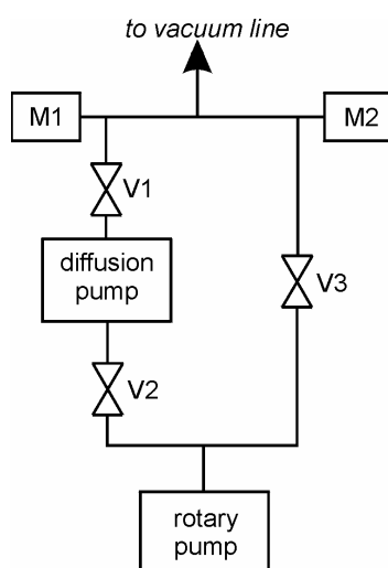
Fig.III.1.1 Scheme of pumping unit were M1, M2 – gauges; V1, V2, V3 – electropneumatic valves
