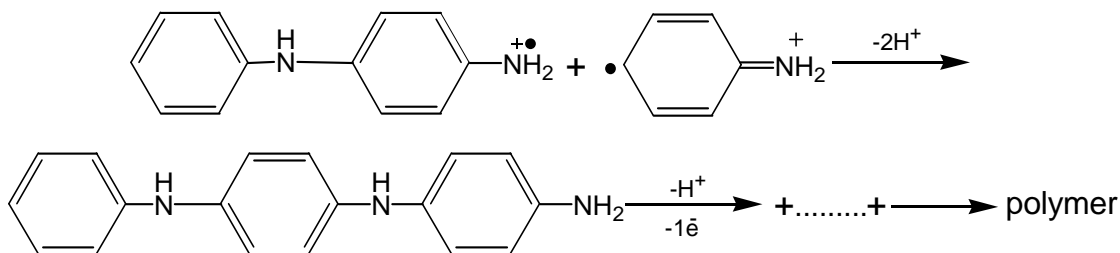
Fig. II.3.4 Propagation of the polyaniline chain
