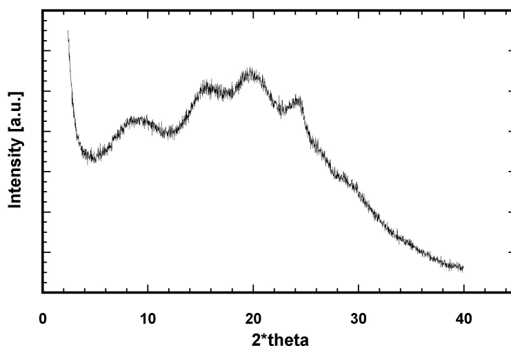
Fig. IV.1.1 Diffraction pattern of emeraldine base
