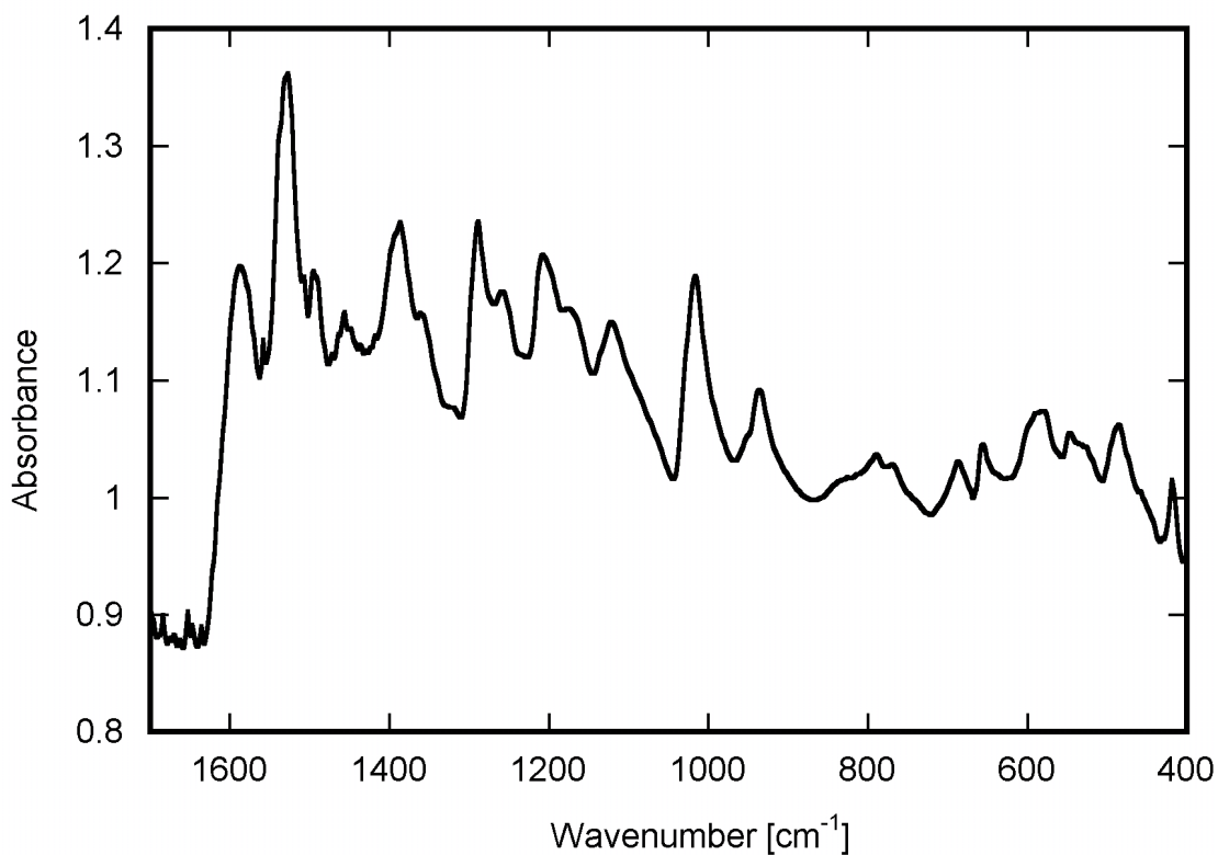
Fig. IV.6.5 IR spectrum ( 400 \text{ cm}^{-1} - 1700 \text{ cm}^{-1} ) of polyanisidine doped with \text{AlCl}_2(\text{acac}) in nitromethane
