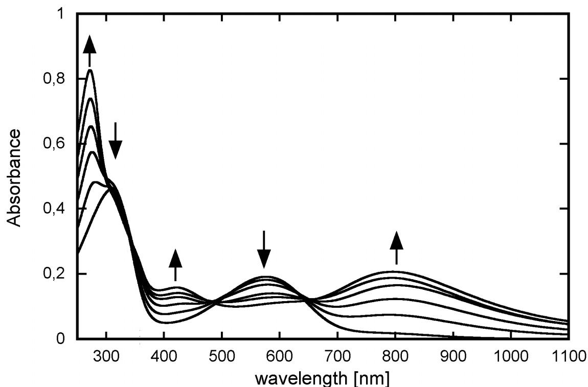
Fig. IV.4.2 UV-Vis-NIR spectra registered during addition of \text{FeCl}(\text{acac})_2 to poly(2-ethylaniline) solution. Arrows show changes of intensity of the particular peaks when concentration of \text{FeCl}(\text{acac})_2 increases. Chloroform was used as a solvent.
