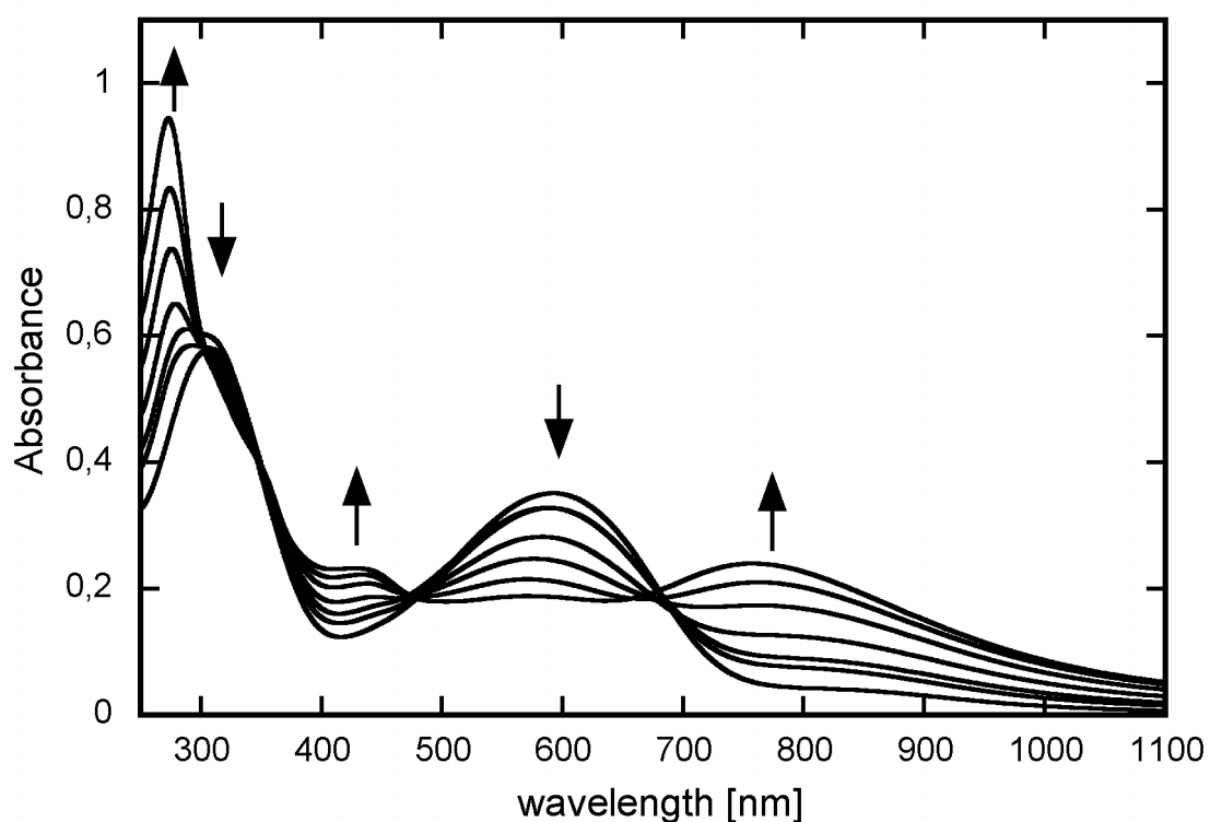
Fig. IV.4.1 UV-Vis-NIR spectra registered during addition of FeCl(acac)_2 to polyaniline solutions. Arrows show changes of intensity of the particular peaks when concentration of FeCl(acac)_2 increases. Chloroform was used as a solvent.
