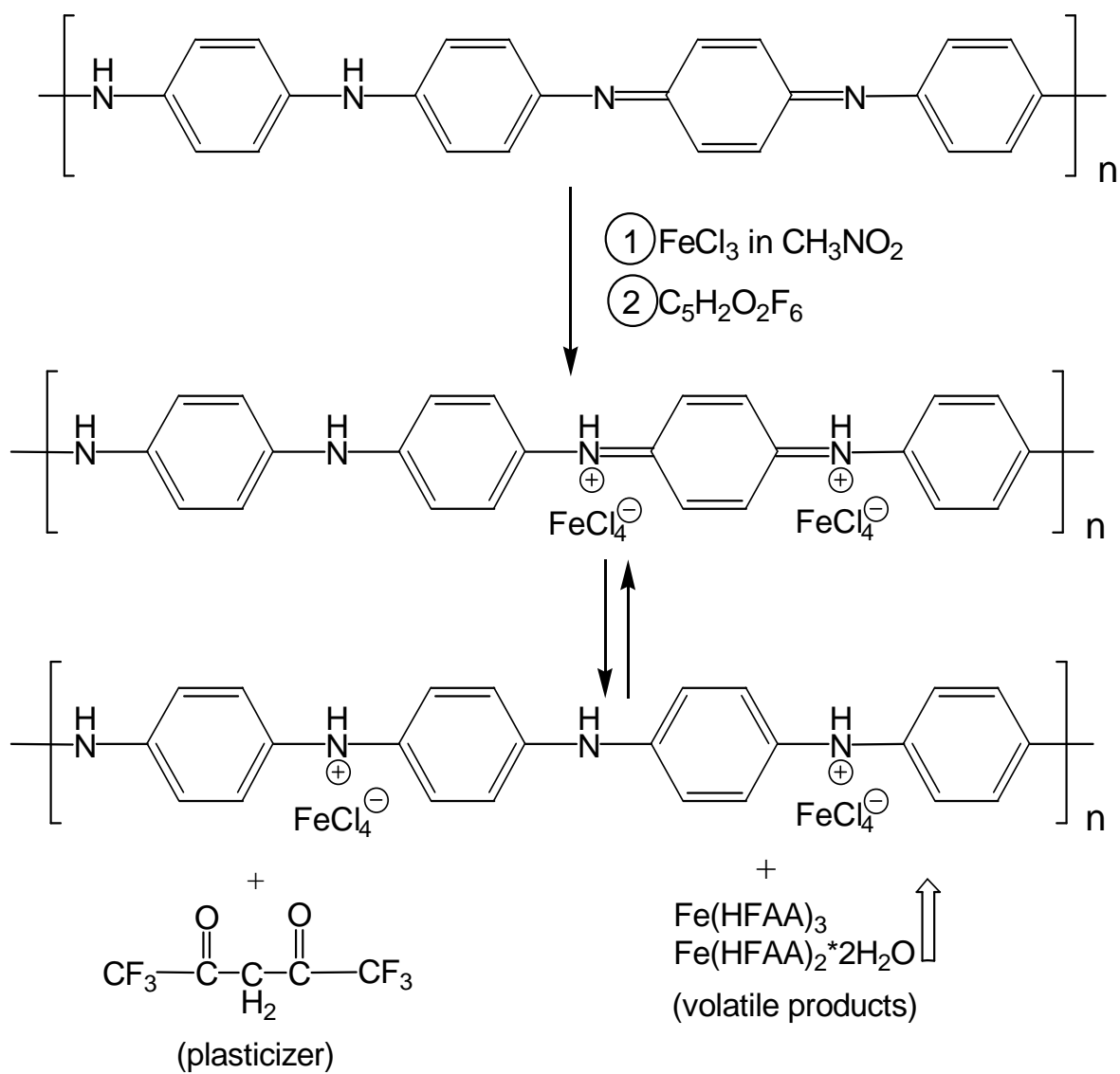
Fig.IV.3.5 Schematic representation of the reaction of emeraldine base with \text{FeCl}_3 and hexafluoroacetylacetone (HFAA) in nitromethane.
