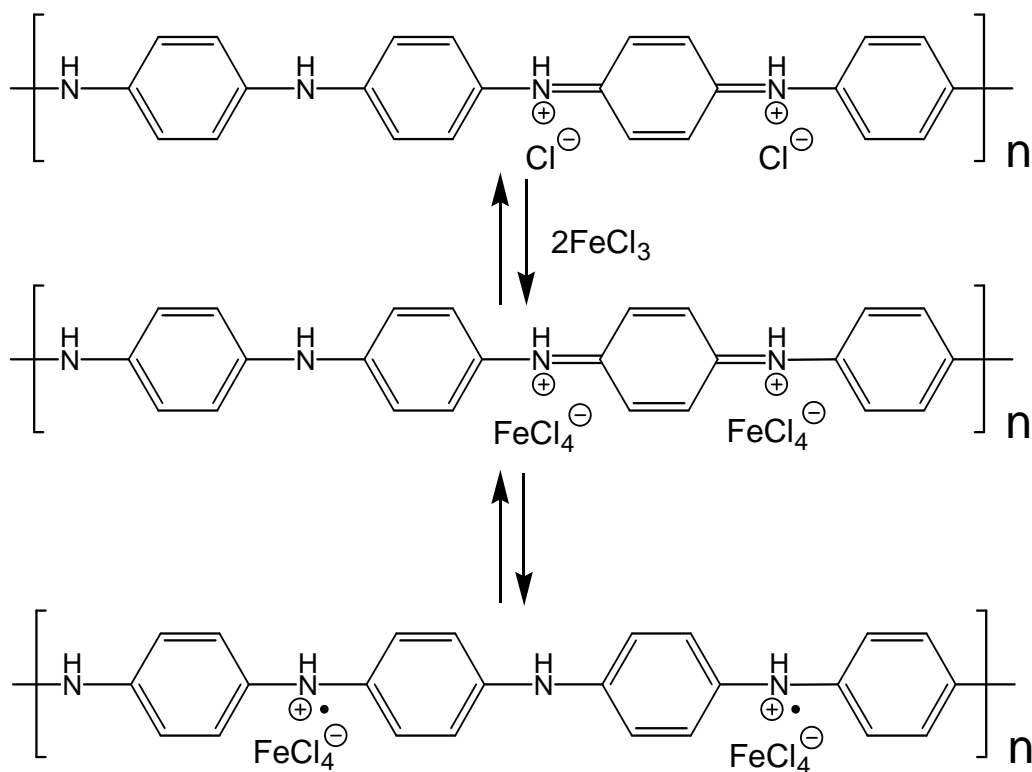
Fig. IV.2.6 Schematic representation of the reaction between \text{FeCl}_3 and polyaniline hydrochloride
