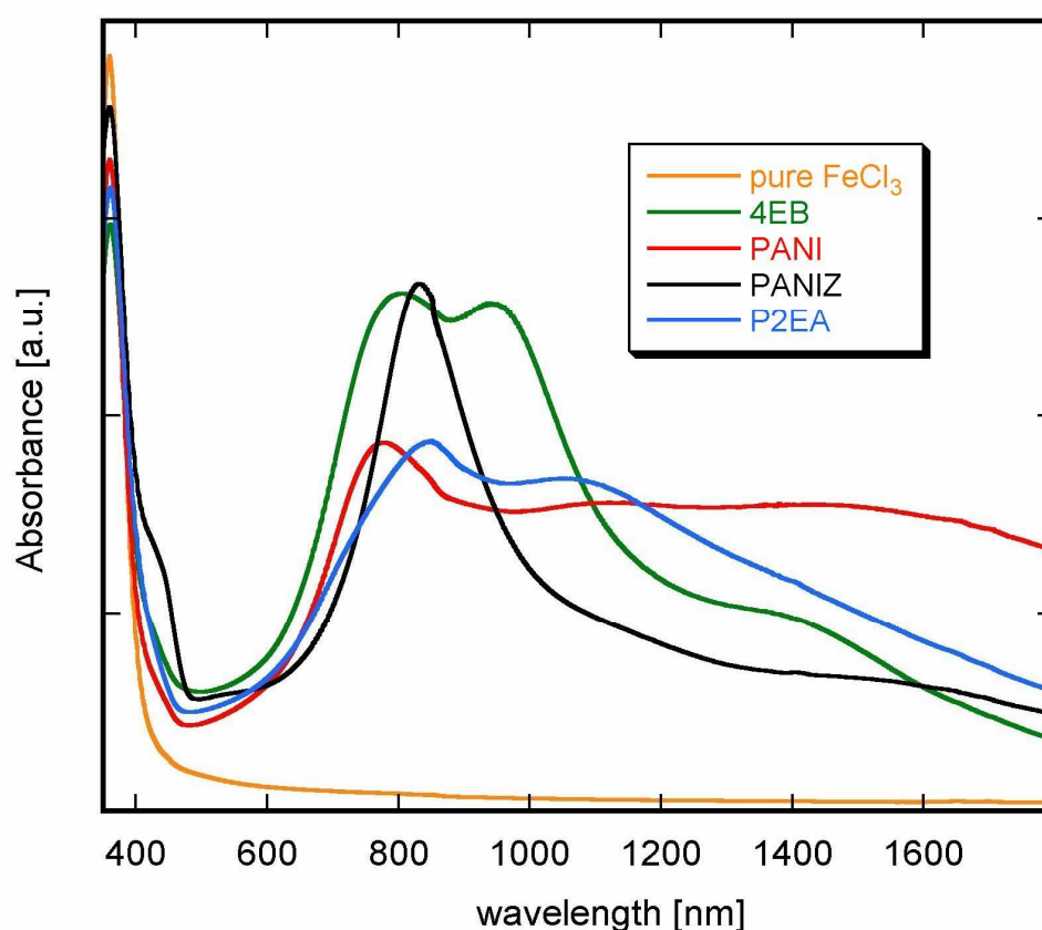
Fig. IV.2.2 UV-Vis-NIR spectra of the nitromethane solutions of pure \text{FeCl}_3 , polyaniline, polyanisidine, poly(2-ethyl)aniline and tetramer of aniline doped with \text{FeCl}_3 , ratio (1:1)
