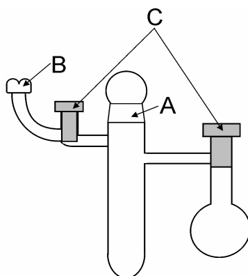
Fig. III.1.3 Vacuum reactor: A – joint, B - spherical joint, C - Rotaflo stopcocks
