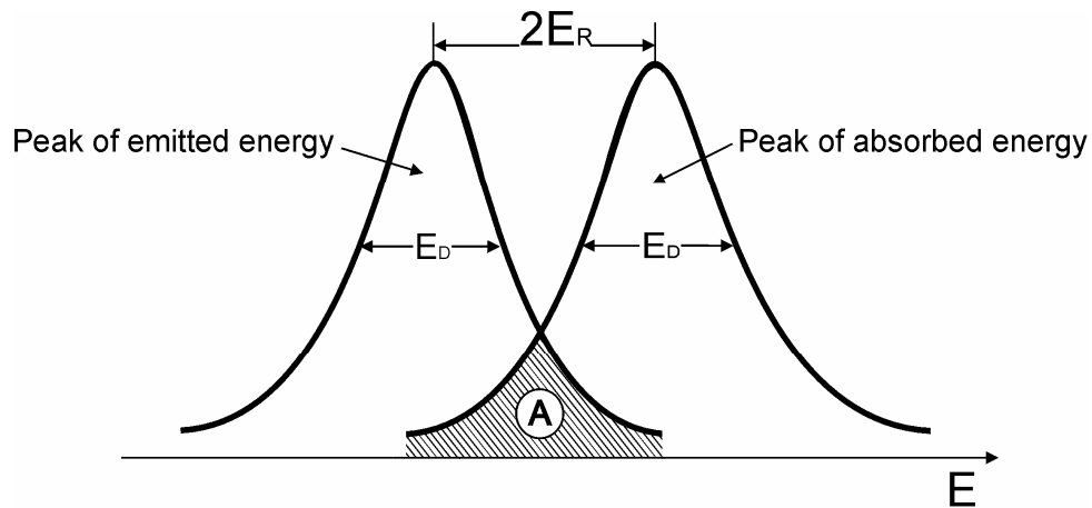
Fig. VI.1.2 Gamma photon absorption and emission energy distributions for free nucleus when recoil effect is observed. A – resonance area
