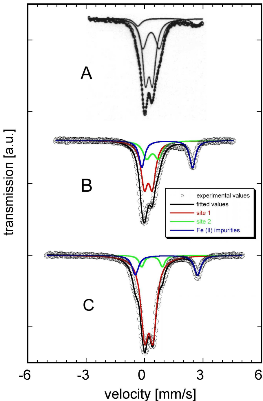
Fig. IV.2.5 Mössbauer spectra of complexes measured at 77K of following compounds doped with FeCl_3 ; mer to dopant ratio (1:1) A) polyaniline, B) poly(2-ethylaniline), C) tetramer of aniline
