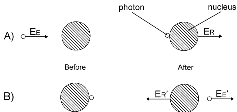
Fig. VI.1.1 Absorption (A) and emission (B) of \gamma photon having energy E_E , ( E_{E'} ) by a nucleus. E_R and ( E_{R'} ) are recoil energies.
