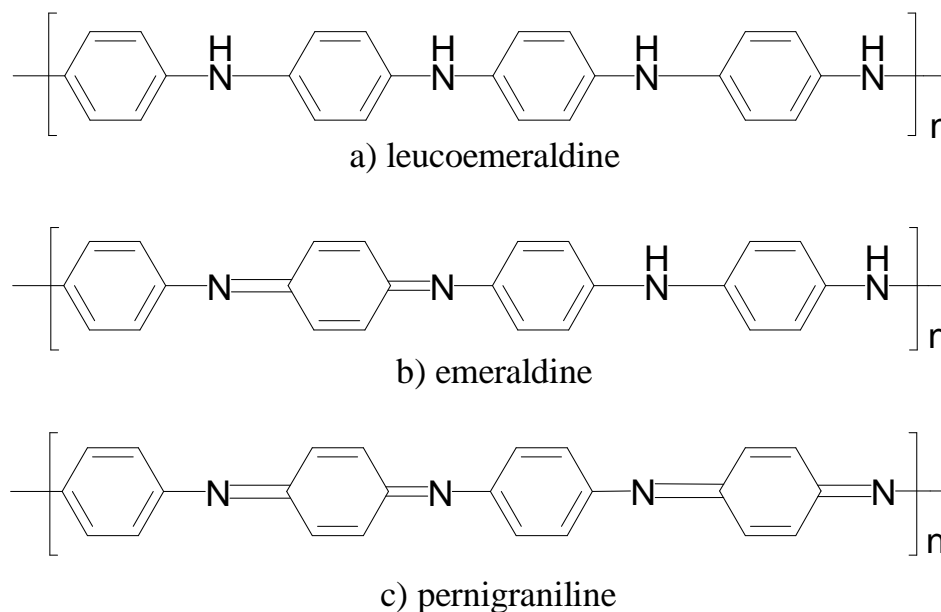
Fig. II.1.2 Principal forms of polyaniline base
