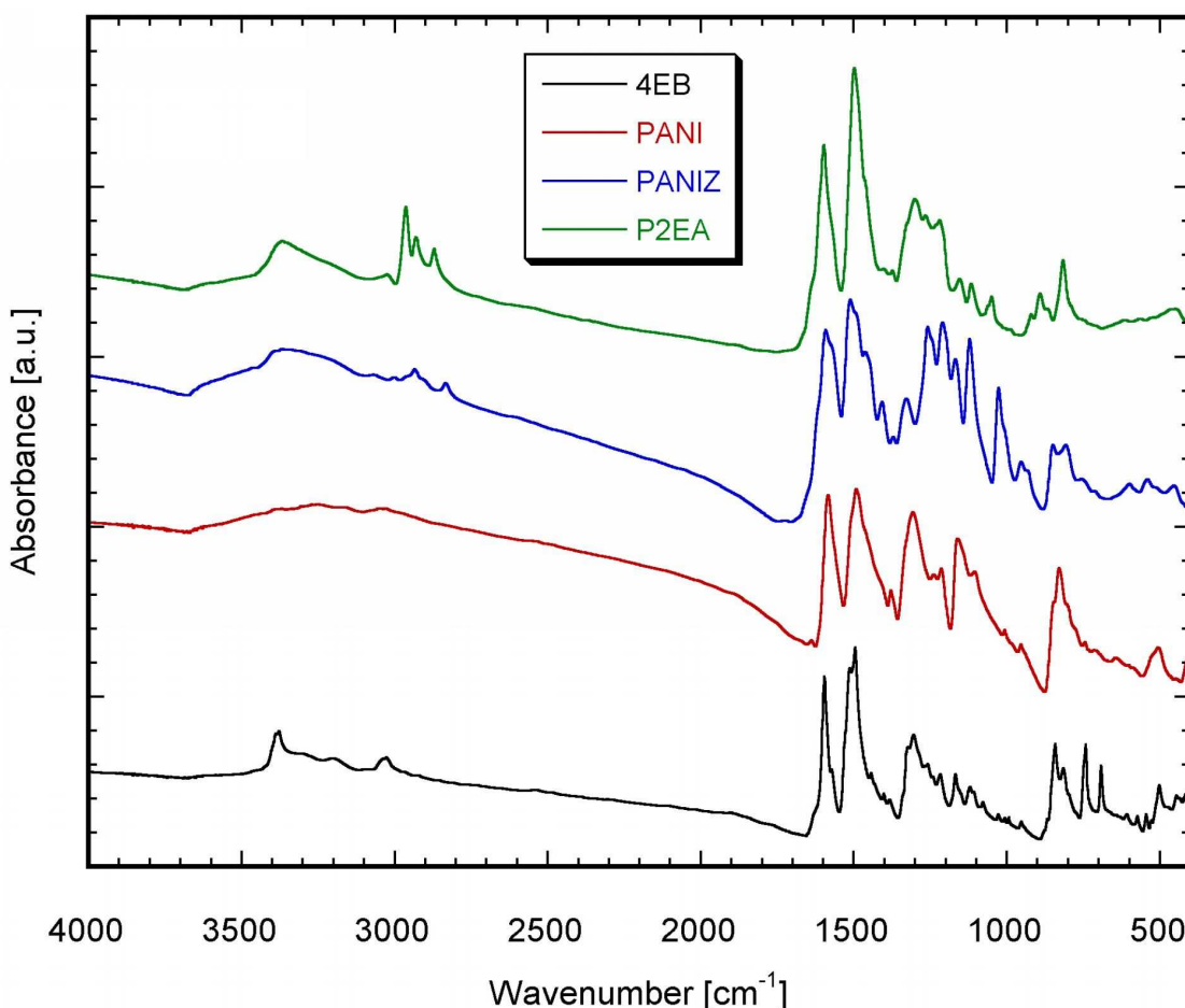
Fig. IV.1.5 IR spectra (4000 cm -1 - 400 cm -1 ) of polyaniline, polyanisidine, poly(2-ethylaniline) and the tetramer of aniline
