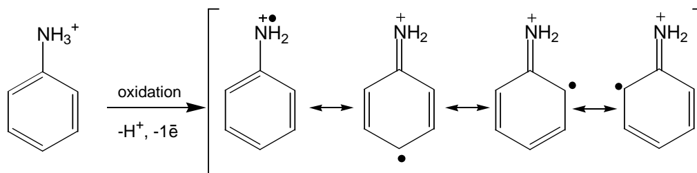
Fig. II.3.1 The formation of aniline radical cation
