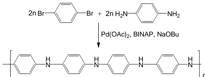
Fig. II.2.1 Synthesis of leucoemeraldine by polycondensation using 1,4-phenylenediamine and 1,4-dibromobenzene
