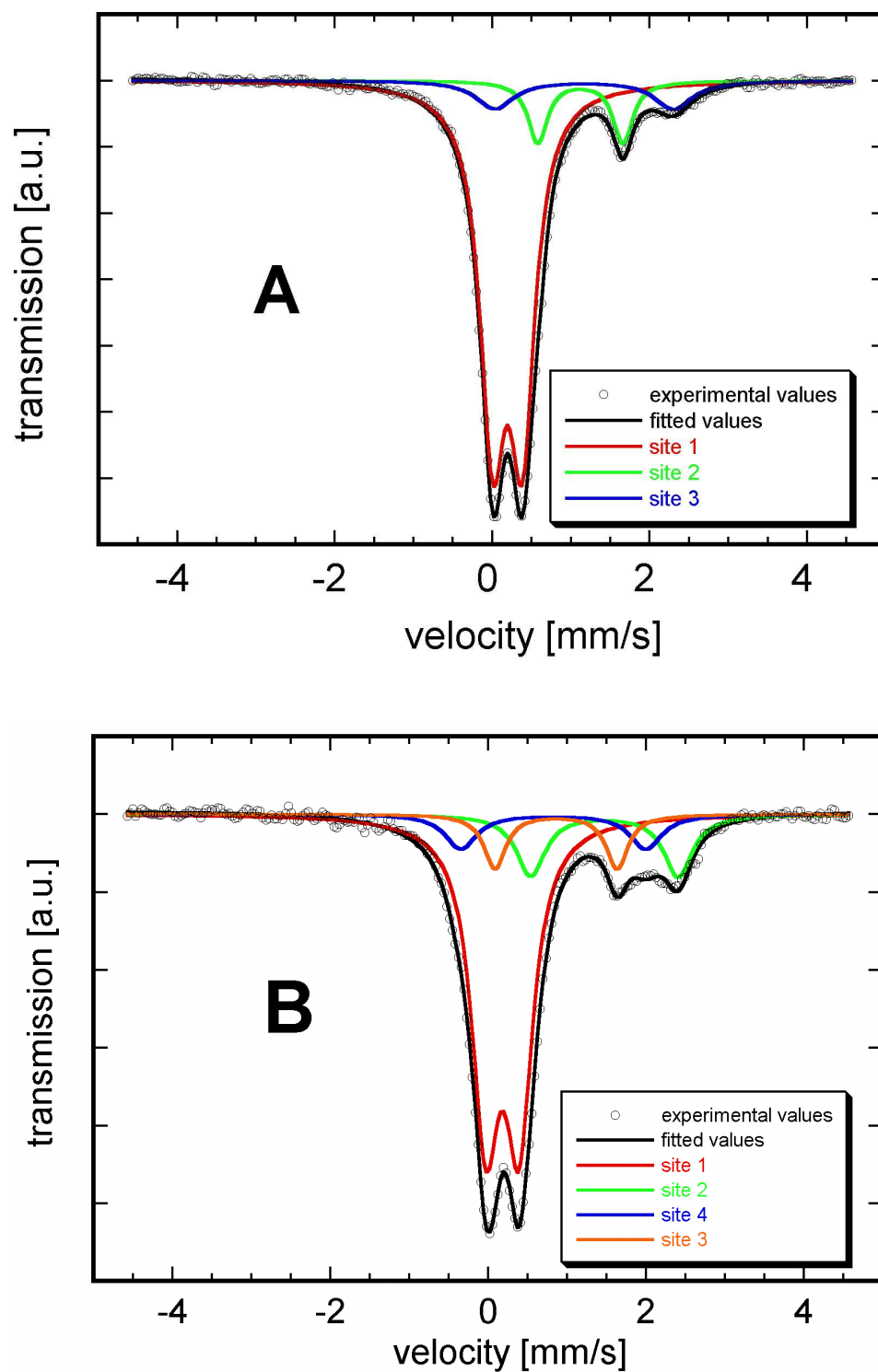
Fig. IV.3.8 Mössbauer spectra of A) polyanisidine, B) poly(2-ethylaniline), all compounds were treated with FeCl_3 and subsequently processed with triple excess of HFAA. Samples pumped for 40 hours, spectra registered at 77K.
