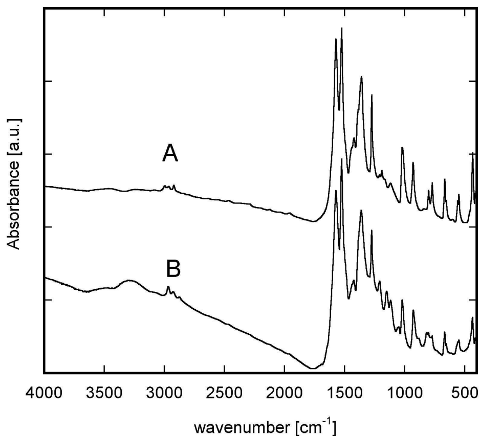
Fig. IV.4.5 Infrared spectra of polyanisidine (A) and poly(2-ethylaniline)(B) doped with FeCl(acac) 2
