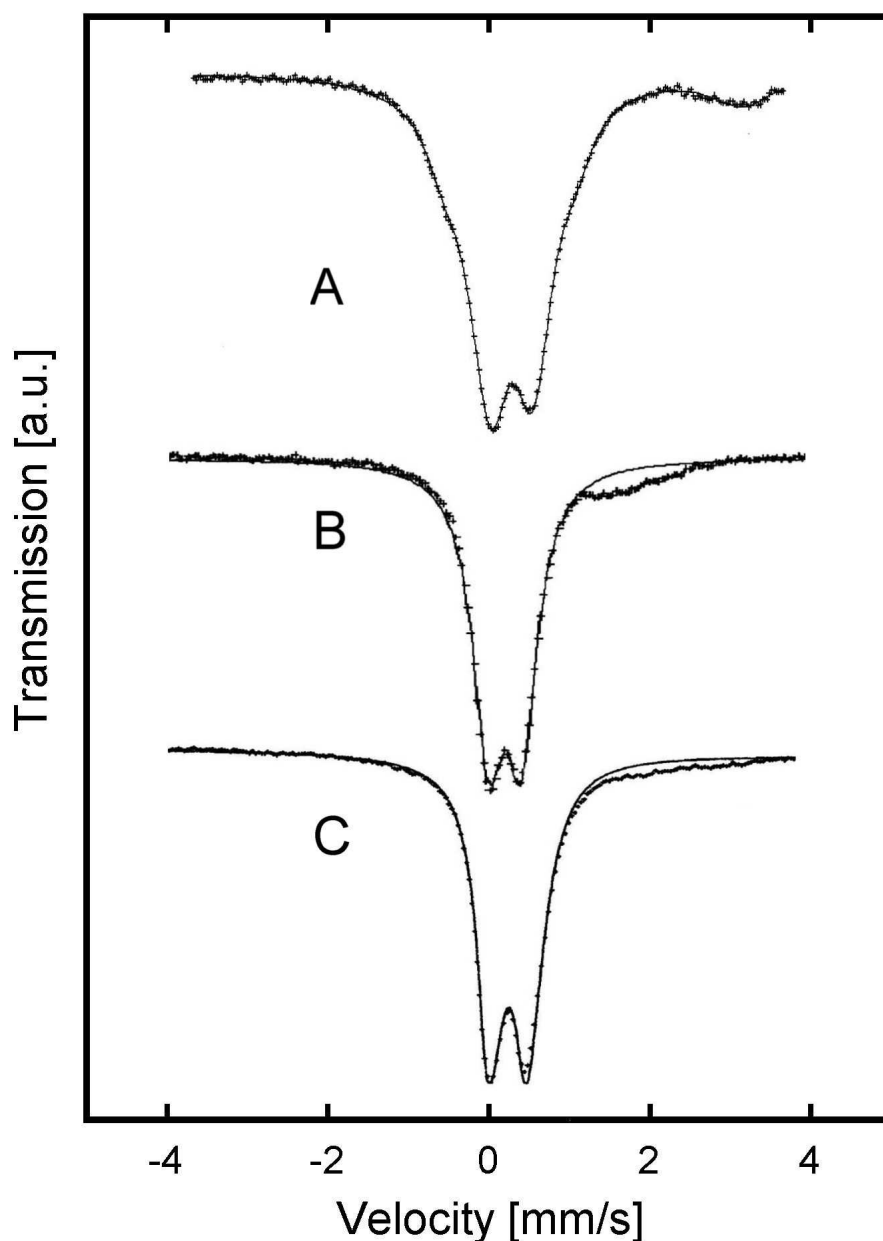
Fig. IV.3.1 Mössbauer spectra of: A) polyaniline base doped with \text{FeCl}_3 and dried under high-vacuum B) PANI/ \text{FeCl}_3 processed with triple excess of HFAA and pumped under high-vacuum for 8 hours C) PANI/ \text{FeCl}_3 processed with triple excess of HFAA and pumped under high-vacuum for 40 hours. Spectra registered at 4K.
