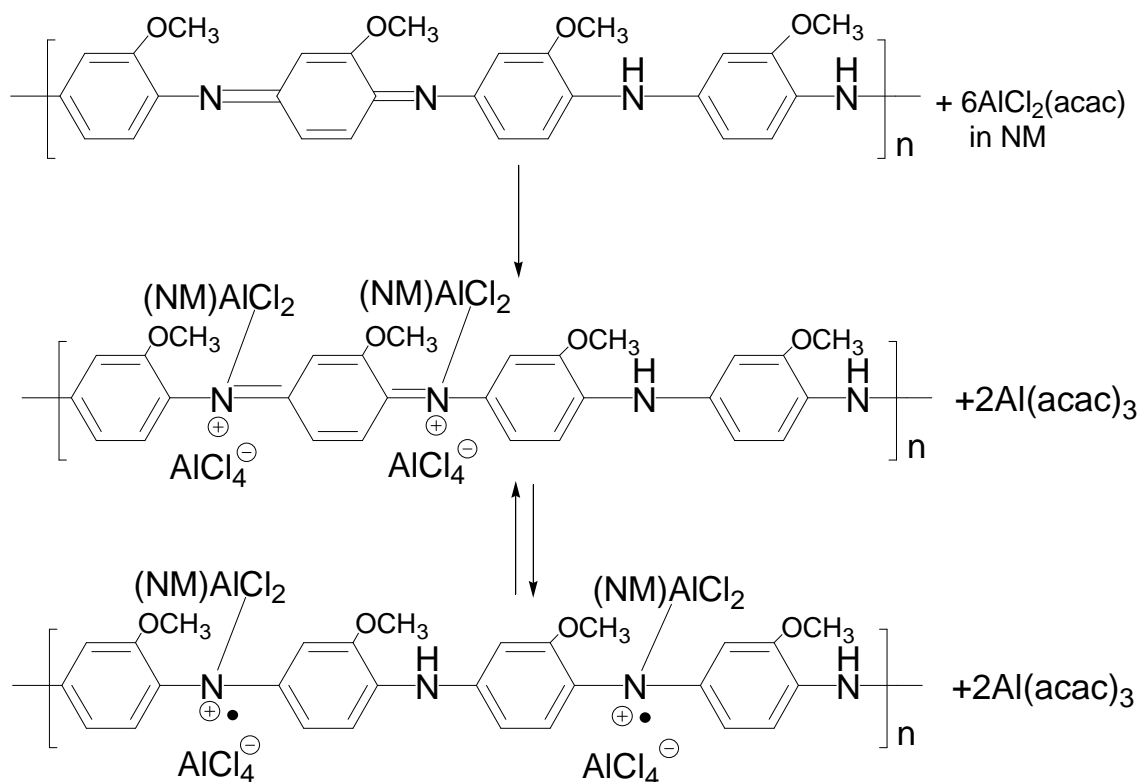
Fig. IV.6.4 Doping of polyanisidine with \text{AlCl}_2(\text{acac}) in nitromethane
