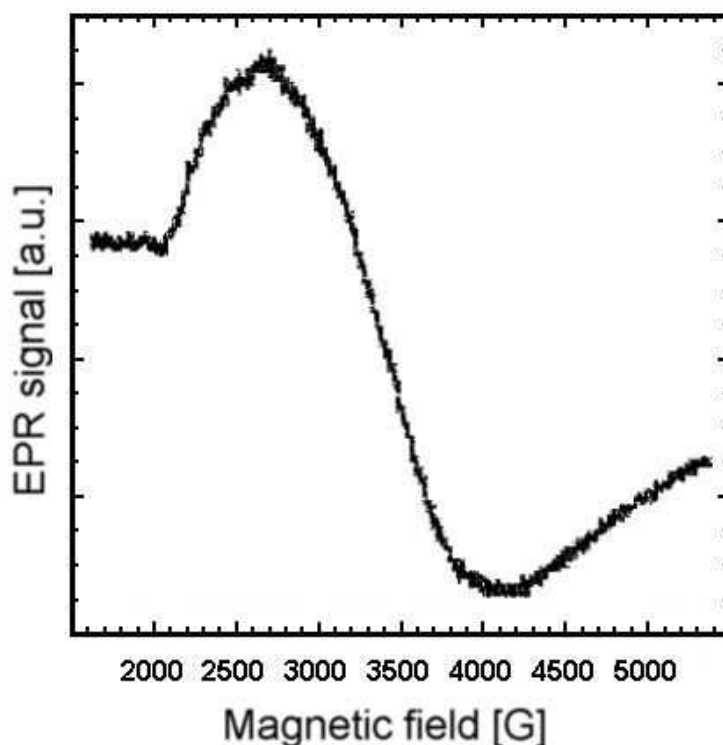
Fig.IV.3.6 EPR spectrum of polyaniline doped with \text{FeCl}_3 and additionally treated with HFAA
