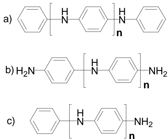
Fig. II.5.1 Three groups of aniline oligomers a) Ph/Ph end-capped, b) NH 2 /NH 2 end-capped, c) Ph/NH 2 end-capped
