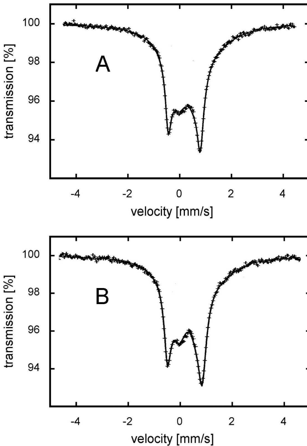
Fig. IV.4.3 Mössbauer spectra of polyanisidine doped with \text{FeCl}(\text{acac})_2 in nitromethane. A) spectrum of the freshly prepared sample; B) spectrum of the sample conditioned for 24 hours on air. Spectra were registered at 77K.
