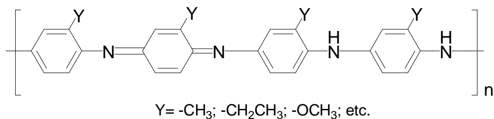
Fig. II.4.1 Ring substituted polyanilines in semi-oxidised form
