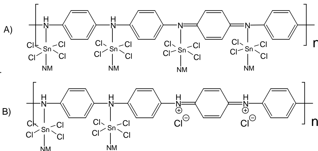
Fig.II.7.5 Emeraldine base (A), and emeraldine hydrochloride (B) doped with SnCl 4 in nitromethane (NM)
