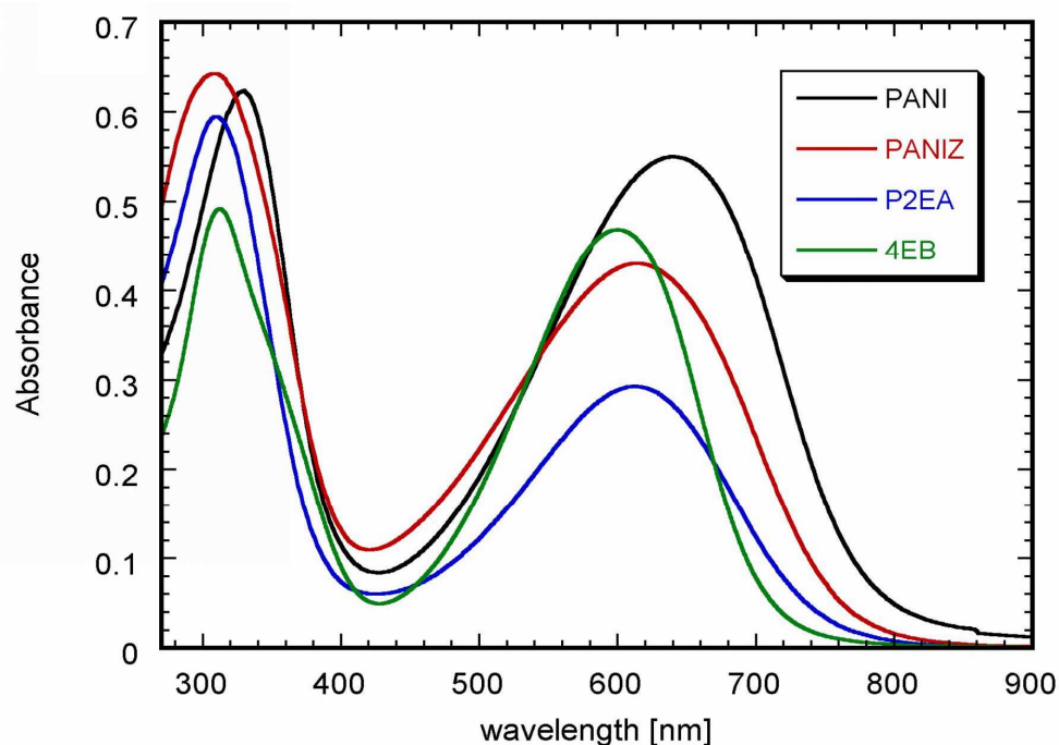
Fig. IV.1.4 The UV-Vis spectra of polyanilines and tetramer of aniline in NMP
