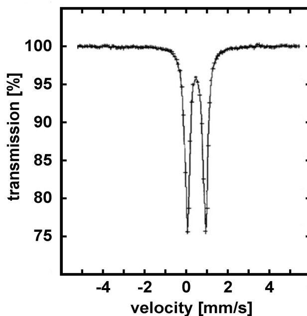
Fig. III.1.4 Mössbauer spectrum of chlorobis(acetylacetonato)iron(III) at 4K
