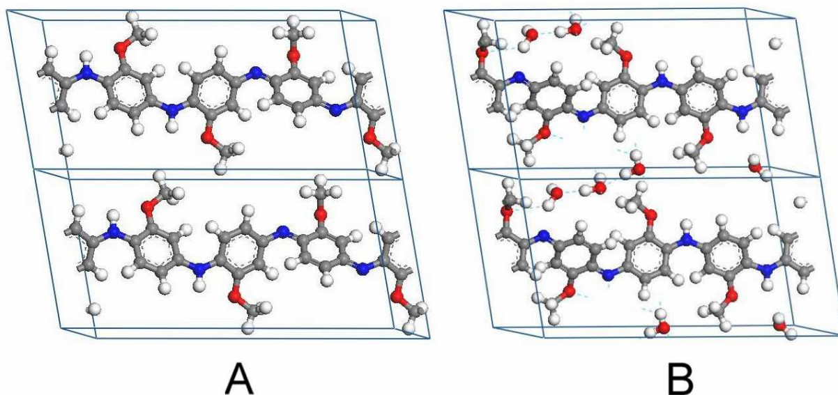
Fig. IV.1.2 Calculated structures of polyanisidine in a crystallite a) without H_2O b) containing H_2O molecules.
