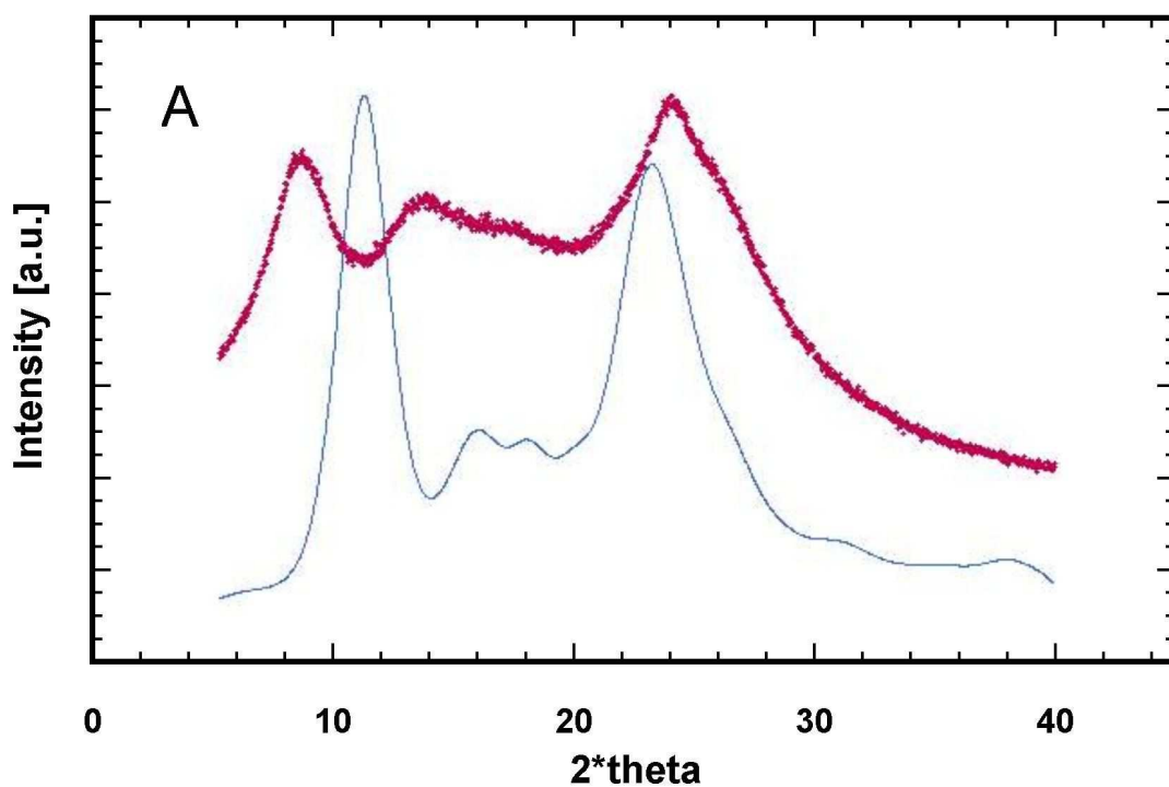
Fig. IV.1.3a Comparison of experimental pattern obtained for PANIZ (red line) and the theoretical results calculated for the model assuming no H_2O molecules (blue line)
