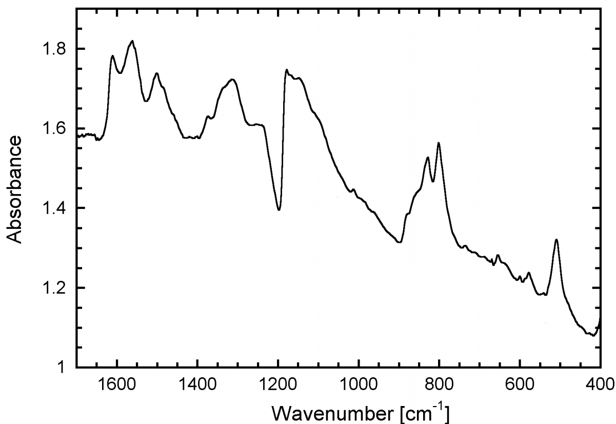
Fig. IV.2.3 IR spectrum ( 1700\text{ cm}^{-1} - 400\text{ cm}^{-1} ) of polyaniline doped with \text{FeCl}_3 ; mer to dopant ratio (1:1)
