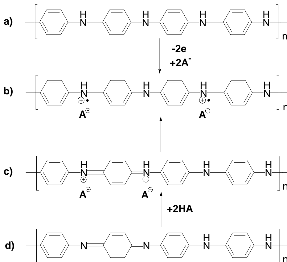
Fig.II.6.1 Principle of polyaniline doping
