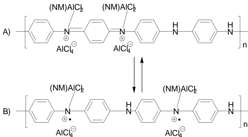
Fig.IV.5.4 Structure of emeraldine treated with aluminium chloride (III) in nitromethane
