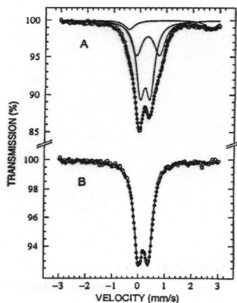
Fig.II.7.6 Mössbauer spectra registered at 77 K of a) emeraldine base doped with FeCl_3 (1:1) in nitromethane b) emeraldine hydrochloride doped with FeCl_3 (1:0,5) in nitromethane [14]
