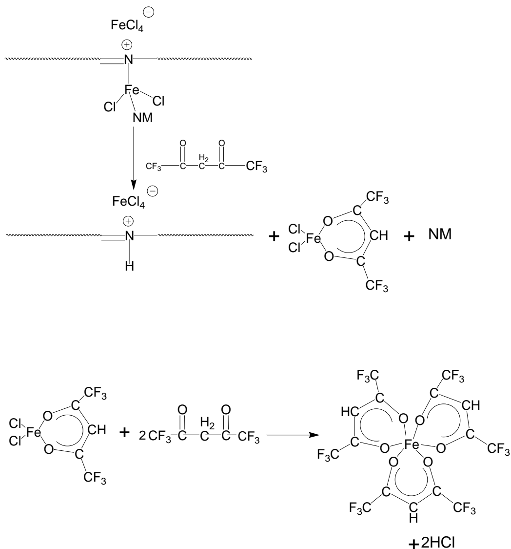
Fig. IV.3.2 Reactions occurring during treatment of PANI/FeCl 3 with triple excess of HFAA
