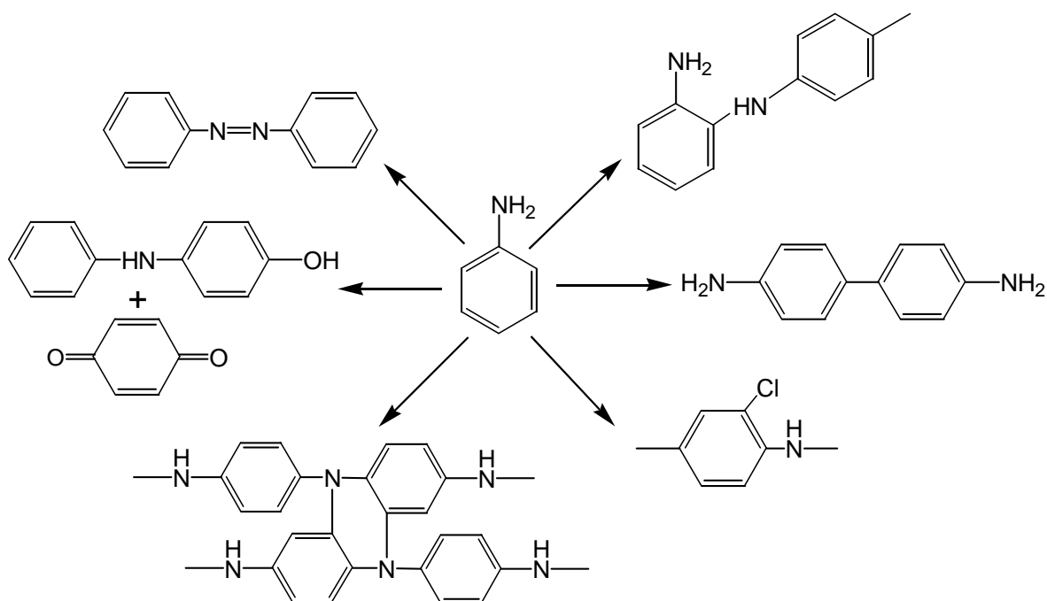
Fig. II.3.8 Side reactions occurring during polyaniline synthesis
