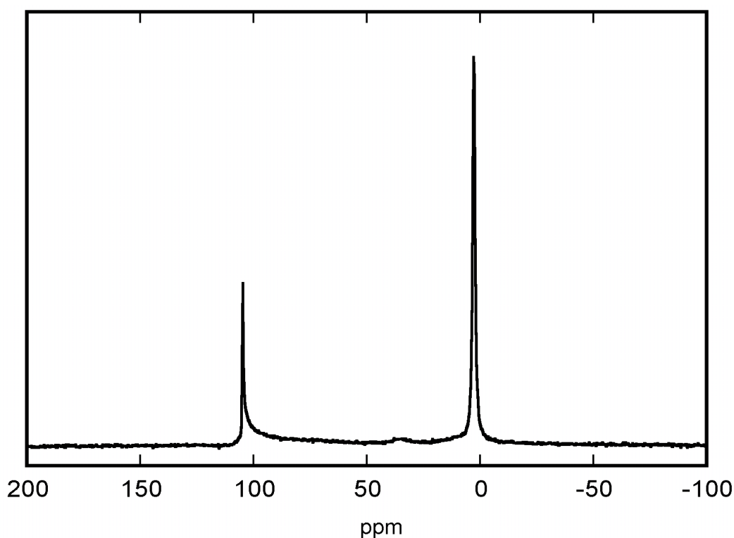
Fig. IV.6.2 ^{27}\text{Al} NMR spectrum of polyanisidine doped with \text{AlCl}_2(\text{acac}) in \text{CH}_3\text{NO}_2/\text{CD}_3\text{NO}_2 (4:1) registered at room temperature
