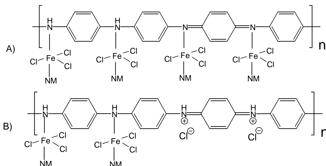
Fig. II.7.7 Emeraldine base (A), and emeraldine hydrochloride (B) doped with FeCl_3 in nitromethane (NM)
