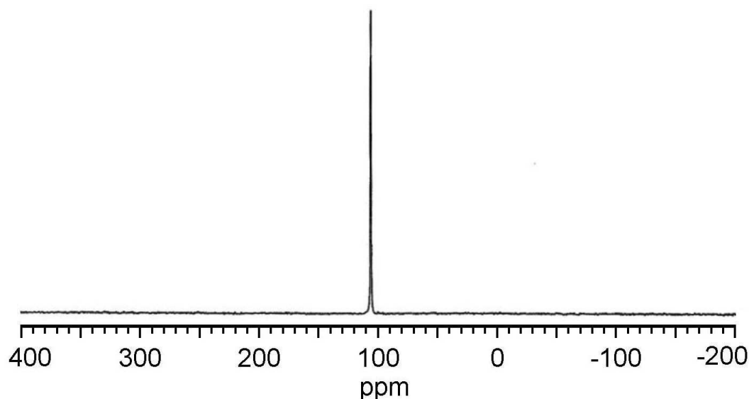
Fig. IV.5.2 ^{27}\text{Al} NMR spectrum of polyaniline- \text{AlCl}_3 mixture in \text{CD}_3\text{NO}_2/\text{CH}_3\text{NO}_2 (1:4) solution at room temperature; mer to dopant ratio (1:1,5)
