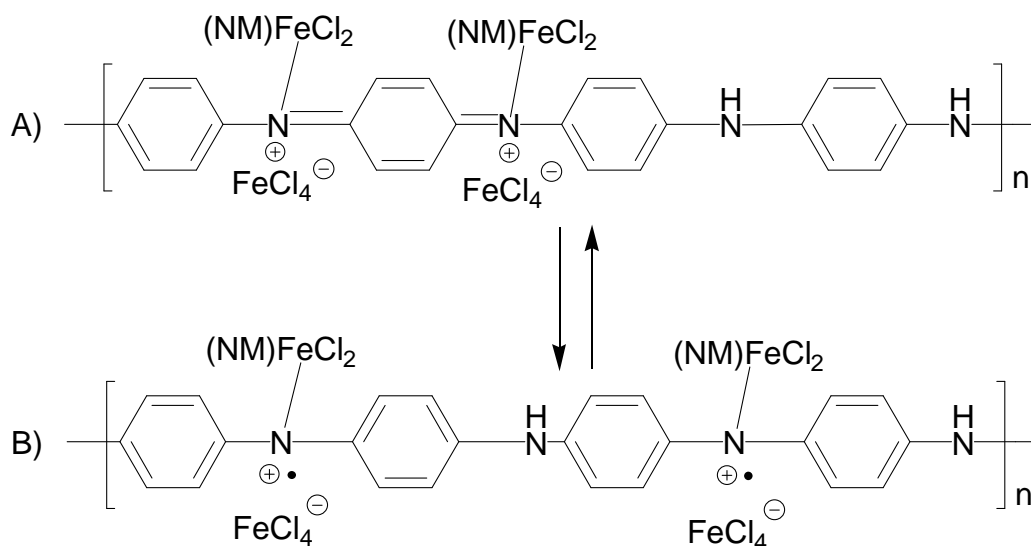
Fig. IV.2.4 Structure of emeraldine treated with iron chloride (III) in nitromethane
