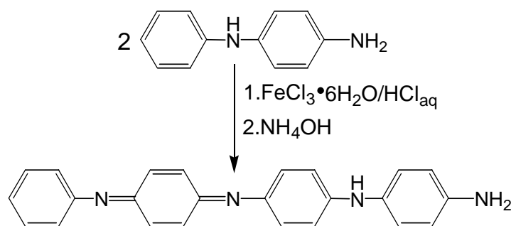
Fig. II.5.3 Oxidative synthesis of aniline Ph/NH 2 tetramer
