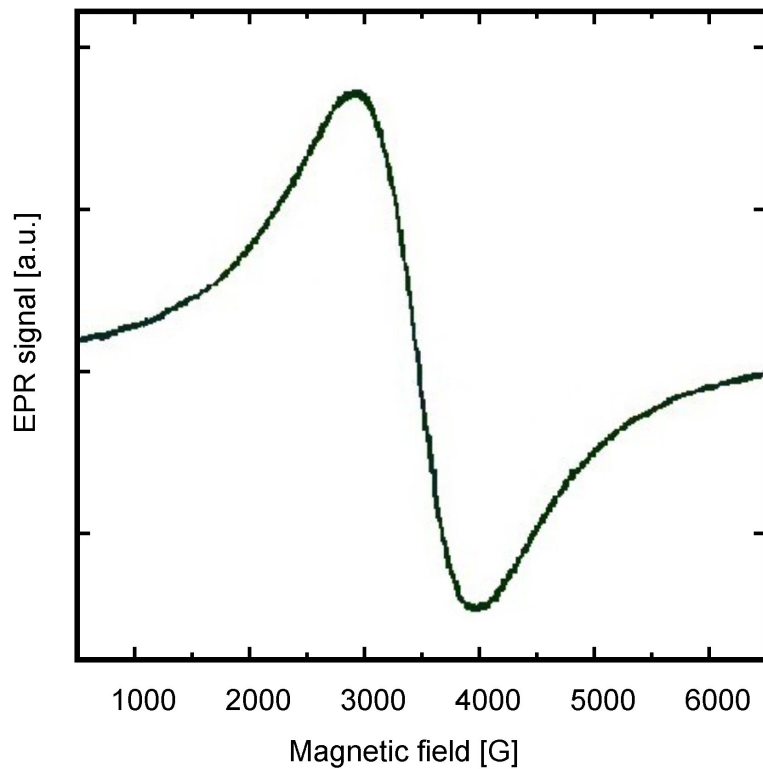
Fig. IV.5.5 EPR spectrum of emeraldine doped with \text{AlCl}_3
