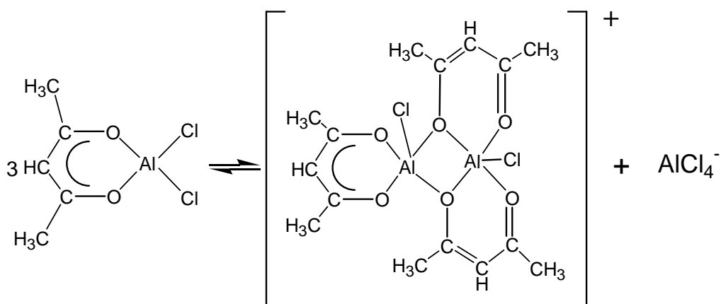
Fig.IV.6.3 Dissociation of monomeric \text{AlCl}_2(\text{acac})
