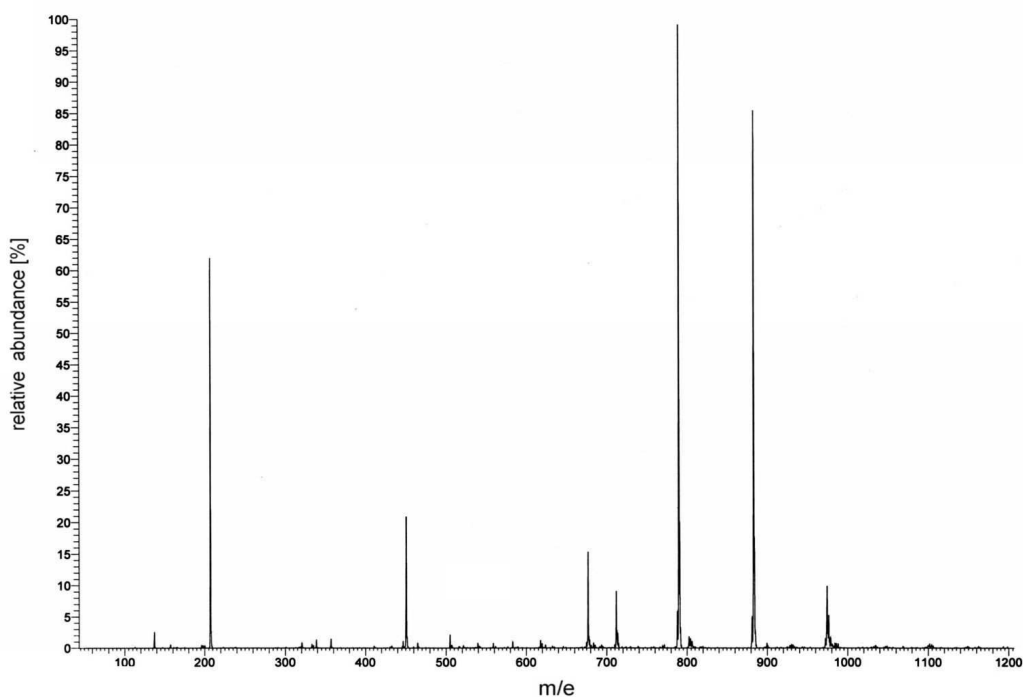
Fig. IV.3.3 Mass spectrum of the species condensed in liquid nitrogen trap during synthesis of PANI/ \text{FeCl}_3 /HFAA.
