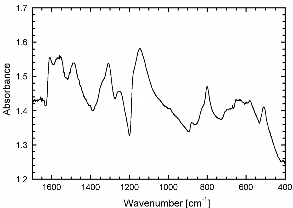
Fig. IV.5.6 IR spectrum ( 1700 \text{ cm}^{-1} - 400 \text{ cm}^{-1} ) of polyaniline doped with \text{AlCl}_3 ; mer to dopant ratio (1:1)
