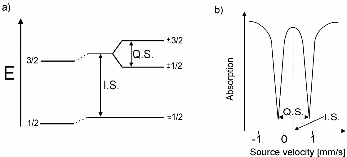
Fig..VI.3.1 a) Energy levels in sample (absorber), b) Corresponding Mössbauer spectrum
