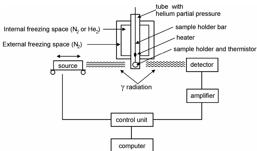
Fig.VI.4.1 Block scheme of Mössbauer spectrometer
