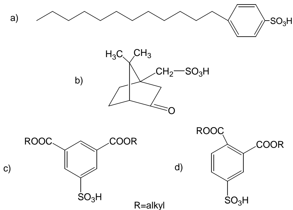
Fig. II.7.1 Selected sulfonic acids used for the acid-base doping of PANI
