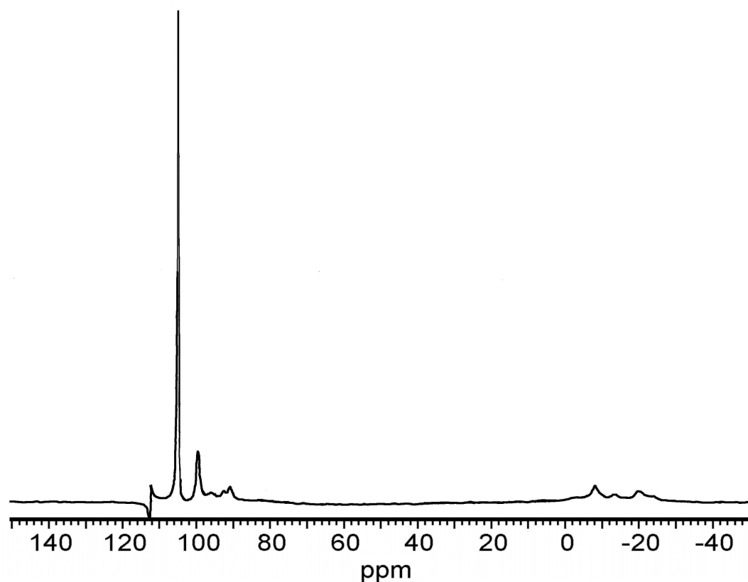
Fig. IV.5.1 ^{27}\text{Al} NMR spectrum of 5% \text{AlCl}_3 solution in \text{CD}_3\text{NO}_2/\text{CH}_3\text{NO}_2 (1:4), registered at room temperature
