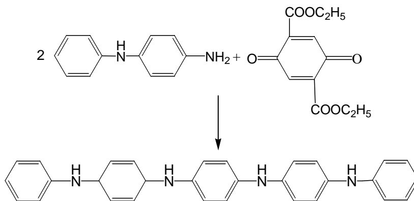
Fig. II.5.2 Honzl's synthesis of aniline tetramer
