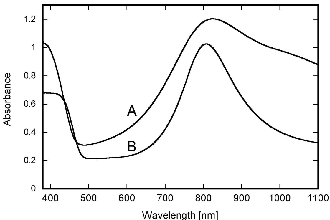
Fig. IV.6.1 UV-Vis-NIR spectra of poly(2-ethylaniline) (A) and polyanisidine (B) doped with dichloro(acetylacetonato) aluminium(III) in nitromethane
