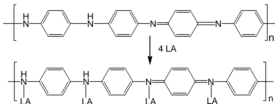
Fig.II.6.2 Lewis acid doping of emeraldine
