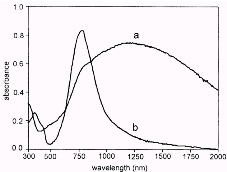
Fig.II.7.4 The UV-Vis-NIR spectra of PANI/(SnCl 4 ) 1,0 /(CH 3 NO 2 ) 1,0 cast from nitromethane: a) freshly prepared film, b) film exposed to the water vapours for 10 min.[13]
