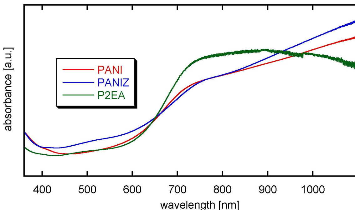
Fig. IV.5.3 UV-Vis-NIR spectra of the nitromethane solutions of polyaniline, polyanisidine and poly(2-ethylaniline) doped with \text{AlCl}_3 ; mer to dopant ratio (1:1)
