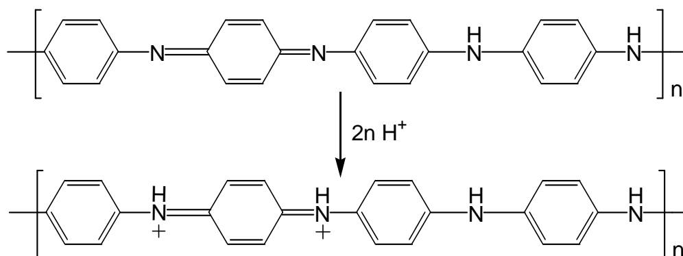
Fig.II.3.7 Protonation of the emeraldine
