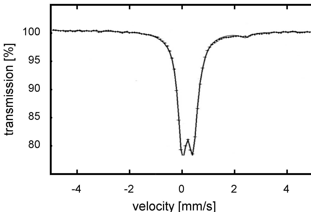
Fig. IV.3.4 Mössbauer spectrum of polyaniline hydrochloride doped with \text{FeCl}_3 (1:0,5) and subsequently treated with HFAA. Spectrum registered at 4K.
