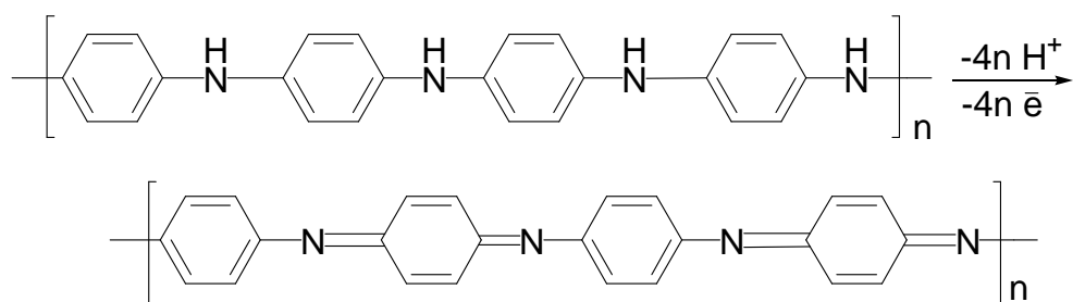
Fig. II.3.5 Oxidation of leucoemeraldine to pernigraniline
