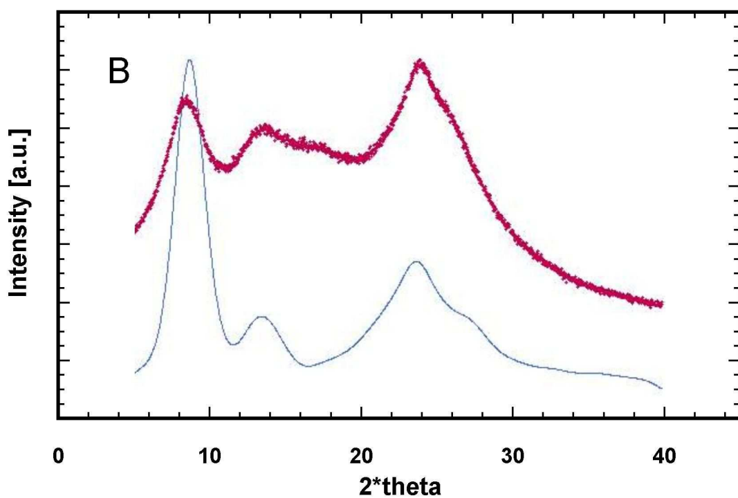
Fig. IV.1.3b Comparison of the experimental curve obtained for PANIZ (red line) and the theoretical results calculated for the model assuming one H_2O molecule per one nitrogen atom (blue line)
