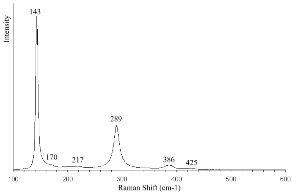
Figure VI-6: Spectre Raman de la Litharge de marque Laverdure. \lambda=514 \text{ nm} , P=5 \text{ mW} , T=5 \text{ sec.} , 4 acc., x50.
