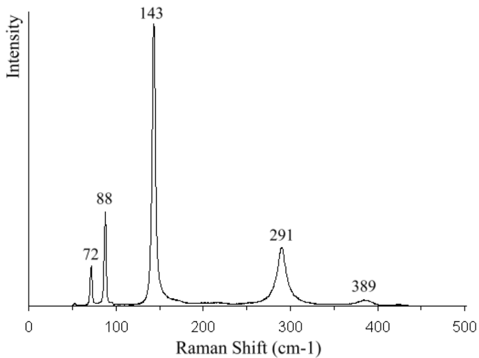
Figure VI-20: Spectre Raman de la plattn rite cuite   616 C pendant 10 heures (massicot pur). \lambda=514 nm P=5 mW, T=5 sec., 4 acc., x200.
