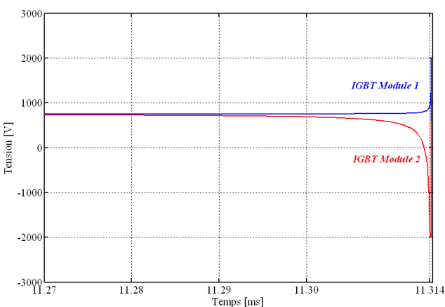
Figure 4-12 : Surtensions aux bornes des IGBTs 1 et 2 (cf. Figure 4-8)
