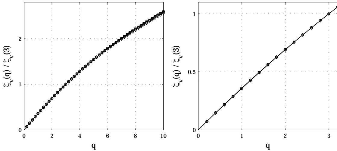
FIG. 13.2 – Exposants \widehat{\zeta}_v^d(q) = \widehat{\zeta}_v^d(q)/\widehat{\zeta}_v^d(3) : R_\lambda \simeq 380 ( \square ), R_\lambda \simeq 580 ( \times ), R_\lambda \simeq 2000 ( \diamond ) et R_\lambda \simeq 3200 ( \circ ).
