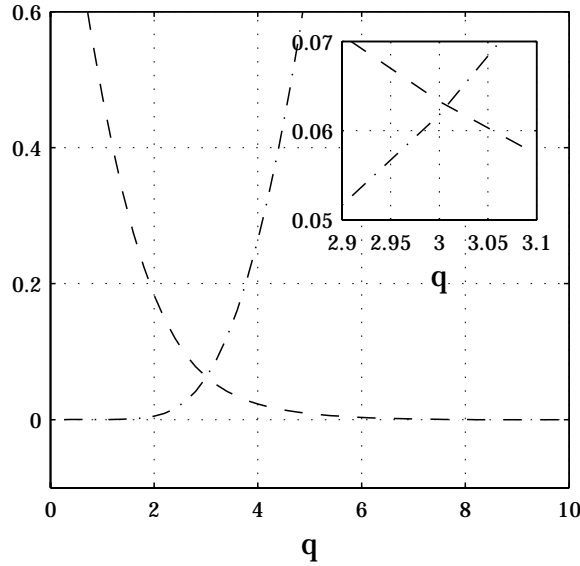
FIG. 9.5 – Cascades de Mandelbrot canoniques. \left| \widehat{\zeta}_{cmc_i}^a(q) - \varphi_{cmc}(q) \right| (trait point-tiret) et \left| \widehat{\zeta}_{cmc_i}^a(q) - \widehat{L}_{cmc_i}^a(q) \right| (trait tiret-tiret).
