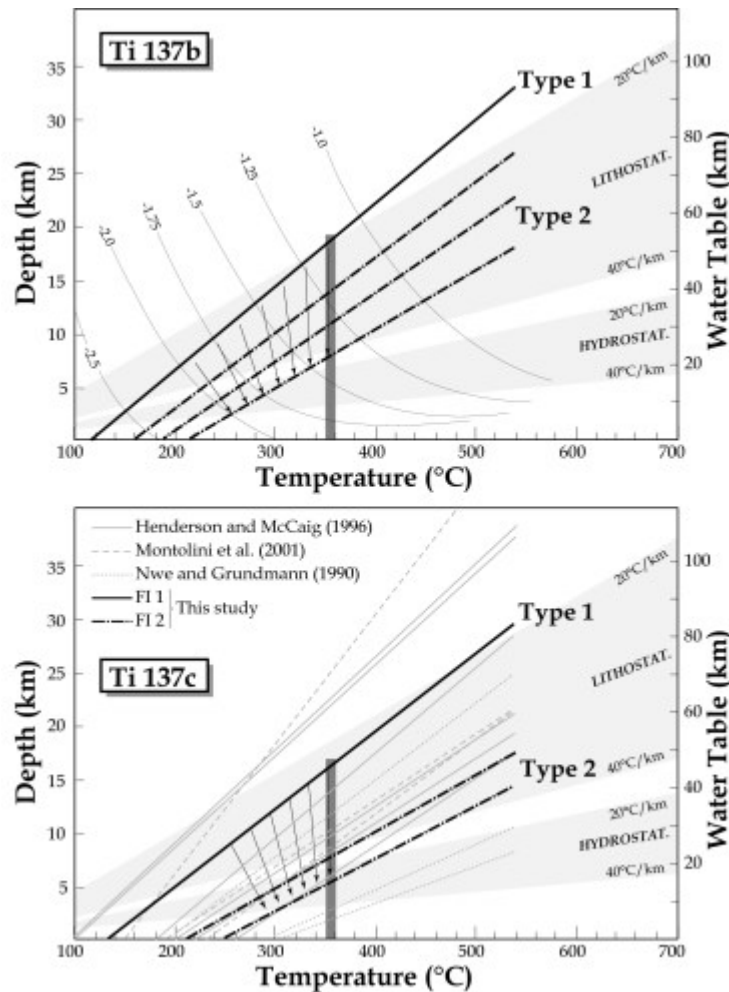
Figure 7: Calculated isochores for Type 1 and Type 2 fluid inclusions. Shaded areas represent the possible range of lithostatic and hydrostatic fluid pressure conditions (rock density = 2.7 g.cm -3 , fluid density = 1g/cm -3 ) based on a realistic range of geothermal gradients (20-40°C/km). Thick grey lines represent the maximum possible temperatures. Black arrows show the possible pressure-temperature paths from Type 1 to Type 2 fluid inclusions crossing silica solubility isopleths (See text for explanation). a) Ti 137b strain fringe. Silica solubility isopleths from Walther and Helgeson (2000). b) Ti 137c strain fringe. Literature microthermometric data from compressive ductile shear zones showing pressure fluctuations have been added for comparison (Nwe & Grundmann, 1990 ; Henderson & McCaig, 1996 ; Montolini et al., 2001).
