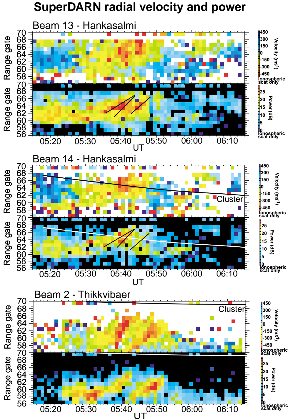
Fig. 6. Pairs of range-time plots (l-o-s velocity and backscattered power) for three beams of SuperDARN radars for the period 05:15–06:15 UT. The Cluster footprint is superimposed on beam 14 of Hankasalmi and beam 2 of Pikkvibær (black or white line). The slope of the range-time dispersed structures are depicted by black segments on the power plot of the beams 13 and 14 of the Hankasalmi radar.
