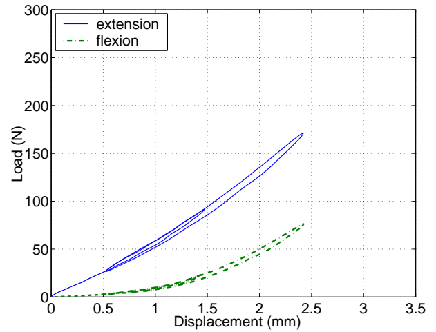
(b) The same LCL alone in flexion and extension, under 5-Hz triangular loading.
