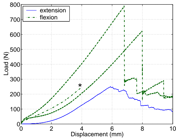
(a) PCL alone up to failure. * : since this sample broke at the level of the femur, the load versus displacement curve was not significant after this displacement.
