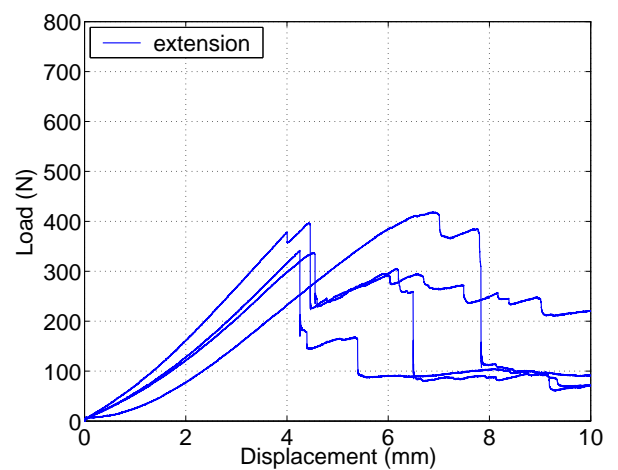
(b) LCL alone up to failure.
