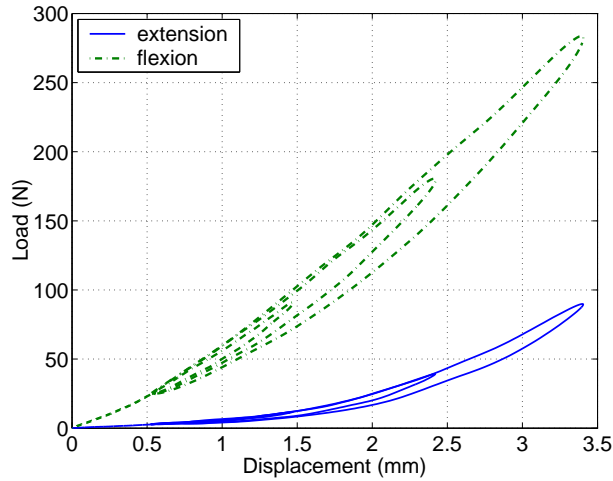
(a) The same PCL alone in flexion and extension, under 5-Hz triangular loading.
