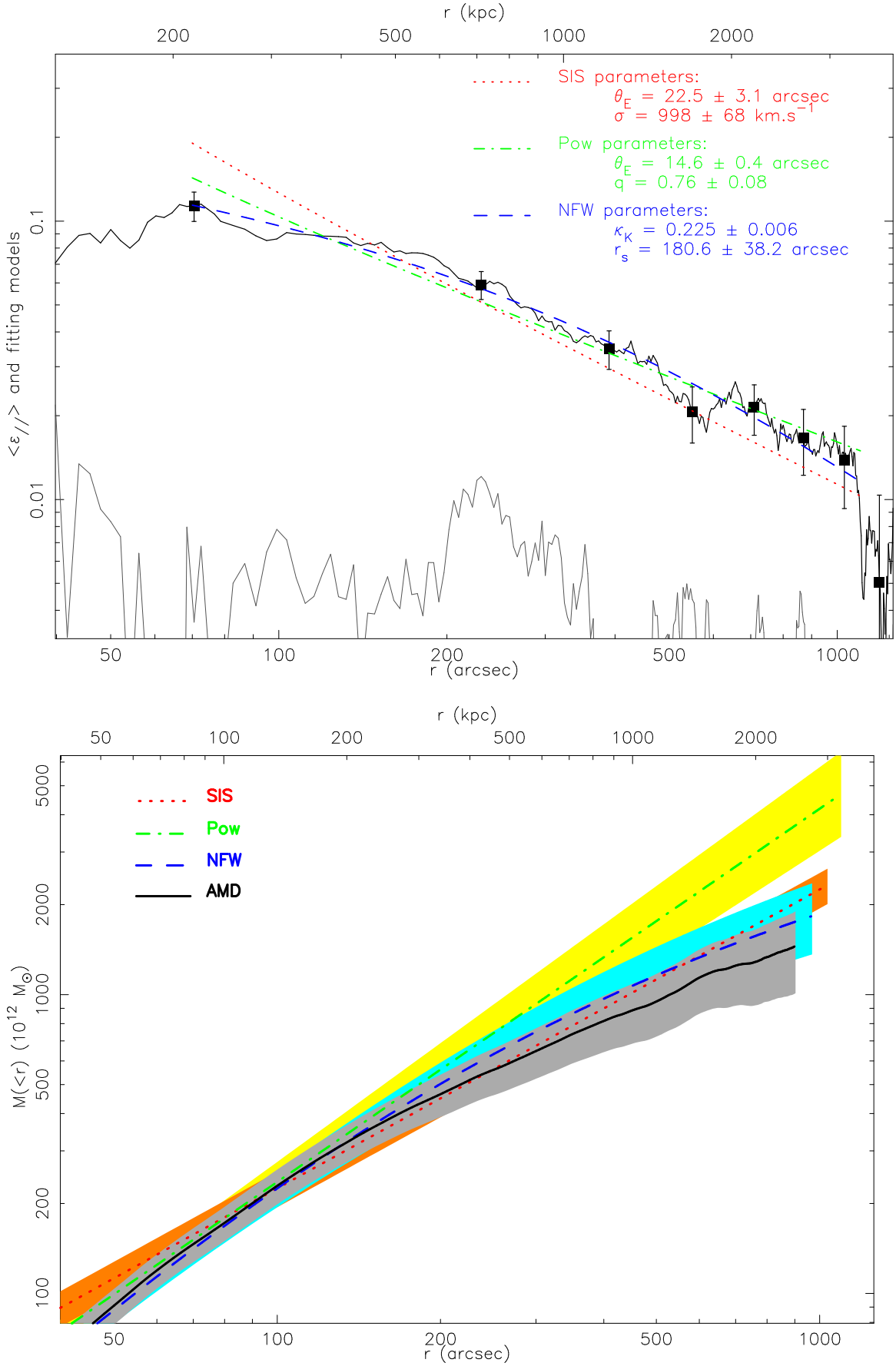
Fig. 12. Top: Best fitting parameters for SIS, Power law and NFW models, for Abell 1689 R-band shear profile. One series of uncorrelated points is shown (bin width = 158"). Bottom: Deduced mass profiles from these. The mass profile from the Aperture Mass Densitometry Method is also displayed, with a reference radius of 1100". See text for details.
