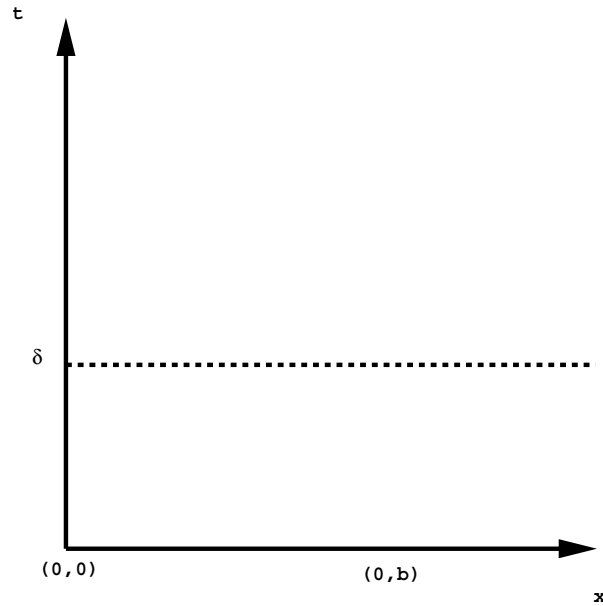
FIG. 3.1 – Space-time
