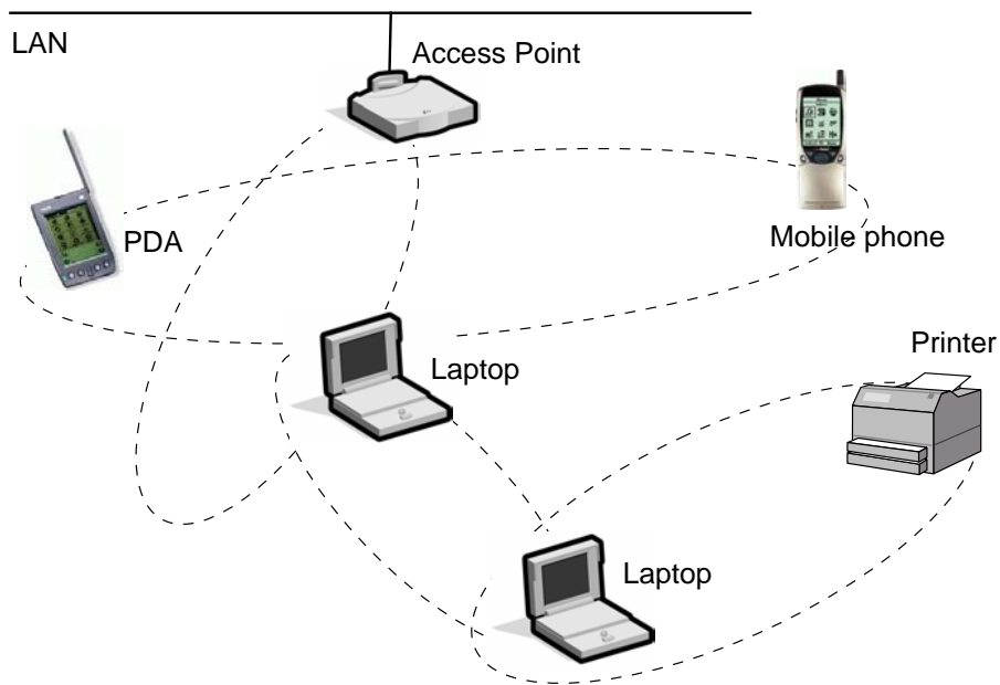
Figure 2.11: A Bluetooth scatternet of four piconets.
