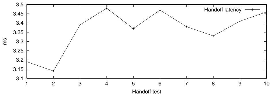
Figure 6.18: Handoff latency.
