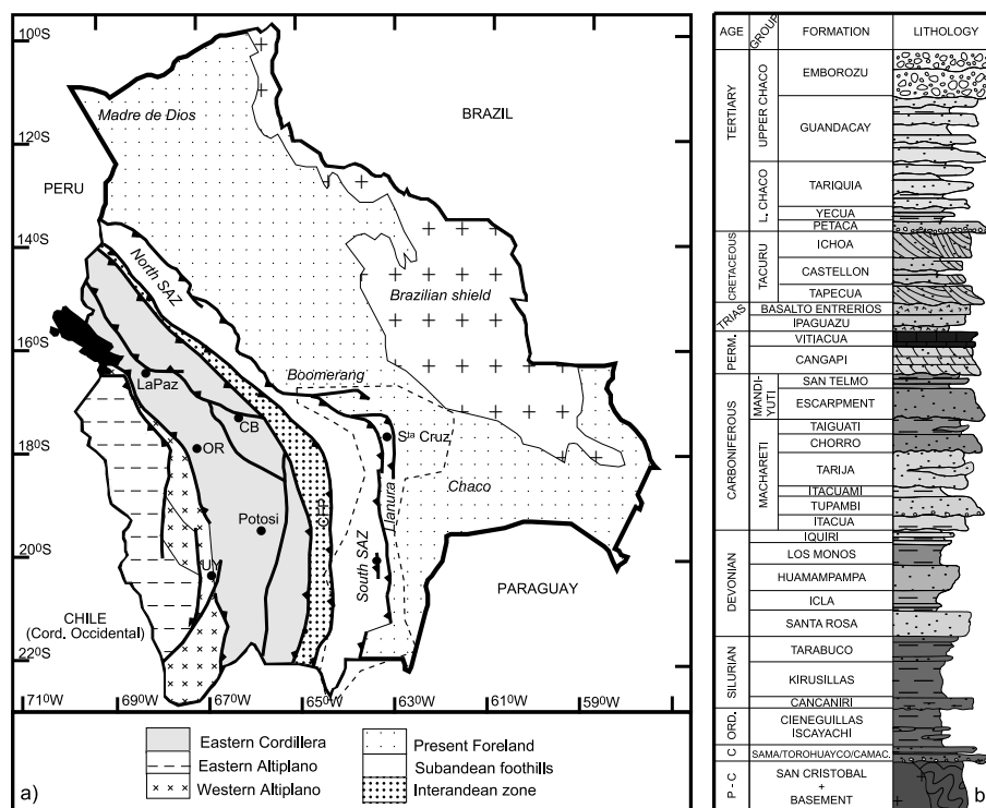
FIG. 2.3.9 – a) Structural map of the Bolivian Andes (modified from Baby et al., 1995a). b) Stratigraphic column of the southern Sub Andean Zone (from Moretti et al., 1996)
