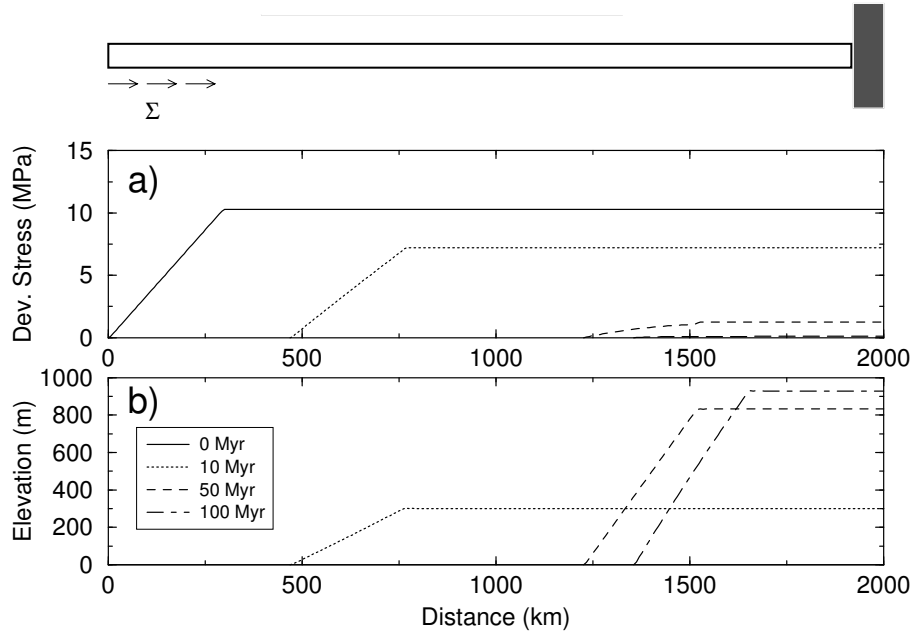
FIG. 2.2.1 – Deviatoric stress (a) and elevation (b) induced by a uniform basal friction \Sigma = 3.5 MPa, toward the hinterland, over the length \Delta_{\Sigma} = 300 km. Four time steps have been chosen. The simulations are performed with L = 100 km, \eta = 10^{22} Pa s, \rho_c = 2800 kg m ^{-3} and \rho_m = 3200 kg m ^{-3} . The initial crustal thickness is S_0 = 35 km and the plate length D = 7000 km. With these values, the plate boundary moves rightward with an initial velocity of 5.6 cm yr ^{-1} . The topography (b) evolves until a final elevation of about 1000 m while the deviatoric stress (a) tends to zero.
