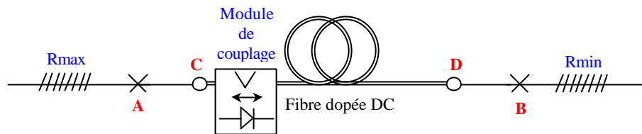
Figure III-1 : Structure (configuration co-propagative).
